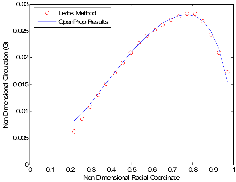
Figure 4: Non-Dimensional Circulation Comparison
