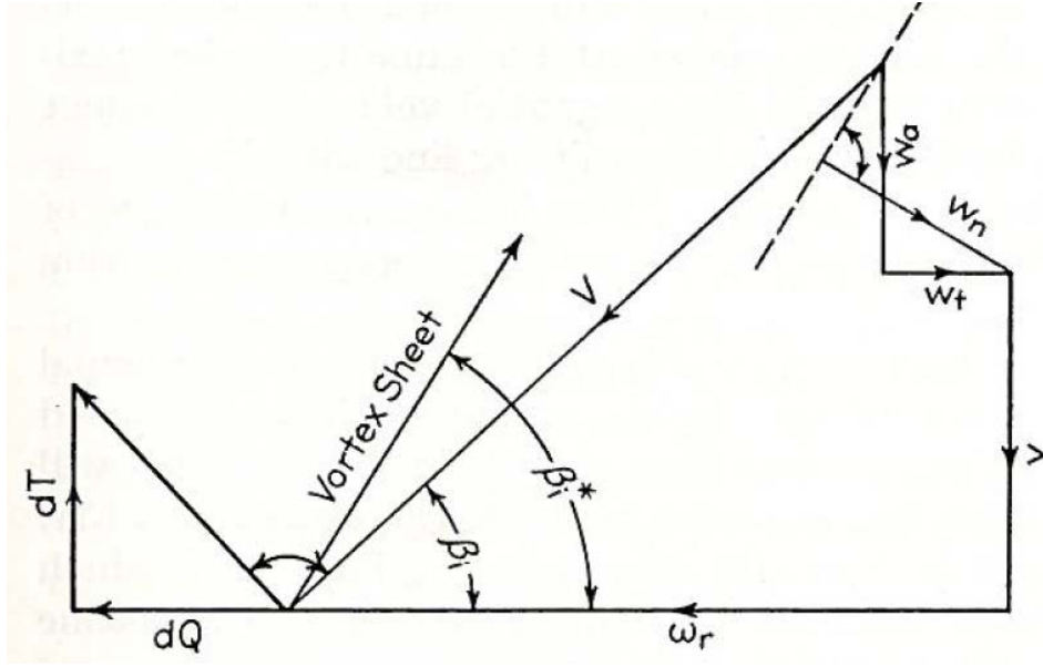
Figure 2: Pitch Angle Relationships to Velocities and Forces (4)
