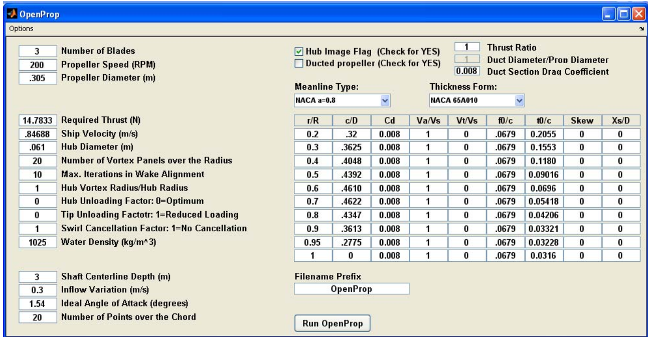
Figure 8: OpenProp Input Parameters for the DTMB 4119 Propeller
