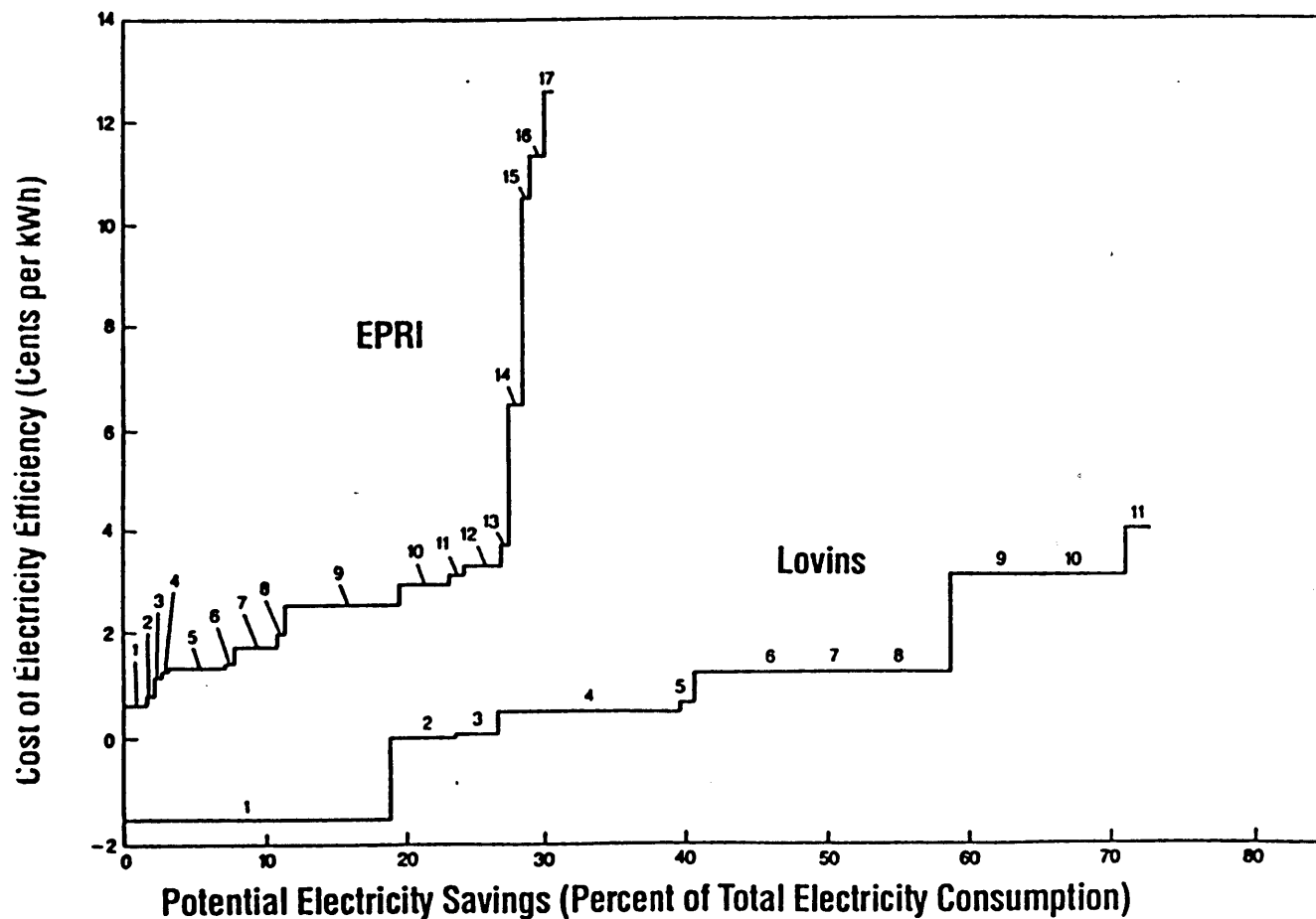
Figure 1: Potential Electricity Savings
