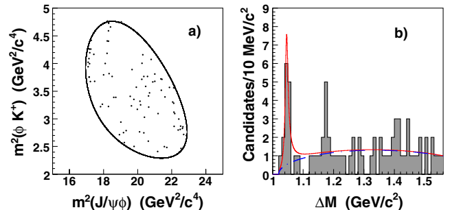
FIG. 2 (color online). (a) The Dalitz plot of m^2(\phi K^+) versus m^2(J/\psi \phi) in the B^+ mass window. The boundary shows the kinematically allowed region. (b) The mass difference, \Delta M , between \mu^+ \mu^- K^+ K^- and \mu^+ \mu^- , in the B^+ mass window. The dash-dotted curve is the background contribution and the red solid curve is the total unbinned fit.
