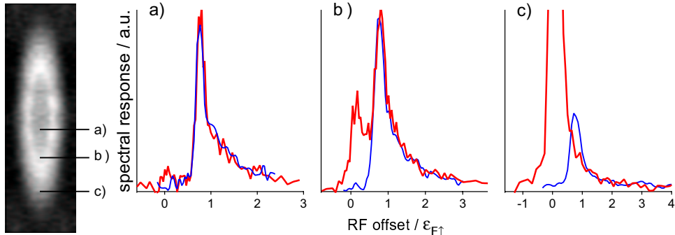
Figure 4. Tomographic RF spectroscopy of strongly interacting Fermi mixtures. A trapped, inhomogeneous sample has various phases in spatially different regions. The spectra of each region (red: majority, blue: minority) reveals the nature of pairing correlation of the corresponding phase. (a) Balanced superfluid. (b) Polarized superfluid. The additional peak in the majority spectrum is the contribution of the excess fermions, which can be identified as fermionic quasiparticles in a superfluid. From the separation of the two peaks, the pairing gap energy of a resonantly interacting superfluid has been determined [43]. (c) Highly polarized normal gas. The minority peak no longer overlaps with the majority spectrum, indicating the transition to polaronic correlations.
