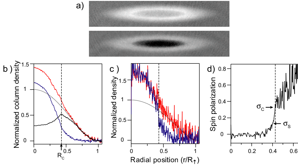
Figure 2. Spatial structure of a trapped Fermi mixture with population imbalance. (a) The in situ column density distributions are obtained using a phase contrast imaging technique [39]. The probe frequencies of the imaging beam are different for two images so that the first image measures the density difference n_{\uparrow} - n_{\downarrow} and the second image measures the weighted density difference 0.76n_{\uparrow} - 1.43n_{\downarrow} . (b) The smooth column density profiles are obtained from the elliptical averaging of the images under the local density approximation (red: majority, blue: minority, black: difference). (c) The reconstructed three-dimensional density profiles. (d) The spin polarization profile shows a sharp increase, indicating the phase separation between a core superfluid and a outer normal region. The vertical dashed line marks the location of the phase boundary.
