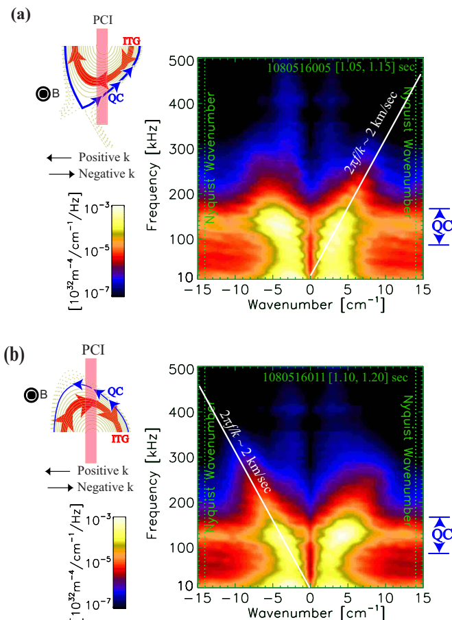
FIG. 7. (Color online) Frequency/wavenumber spectra of plasma fluctuations measured by PCI in the ITB plasma with only off-axis ICRF heating. On the left corner of each plot, the diagnostic line-of-sight is shown according to the masking phase plate setup: (a) The bottom plasma view, (b) the top plasma view.
