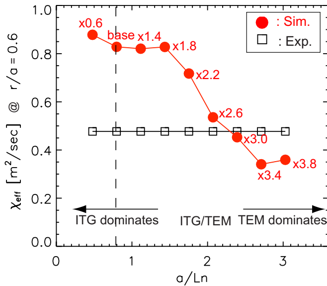
FIG. 10. (Color online) Impact of varying a correction factor applied to the measured density gradient on turbulent transport in the ITB plasma with only off-axis ICRF heating, where a/L_n = -(a/n)(dn/dr) .
