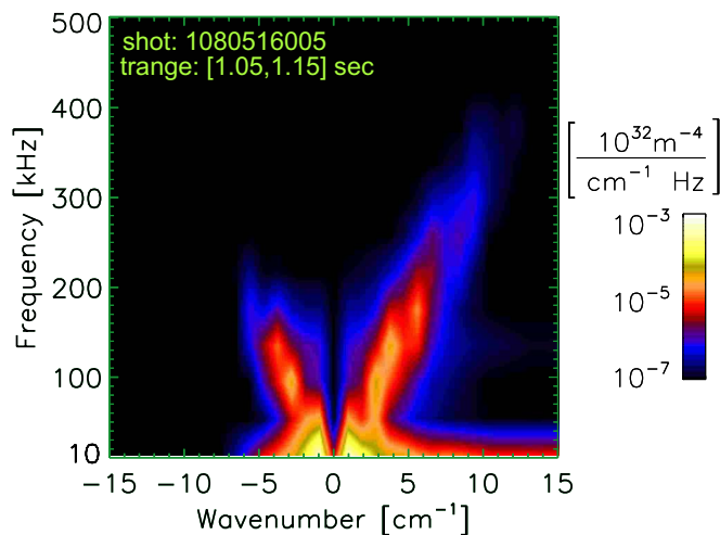
FIG. 12. (Color online) Synthetic PCI frequency/wavenumber spectra in the ITB with only off-axis ICRF heating. In the analysis, appropriate system response functions have been implemented to emulate the top view configuration of the masked phase plate.
