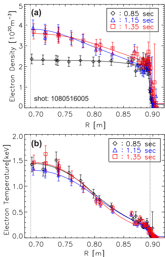
FIG. 2. (Color online) Profiles of electron density (a) and temperature (b) from the Thomson scattering (TS) diagnostic (Ref. 18) are shown before the ITB onset (black diamond), during the ITB with only off-axis ICRF heating (blue triangle), and during the ITB after adding on-axis ICRF heating (red square). The solid line is a fit to the experimental measurements using FiTs. Two vertical dashed lines are the magnetic axis and last closed flux surface (LCFS), respectively.
