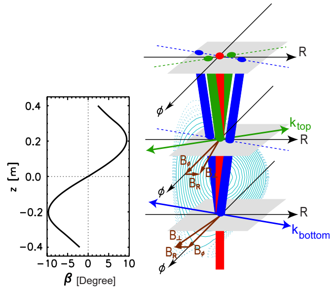
FIG. 4. (Color online) Left: Magnetic pitch angle \beta vs vertical coordinate z . Right: Principle of vertical localization. The vertical beam (red online) passing through the whole plasma corresponds to the unscattered beam, while the beams originated from the bottom (blue online) and the top (green online) correspond to the scattered beams from the turbulence localized at z = -0.2 m and z = +0.2 m, respectively.
