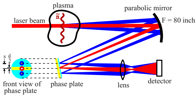
FIG. 3. (Color online) Principle of phase contrast imaging.
