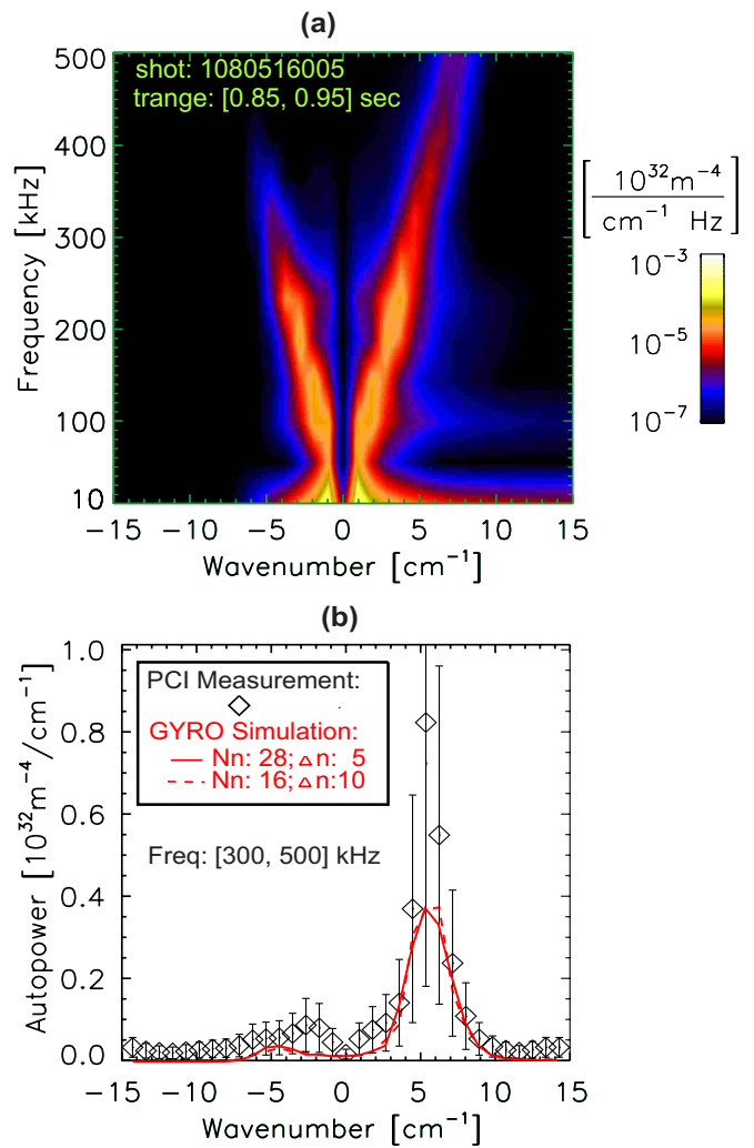
FIG. 11. (Color online) (a) Synthetic PCI frequency/wavenumber spectra in the H-mode plasma before the ITB formation. A system response function has been implemented to emulate the top view configuration of the masked phase plate. (b) Comparison of the synthetic and experimental PCI wavenumber spectra integrated in the frequency range of 300–500 kHz.
