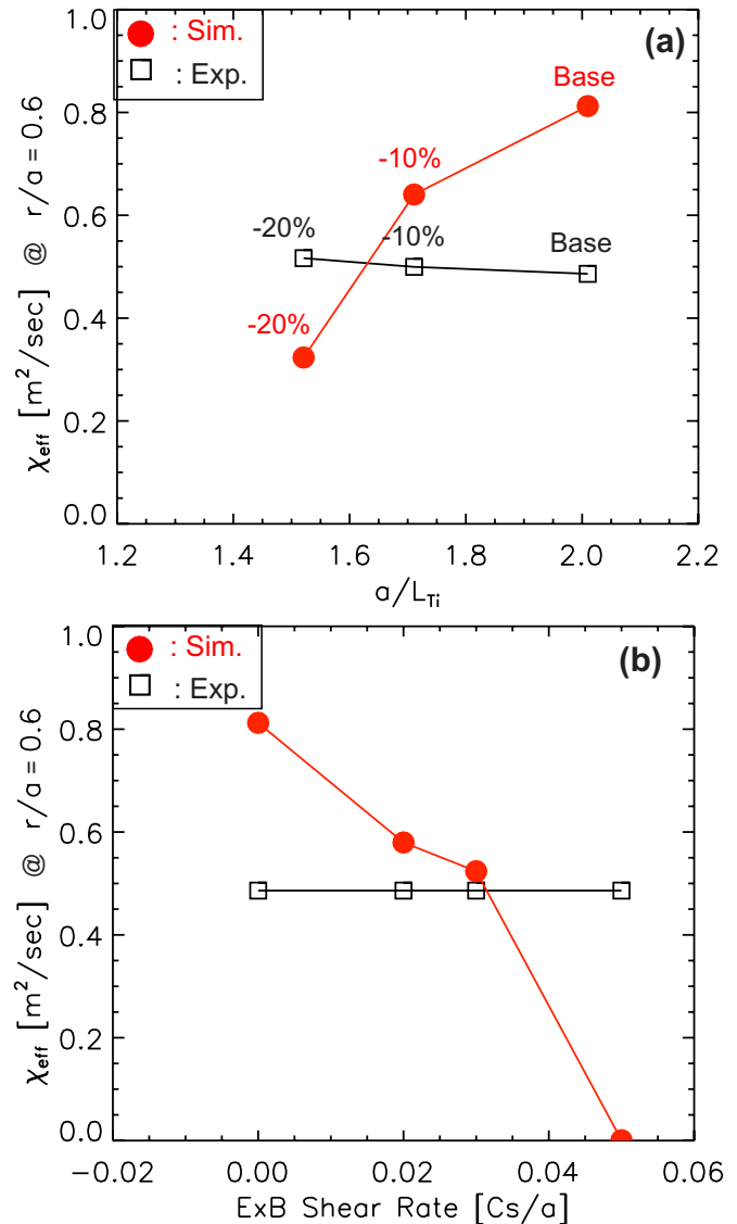
FIG. 9. (Color online) (a) Impact of varying a correction factor applied to the measured ion temperature gradient in the ITB plasma with only off-axis ICRF heating, where a/L_{Ti} = -(a/T_i)(dT_i/dr) . (b) Effect of the E \times B shear on turbulent transport in the ITB plasma with only off-axis ICRF heating, where c_s/a = 9 \times 10^5 Hz.
