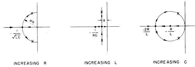
Fig. VIII-4. Loci for poles of single-tuned circuit.
