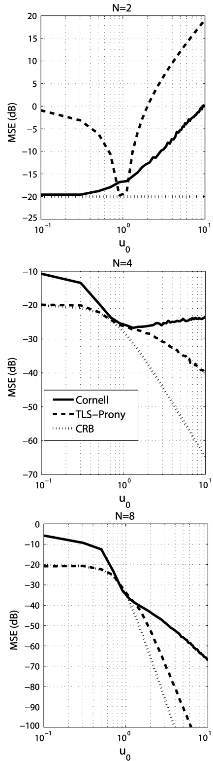
Fig. 3. Comparison between CRB and performance of the Cornell and TLS algorithms in estimating a real-valued powersum with one component in the presence of powersum AWGN. The SNR is 20 dB.
