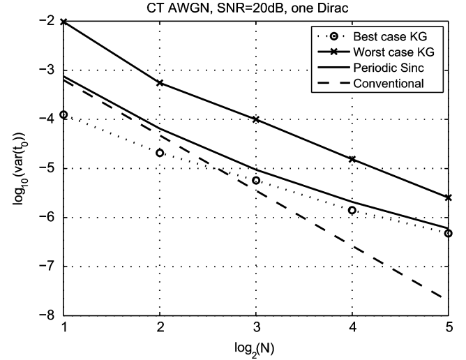
Fig. 8. Performance comparison for single-Dirac estimation, located within [0, T) , for the same numbers of samples. KG refers to the architecture proposed by the authors.
