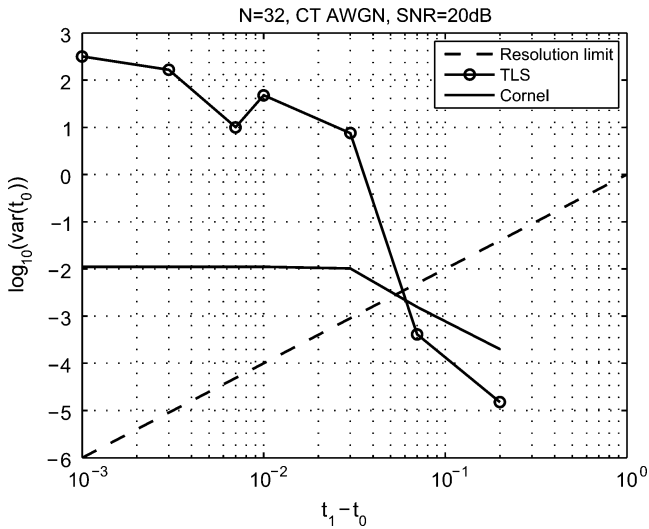
Fig. 7. Performance results for estimation of two Diracs using a first-order B-spline. The reconstruction first forms a length-4 powersum series. The AWGN is added in the continuous-time domain, with spectral density N_0 = 0.1 .
