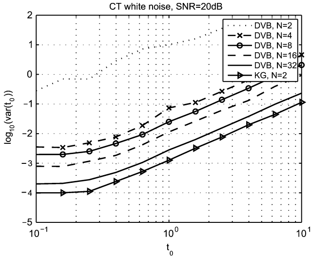
Fig. 6. Performance results for estimation of one Dirac using a first-order B-spline. The system is implemented using the simple Cornell algorithm. The plot shows different number of samples N , but the reconstruction first forms a length-2 powersum series. The AWGN is added in the continuous-time domain, with spectral density N_0 = 0.1 . DVB refers to the Dragotti-Vetterli-Blu architecture and KG refers to the architecture proposed by the authors.
