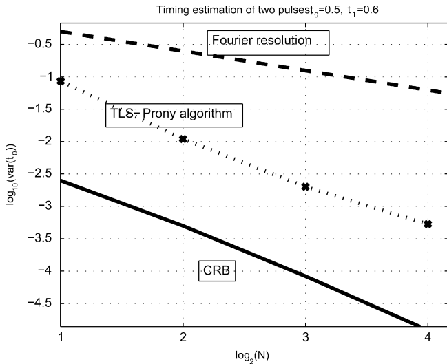
Fig. 2. Timing estimation result for the case of two signal components using the FRI in-time sampling system. The SNR is 20 dB, and we compare the Fourier resolution, the CRB, and the performance of the TLS-Prony algorithm.
