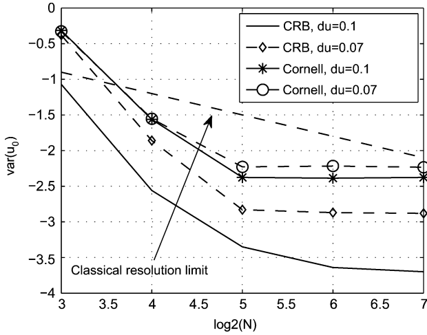
Fig. 4. Comparison between CRB of the proposed system and the Cornell algorithm in the presence of AWGN, in terms of number of samples. In this case the poles are near unity, u_0 = 0.8 , and we consider \delta u = u_1 - u_0 = 0.1, 0.07 . The simulation is done at SNR = 20 dB. As the performance of the TLS algorithm is very poor, we omit this from presentation.
