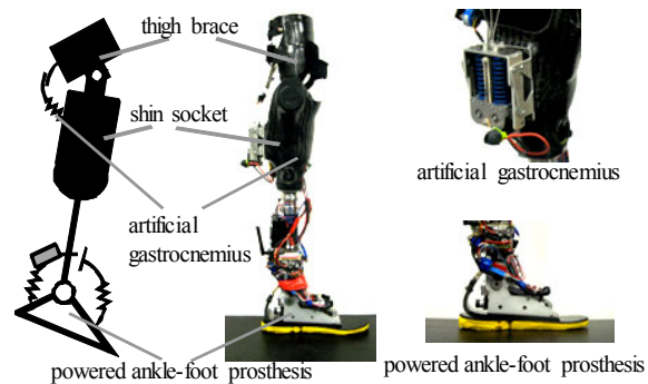
Fig. 4 Transtibial prosthesis with the PAP and the AG.
