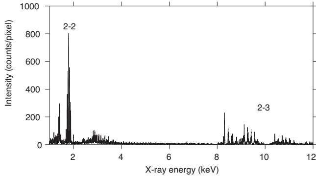
FIG. 1. Spectrum of tungsten from SuperEBIT recorded with the EBIT calorimeter spectrometer (ECS). Transitions between levels of principal quantum number n are labeled.
