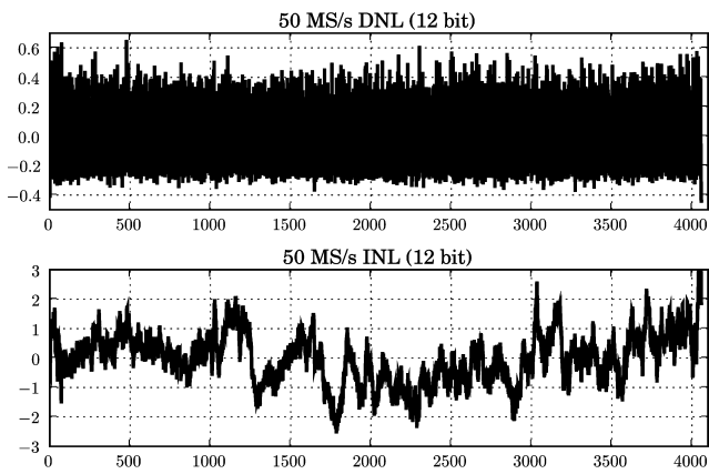
Fig. 27. Measured linearity.
