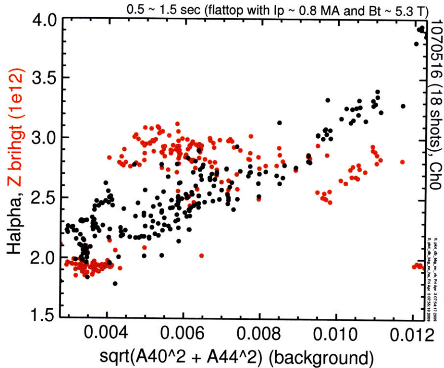
Figure 2-13: Total MSE background signals from Channel 0 (edgemoat channel; R = 85.7 cm) versus (a) Z brightness and (b) H_\alpha during the flattop phases.
