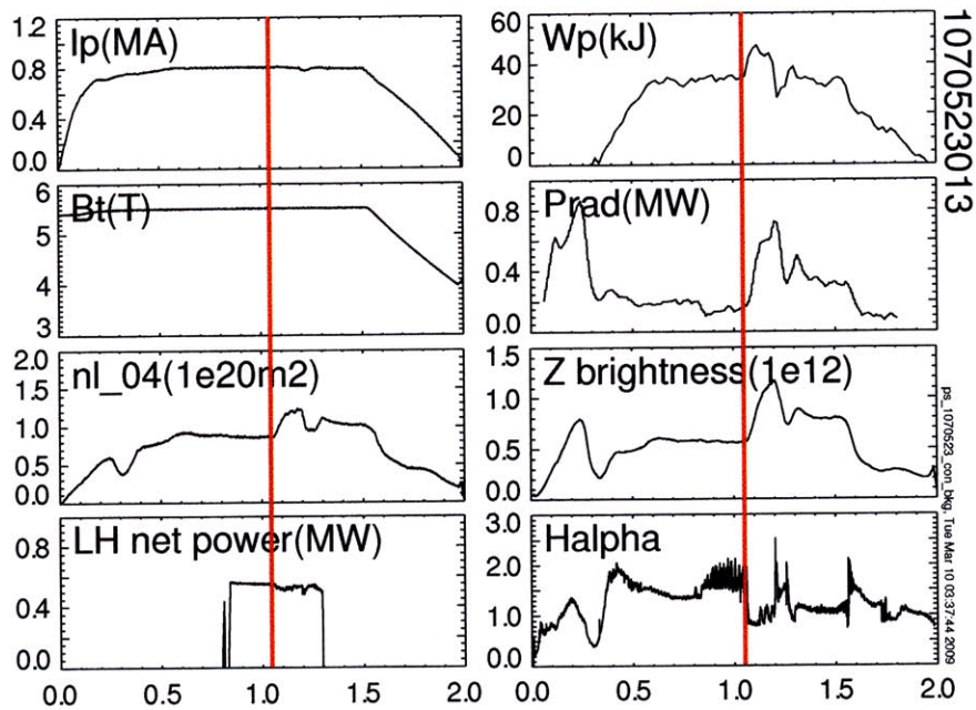
Figure 2-14: The waveforms of some plasma parameters from Shot 1070523013 for the MSE background study. The H-mode is induced by LH heating only (no ICRF). L-H transition is marked with a vertical red line.
