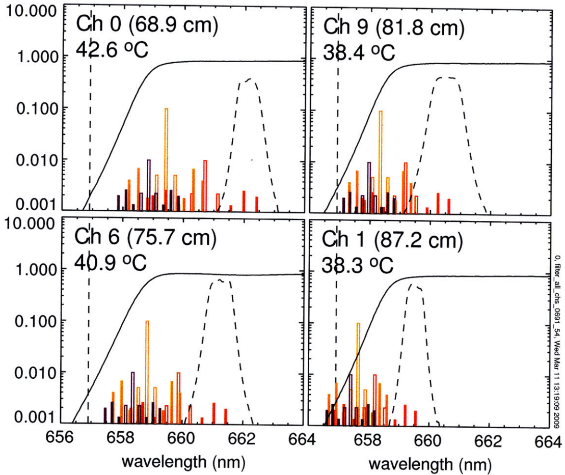
Figure 2-17: Edge (solid) and bandpass (dashed) filter functions in several MSE channels for B_T = 5.4 T along with the expected Stark lines ( \sigma in unfilled bar and \pi in filled bar) from Doppler-shifted full (red), half (orange), and a third (blue) beam energy components. The vertical line is at 656.9 nm where the blocking OD should be greater than 2 according to the spec. The oven temperature of the filter assembly is also given.
