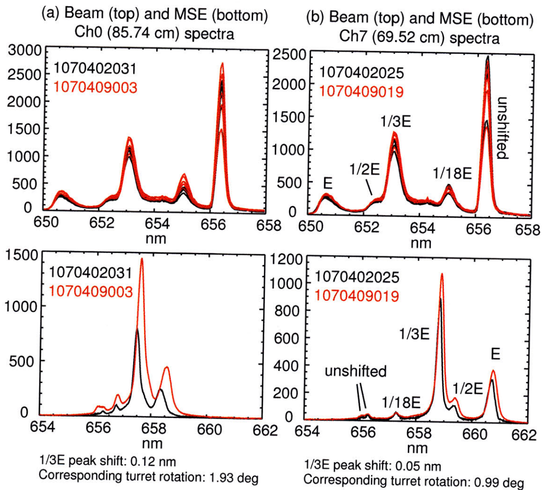
Figure D-2: Beam (top) and MSE (bottom) spectra from two beam-into-He gas runs with zero field (1070402 and 1070409) for (a) Channel 0 (edge) and (b) Channel 7 (core). Beam spectra have taken multiple times within a shot, showing multiple spectra for each shot. The shift in a third energy component peak between two spectrum runs in each channel is shown at the bottom along with the estimated MSE turret rotation that can give this much of the shift.
