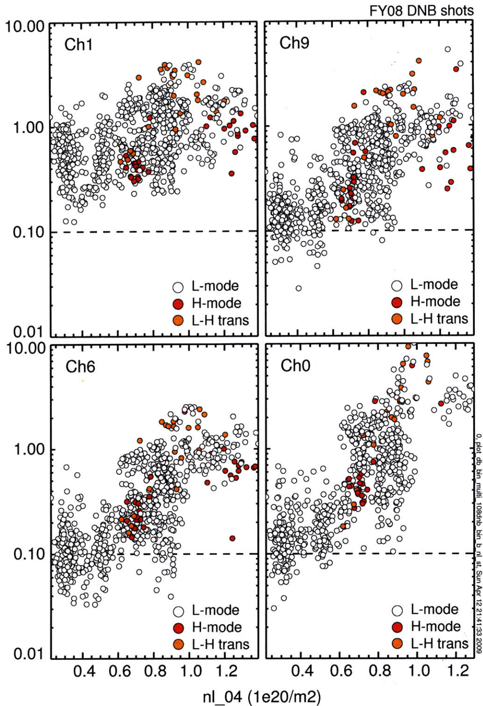
Figure 2-50: Macro-bin pitch angle error in degree vs plasma density, nl_{04}(10^{20} \text{ m}^{-2}) for the MSE channels 1 (87.21 cm), 9 (81.75 cm), 6 (75.74 cm) and 0 (68.94 cm) from FY2008 shots with DNB sorted by L-mode, H-mode, and L-H transition. Constraints are macro-bin timing > 50 ms, time between 0.5 ~ 1.7 sec, signal-to-background ratio > 1 , and beam current > 6 A.
