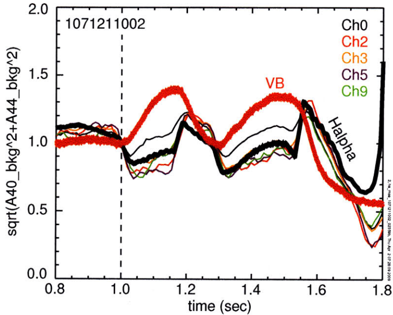
Figure 2-19: The time evolution of the Z brightness and H_{\alpha} along with the MSE background from several MSE channels from Shot 1071211002 with the new steep-edge filters installed. The signals are normalized at 1 sec (dashed line). This is directly compared with Fig 2-15 which is the case without the steep-edge filters
