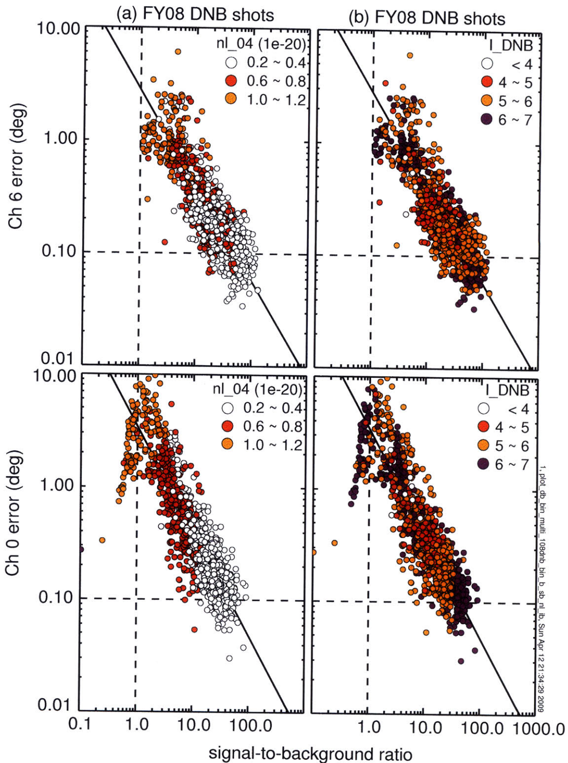
Figure 2-49: Macro-bin pitch angle error in degree vs signal-to-background ratio for the MSE channels 6 (Top: 75.74 cm) and 0 (Bottom: 68.94 cm) from FY2008 shots with DNB sorted by (a) 3 different density ( nl_{04} in 10^{20} \text{ m}^{-2} ) ranges and (b) 4 different beam current ( I_{DNB} in A) ranges. The solid line is the linear fit of the data on the log scale.
