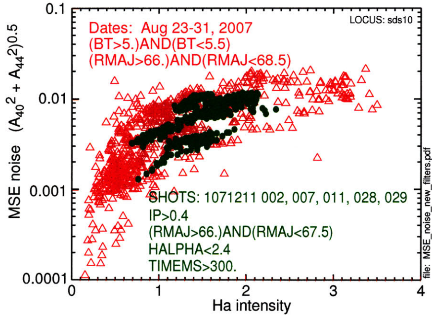
Figure 2-20: The magnitude of MSE noise as a function of H_\alpha for the MSE channels with major radii between about 66 ~ 68 cm from two groups of shots: before (red triangle) and after (green circle) the edge filter installation.
