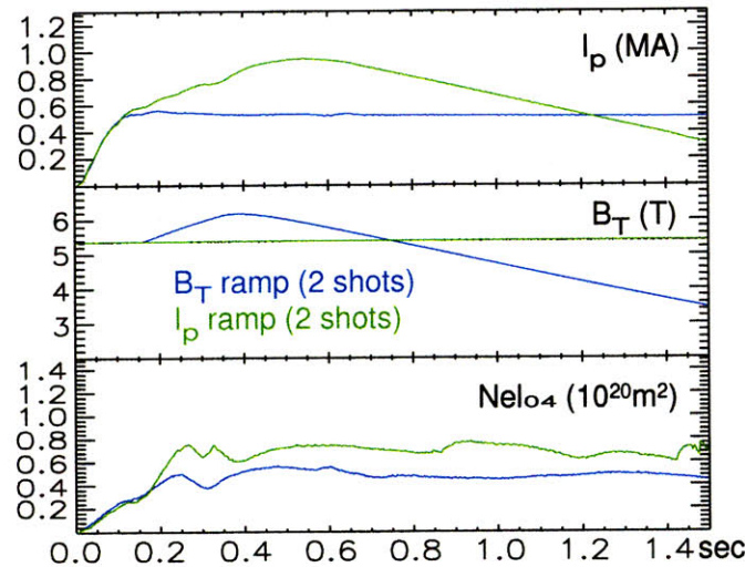
Figure 2-9: The waveforms of I_p , B_T , and nl_{04} for the Faraday rotation test using the invessel WGP. Two I_p -constant and B_T -ramping shots (1051108020, 1051108024) and Two B_T -constant and I_p ramping shots (1051108027, 1051108029) are used.
