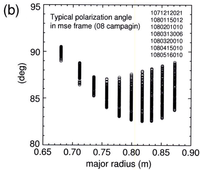
Figure E-6: (a) An example configuration for the in-situ single-waveplate calibration scheme that is capable of calibrating an 8°-range of angles. (b) EFIT-calculated pitch angle converted into the polarization angle in the MSE frame as a function of MSE major radius. The shots are from the FY08 campaign and include some high-field (~ 7 T) shots.
