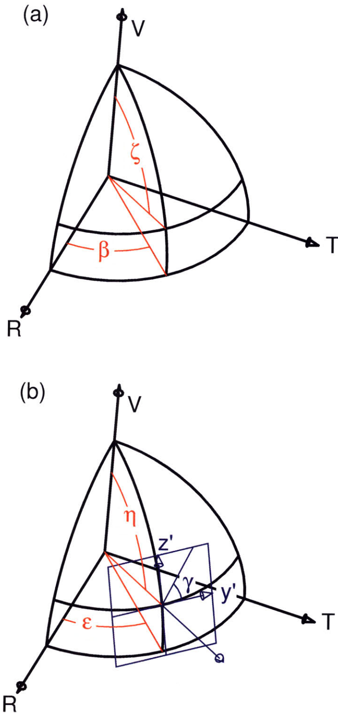
Figure A-1: Local spherical coordinate systems representing (a) the DNB vector and (b) the MSE line-of-sight vector
