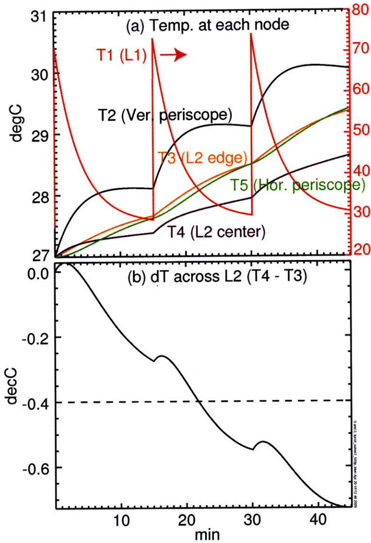
Figure 3-14: Numerical solution to Eqn G.29 with the configuration given in Figs G-2 and G-3 for three consecutive shots with q_e = 220 \text{ kW/m}^2 for 2 seconds every 15 minutes with a fixed wall temperature of 300 Kelvin. (a) shows the temperature time evolution at each node and (b) the temperature difference between the center and the edge of L2 (center - edge).
