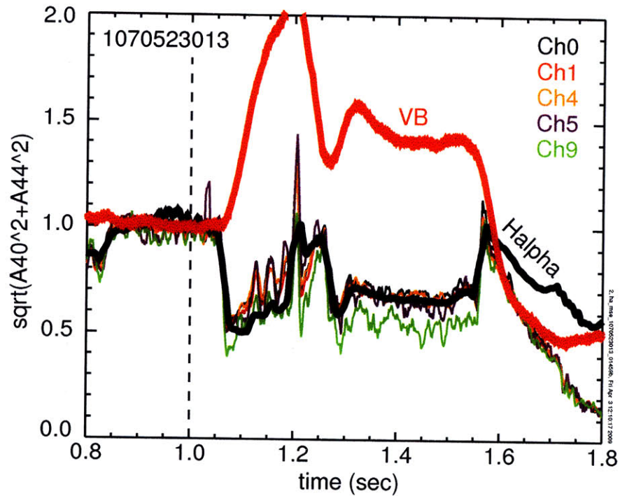
Figure 2-15: Time evolution of the Z brightness and H_\alpha along with the MSE background from several MSE channels during the H-mode from Shot 1070523013 shown in Fig 2-14. The signals are normalized at a time near the L-H transition, which is marked with a vertical dashed line.
