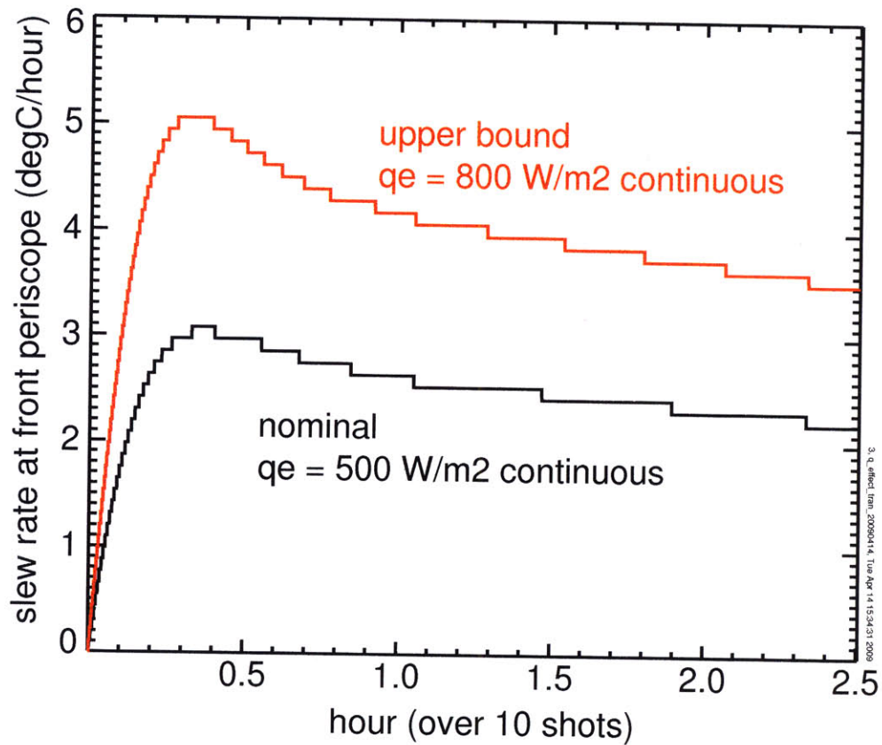
Figure 3-13: Time evolution of the temperature slew rate at the periscope front surface for nominal (black) and upper-bound (red) q_e values. Torus wall temperatures are fixed at 27 °C. Emissivities of plasma facing and periscope inner surfaces are assumed to be unity.
