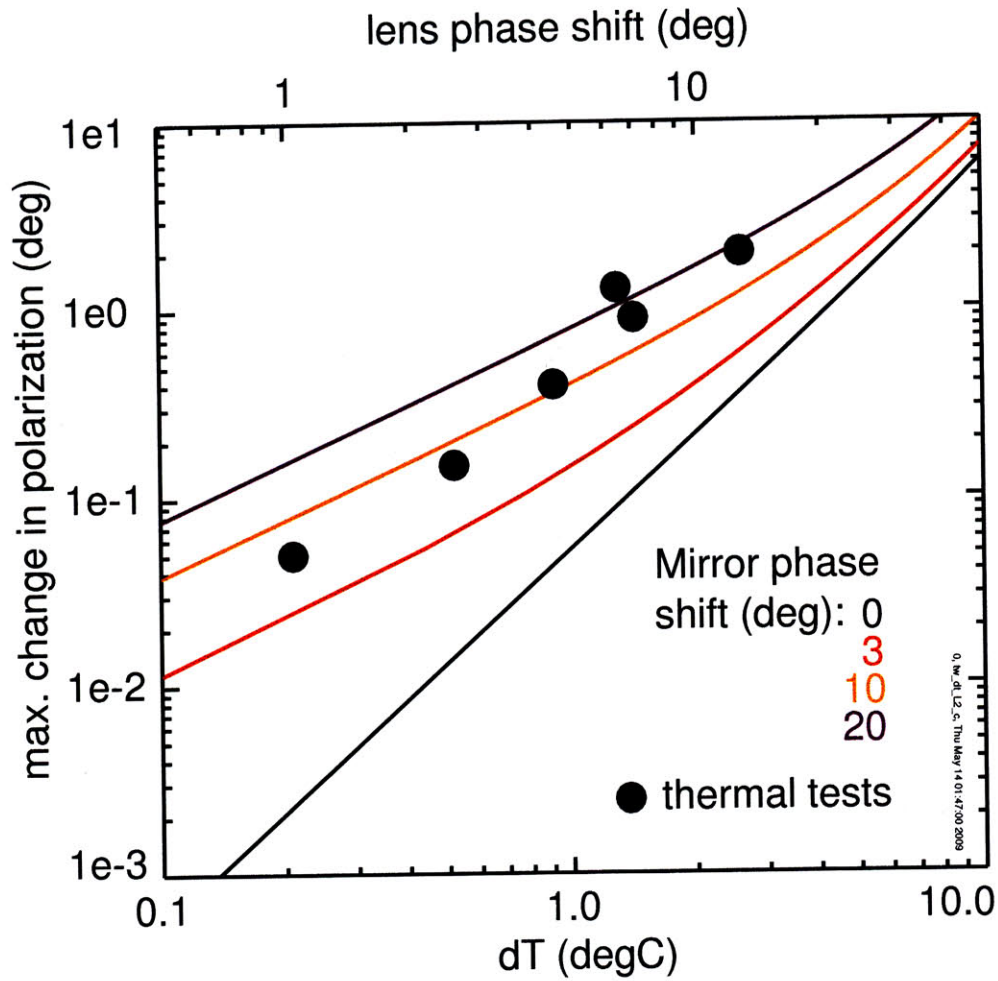
Figure 3-20: Scaling of the maximum change in polarization direction as a function of the magnitude of phase shift of the lens, E , and the temperature variability across the lens for four different mirror phase shifts, \epsilon . The maximum is taken over all input polarization angles and all orientations of the fast axis of the lens. The fast axis of the mirror, \phi , is assumed to be horizontal. The points are from thermal bench tests.
