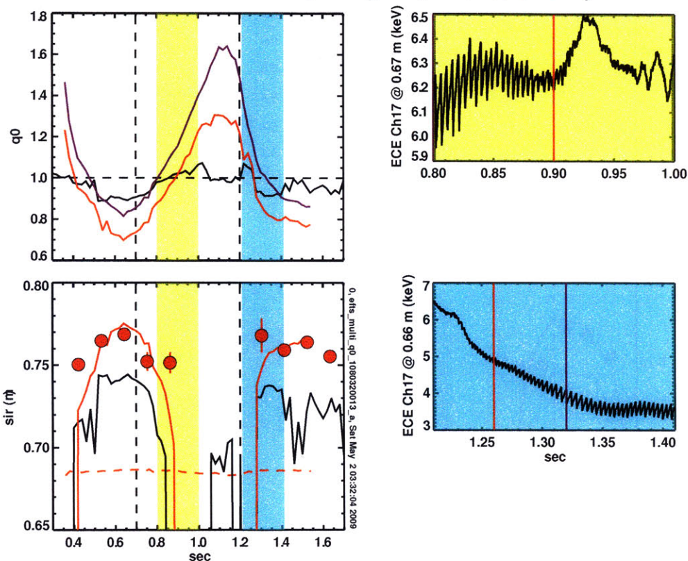
Figure 4-9: Time evolutions of q_0 (TOP LEFT) and SIR (BOTTOM LEFT) calculated by the ANALYSIS (black), EFIT16 (purple), and EFIT17 (red) equilibrium reconstructions for 1080320013. The LHC pulse duration is marked as two vertical lines. In the bottom plot, the raw SIR data from ECE is included and the magnetic axis is marked with a red dashed line. Time evolutions of electron temperature from two shaded (in yellow and cyan) areas are separately plotted on the right column. In each plot on the right column, the vertical lines indicate the time when q_0 crosses 1 (becoming either larger or smaller than 1) in a color which corresponds to either EFIT16 or EFIT17.
