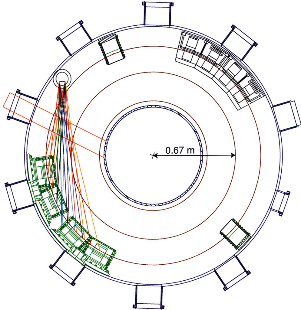
Figure 1-2: Plan view of the C-Mod torus, the MSE lines of sight, and the DNB trajectory (red rectangle). The green structures are the ICRF antennas.
