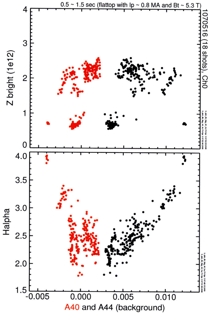
Figure 2-12: 40 and 44 kHz amplitudes in MSE background signals from Channel 0 (edgemoat channel; R = 85.7 cm) versus (a) Z brightness and (b) H_\alpha during the flatop phases.
