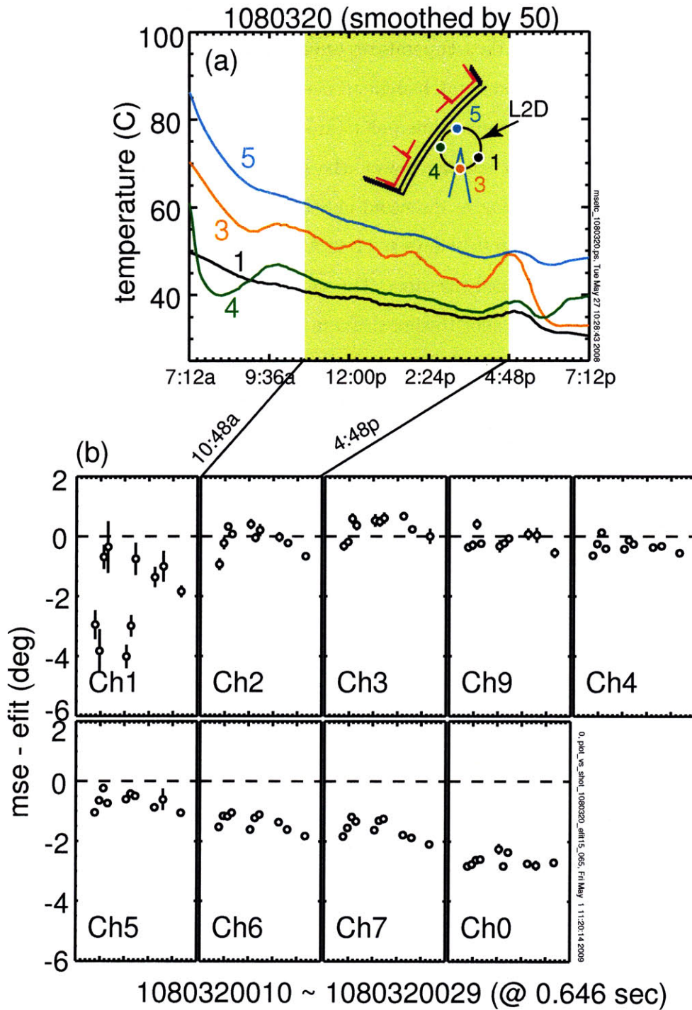
Figure 4-4: Time evolutions of (a) the temperatures around the MSE invessel periscope (L2 region) and (b) the deviation in pitch angle measured by MSE from the EFIT-predicted pitch angle at a flattop Ohmic time point (where I_p = 0.8 MA, B_T = 6.2 T, and nl_{04} = 3 \sim 4 \times 10^{19} \text{ m}^{-2} ) from the shots given in Table 4.1. The yellow shaded region in plot (a) is the horizontal range of the individual plots in (b) which are arranged in the major radius order (edge \rightarrow core).
