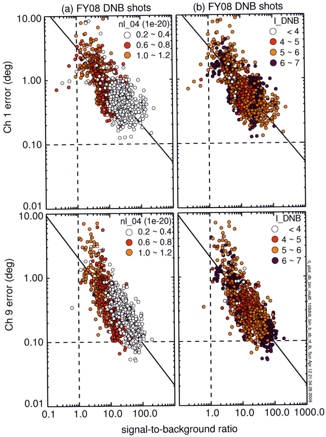
Figure 2-48: Macro-bin pitch angle error in degree vs signal-to-background ratio for the MSE channels 1 (Top: 87.21 cm) and 9 (Bottom: 81.75 cm) from FY2008 shots with DNB sorted by (a) 3 different density ( nl_{04} in 10^{20} \text{ m}^{-2} ) ranges and (b) 4 different beam current ( I_{DNB} in A) ranges. The solid line is the linear fit of the data on the log scale.
