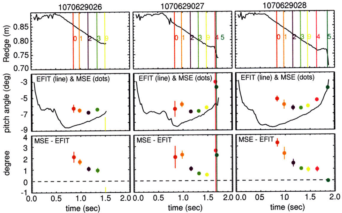
Figure 2-34: Plasma edge sweeping experiments from 1070629. The time evolution of plasma edge position (top) with the vertical lines indicating the MSE channel number whose position is swept by the plasma edge at that time point. The middle plots show the pitch angle measured by the channel marked with the same color shown on the top plot (point) with the pitch angle computed by EFIT (black line). The vertical lines for 1070629027 on the middle plot indicates those channels can be excluded in the analysis because the data from those channels are taken include some spurious signals at the moment of the plasma termination. The bottom plots show the difference in pitch angles between MSE and EFIT.
