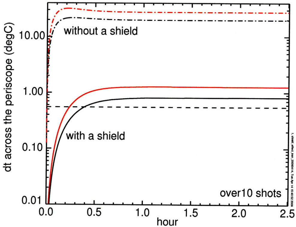
Figure 3-11: Time evolution of the temperature difference between the front and back sides of the periscope calculated by Eqn G.6 with single-shield (solid) and no-shield (dot-dashed) configurations for q_e = 500 (black) and 800 (red) W/m^2 . Torus wall temperatures are fixed at 27 °C. Emissivities of plasma facing and periscope inner surfaces are assumed to be unity. The horizontal line at 0.55 °C is the maximum allowable temperature variability across the periscope.
