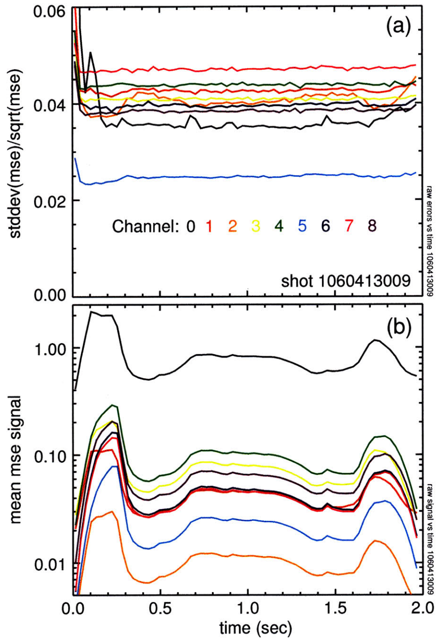
Figure 2-4: (a) The measured standard deviation in signal intensity, normalized to square-root of signal intensity ( \sigma_S/\sqrt{S} ), and (b) the measured intensity. Channel 0 signal is from APD and the rest of the channels from PMT. Binning time is 30 msec and PEM is off for this shot.
