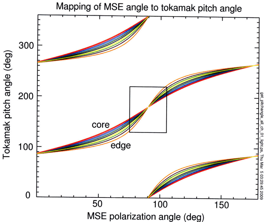
Figure A-4: Real tokamak pitch angle versus MSE polarization angle for ten MSE channels.
