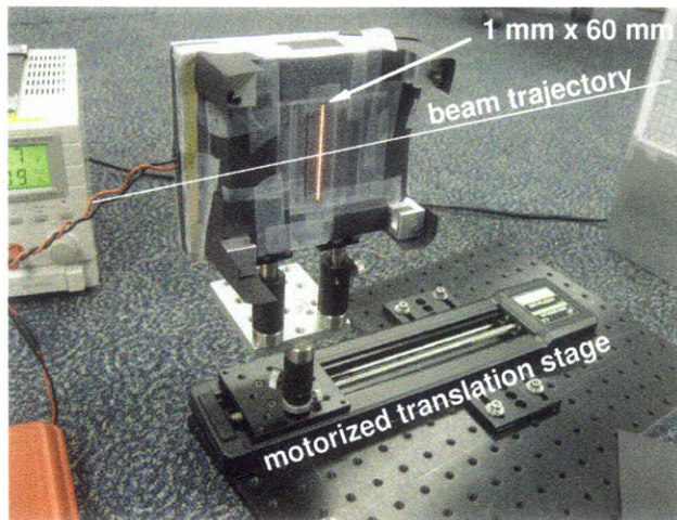
Figure 2-39: Setup for the radial intensity weighting calibration (Feb 13 2007)
