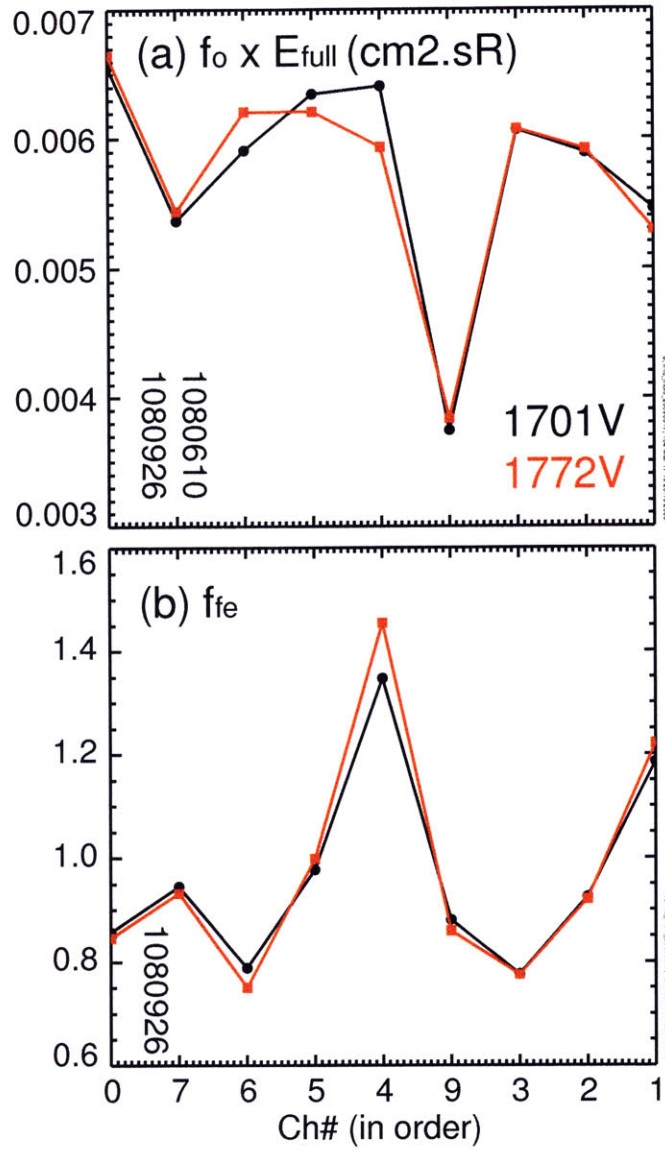
Figure 2-37: (a) The product of f_o E_{full} calculated by Eqn 2.30 and (b) The parameter f_{fe} calculated by Eqn 2.28 for two different HV_{fiber} .
