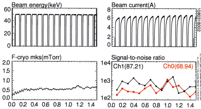
Figure 2-21: Typical beam-into-gas calibration conditions. The torus gas pressure ranges 0.3 ~ 3 mTorr. Signal-to-noise ratio is shown for the innermost (Ch0) and the outermost (Ch1) channels.
