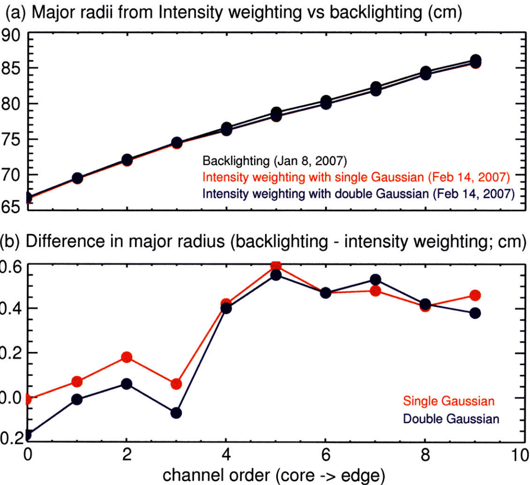
Figure 2-43: (a) Major radii as a function of channel order estimated from the invessel backlighting calibration (black) and the single (red) and double (blue) Gaussian fits of the intensity weighting calibration. (b) The deviation in the major radius of the single (red) and the double (blue) Gaussian fits from the backlighting calibration.
