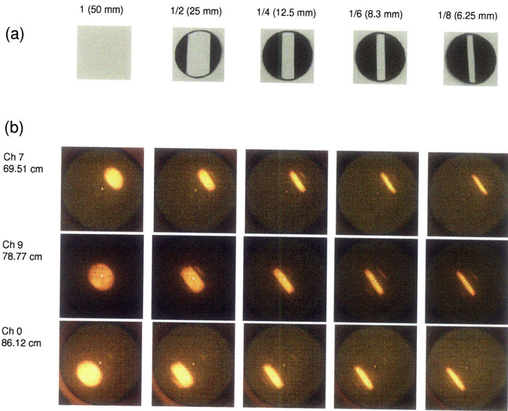
Figure B-5: (a) Aperture paper installed on L1 and (b) their images at the end of the optical train outside the F port for three MSE channels.
