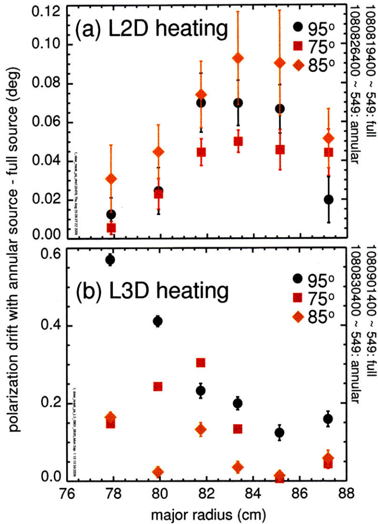
Figure E-9: The difference in the polarization drift between annular and full apertures on L1 as a function of MSE major radii from (a) L2D heating and (b) L3D heating bench tests. Both heating tests have 6 °C/h slew rate.
