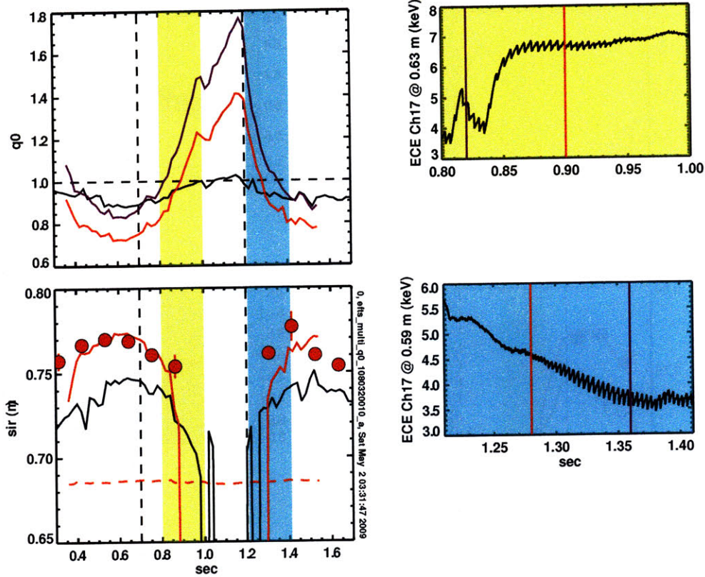
Figure 4-6: Time evolutions of q_0 (TOP LEFT) and SIR (BOTTOM LEFT) calculated by the ANALYSIS (black), EFIT16 (purple), and EFIT17 (red) equilibrium reconstructions for 1080320010. The LHCD pulse duration is marked as two vertical lines. In the bottom plot, the raw SIR data from ECE is included and the magnetic axis is marked with a red dashed line. Time evolutions of electron temperature from two shaded (in yellow and cyan) areas are separately plotted on the right column. In each plot on the right column, the vertical lines indicate the time when q_0 crosses 1 (becoming either larger or smaller than 1) in a color which corresponds to either EFIT16 or EFIT17.
