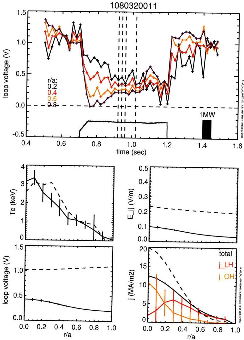
Figure 4-15: Time evolution of loop voltages at four radial locations (TOP) from 1080320011. The radial profiles of T_e , E_{||} , loop voltage, and three current densities (total, LH-driven, and Ohmic) averaged over the time points marked as vertical lines on the top plot are shown at the four plots at the bottom. The dashed curves on these profile plots are the profiles at ' t_0 ' (averaged over 0.6 ~ 0.65 sec). The waveform of the LH power applied to this shot is also illustrated at the top plot.
