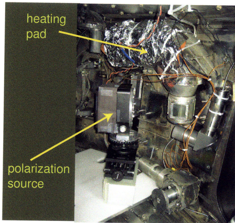
Figure C-1: MSE invessel periscope heating test setup. The heating pad is applied to most of the plasma-facing part of the periscope.
