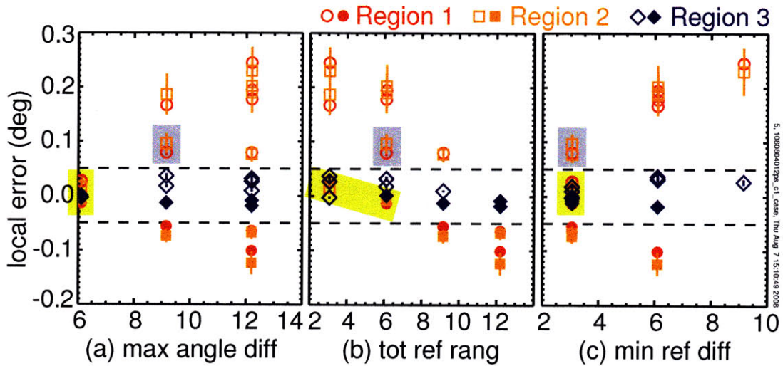
Figure E-3: Correlations between the local calibration error from each region and the three case parameters, (a) maximum angle difference, (b) total reference range, and (c) minimum reference distance all in degree using the single-waveplate scheme. Different colors and symbols denote the errors from different regions shown in Fig E-1. Filled symbols indicate the tested angle is between two references and empty symbols indicate otherwise. The acceptable range of the error ( \pm 0.05^\circ ) is marked as two horizontal dashed lines.
