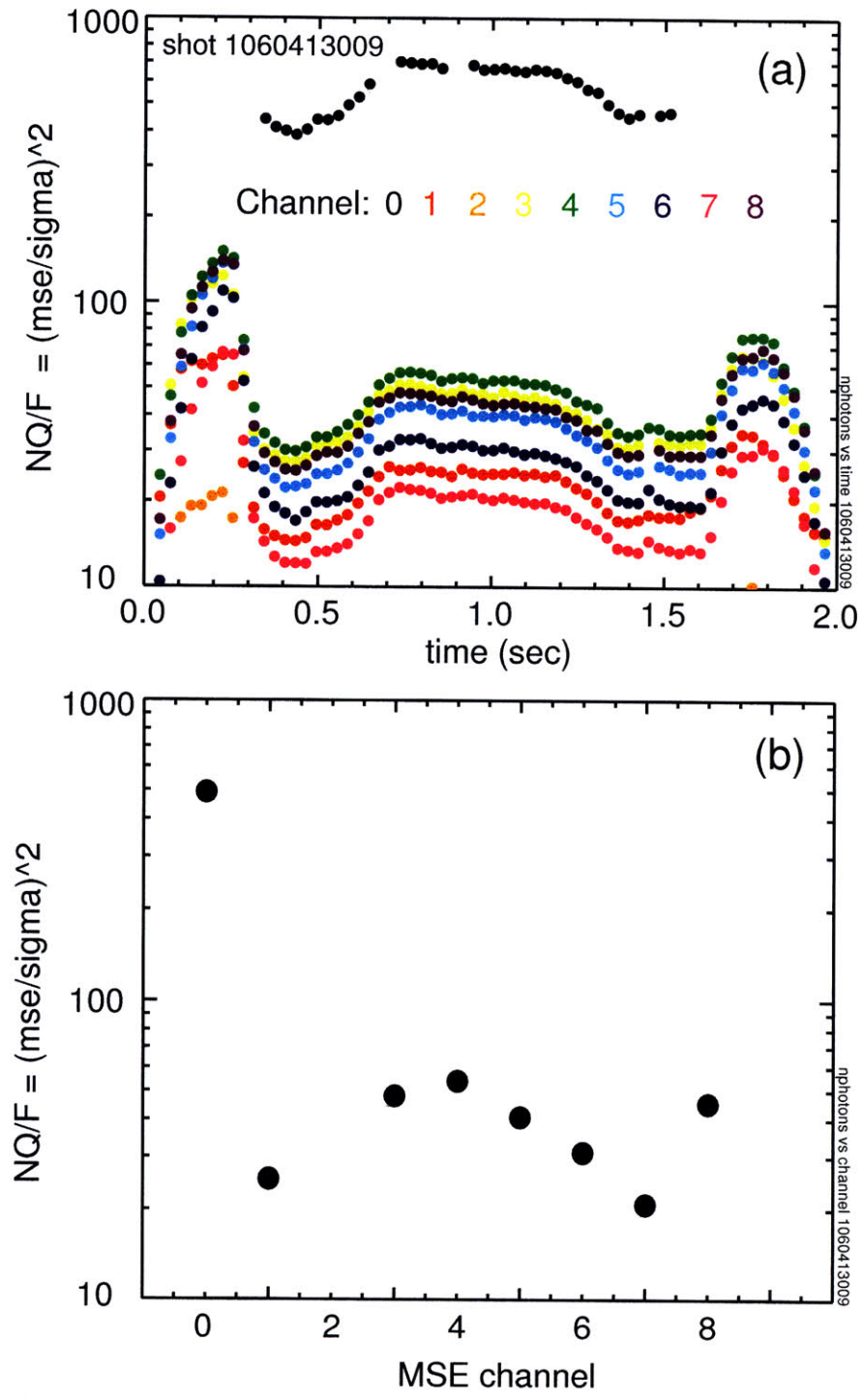
Figure 2-5: (a) Square of the measured intensity normalized by its standard deviation ( S^2/\sigma_S^2 ) which corresponds to the quantity NQ/F , and (b) the same quantity (shot-averaged) as a function of MSE channel number. Channel 0 signal is from APD and the rest of the channels from PTM. Binning time is 30 msec and PEM is off for this shot.
