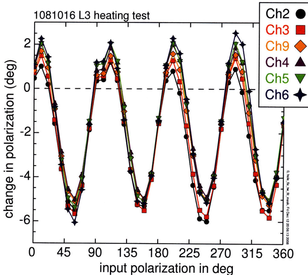
Figure 3-18: Change in the polarization angle from the L3 heating test with the input polarization scan for 6 MSE channels.
