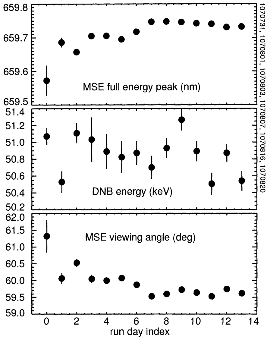
Figure D-3: Run-to-run variations of MSE full energy peak (top), DNB energy (middle), and MSE viewing angle (bottom) inferred from the zero-field beam-into-He gas spectrum measurements over 6 run days (1070731 ~ 1070820). The details on the horizontal axis ('run day index') are described in the text.
