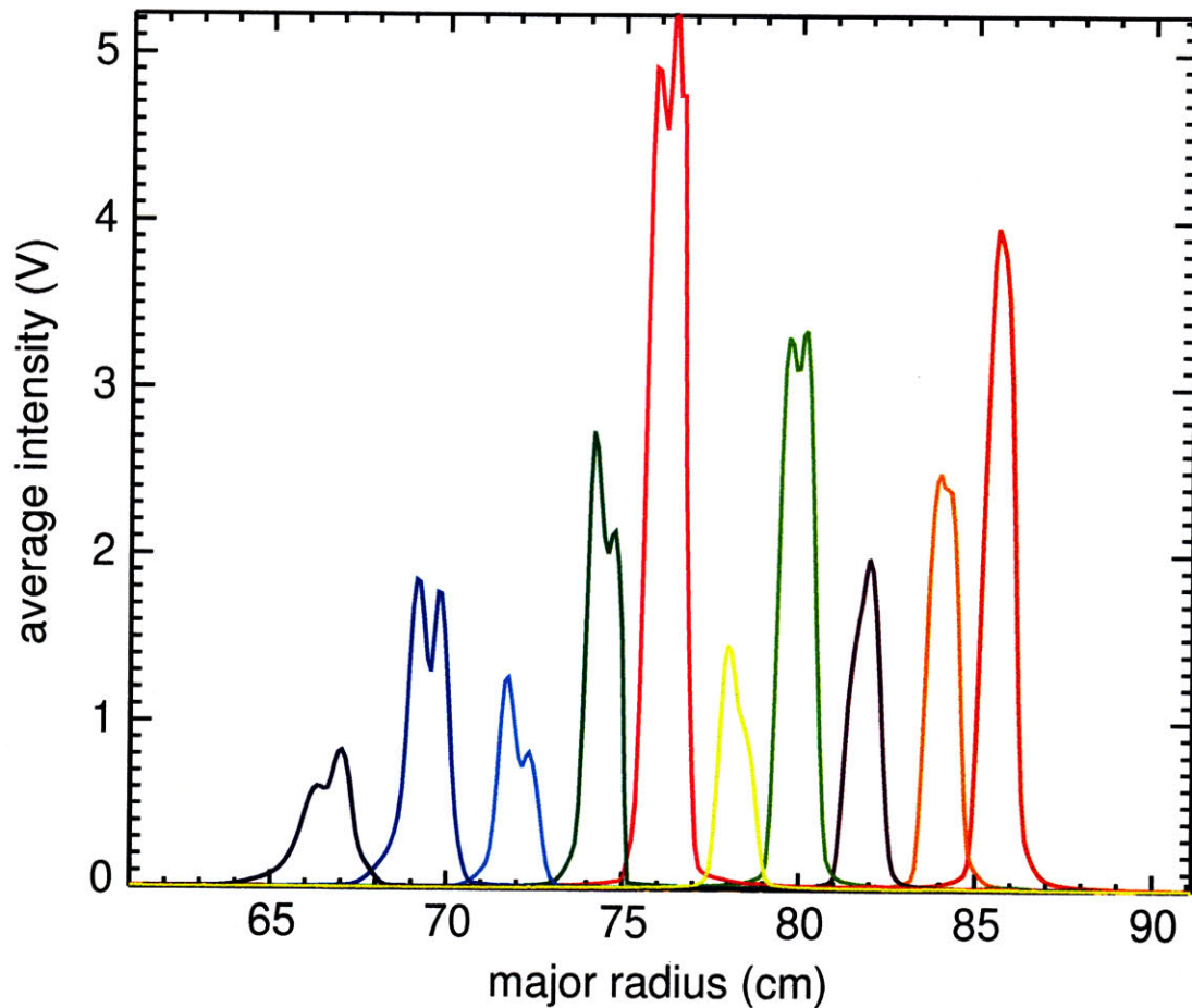
Figure 2-40: Result of intensity weighting calibration. The intensity is measured for each channel while the 1 mm \times 60 mm-slit light source shown in Fig 2-39 is translated along the DNB trajectory on the midplane by 1 mm per shot. The signal from each channel, after the background subtraction, is plotted here as a function of major radius (that is, shot number) in a different color. The saturated shots have been taken care of by replacing them with the shots taken separately with a lower bias voltage and with a corrected magnitude. Note there are ten peaks from ten MSE channels.
