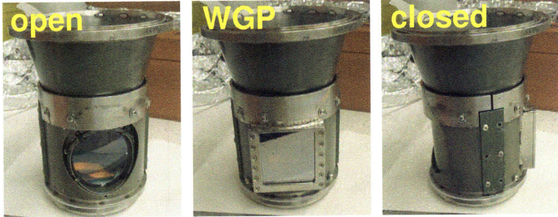
Figure 2-6: Three possible rotational positions of the upgraded MSE shutter. The WGP allows the MSE system to respond to non-motional-Stark-effect-induced polarized light. The shutter is controlled by the push-pull mechanism.
