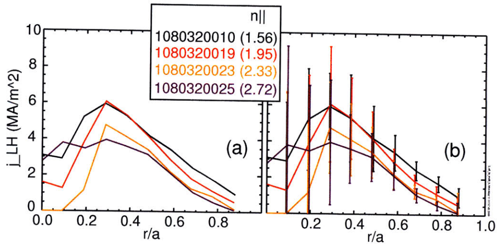
Figure 4-17: Radial profile of J_{LH} for four different n_{||} (a) without and (b) with the uncertainties.
