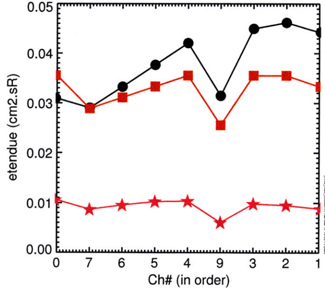
Figure 2-38: Comparison of étendue based on Eqn 2.30 and measured f_o ('star') with E_{full} ('circle') and E_{fiber} ('square') calculated at L1 using Eqn 2.31 and the fiber entrance using Eqn 2.32, respectively.
