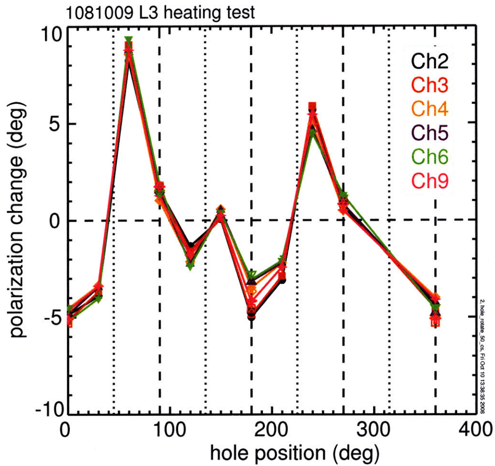
Figure 3-17: Change in the polarization angle from the L3 heating test with the hole-aperture scan for 6 MSE channels. Also shown in the figure are the data points (empty symbols) at some hole positions ( 180^\circ and 360^\circ ) which are taken from a separate test with the same kind of setup, reflecting a good reproducibility.
