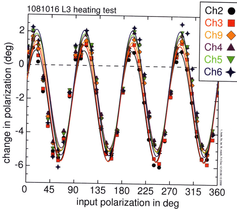
Figure 3-21: Data shown in Fig 3-18 with the fit using the dual-waveplate model: Change in the polarization angle from the L3 heating test with the input polarization scan for 6 MSE channels (Ch2:edge \rightarrow Ch6:core).
