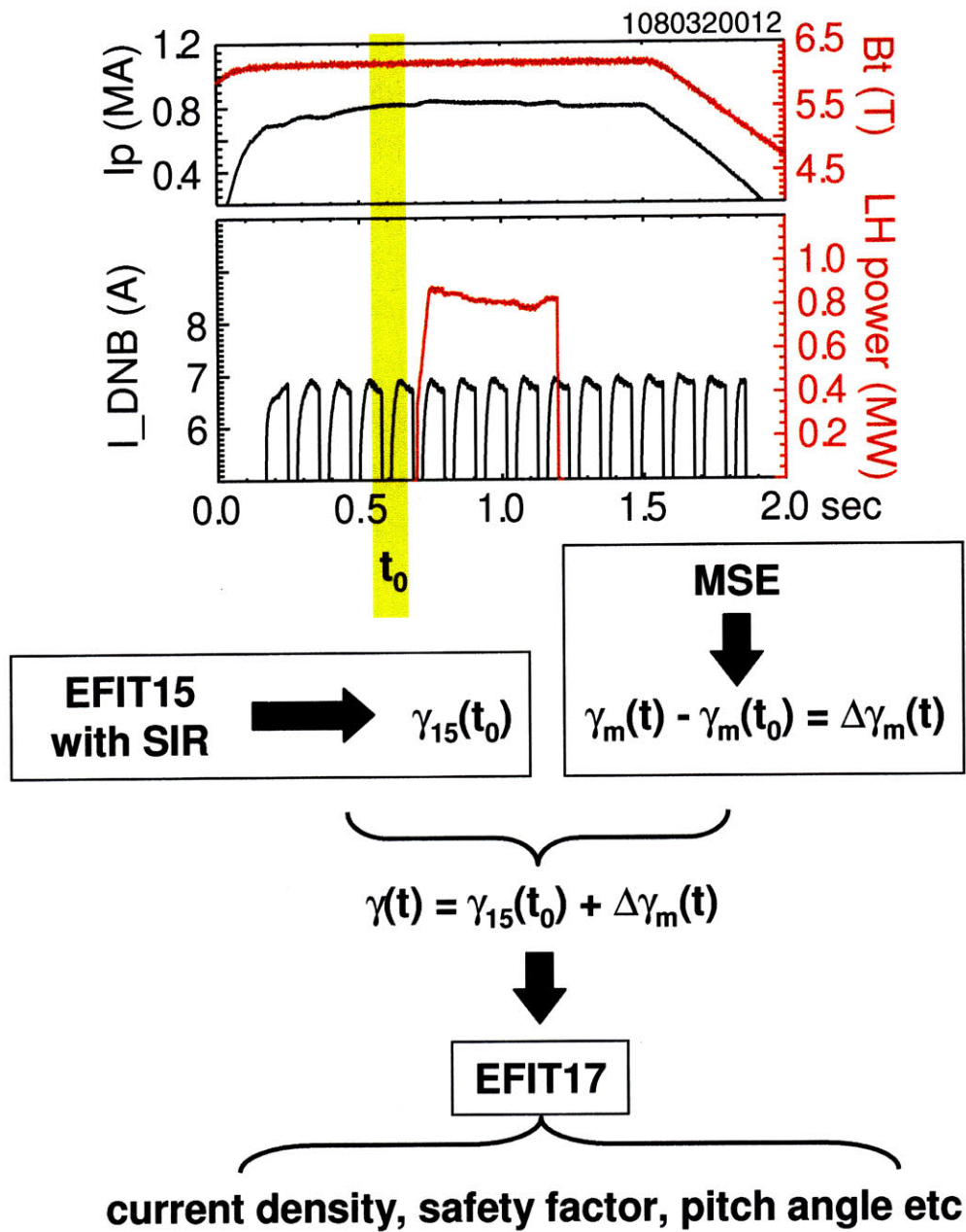
Figure 4-5: Schematic diagram for the within-shot calibration procedure.
