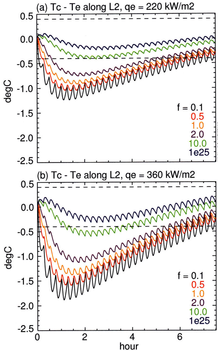
Figure 3-15: Time evolution of temperature difference across L2 from the numerical solution to Eqn G.29 over 30 consecutive shots for 6 different multiplication factors ( f ) to the nominal R_{L2o}^c , the conductive thermal resistance across the Viton o-ring given in Table G.3 with q_e = (a) 220 \text{ kW/m}^2 and (b) 360 \text{ kW/m}^2 for 2 seconds every 15 minutes with a fixed wall temperature of 300 Kelvin.
