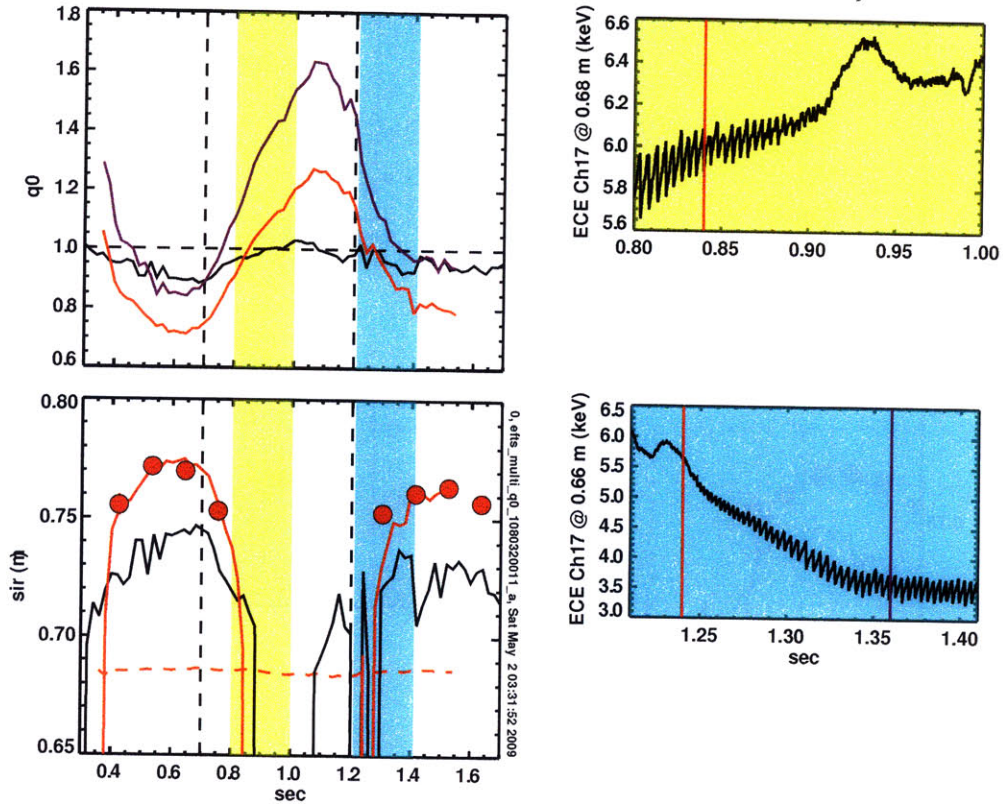
Figure 4-7: Time evolutions of q_0 (TOP LEFT) and SIR (BOTTOM LEFT) calculated by the ANALYSIS (black), EFIT16 (purple), and EFIT17 (red) equilibrium reconstructions for 1080320011. The LHCD pulse duration is marked as two vertical lines. In the bottom plot, the raw SIR data from ECE is included and the magnetic axis is marked with a red dashed line. Time evolutions of electron temperature from two shaded (in yellow and cyan) areas are separately plotted on the right column. In each plot on the right column, the vertical lines indicate the time when q_0 crosses 1 (becoming either larger or smaller than 1) in a color which corresponds to either EFIT16 or EFIT17.
