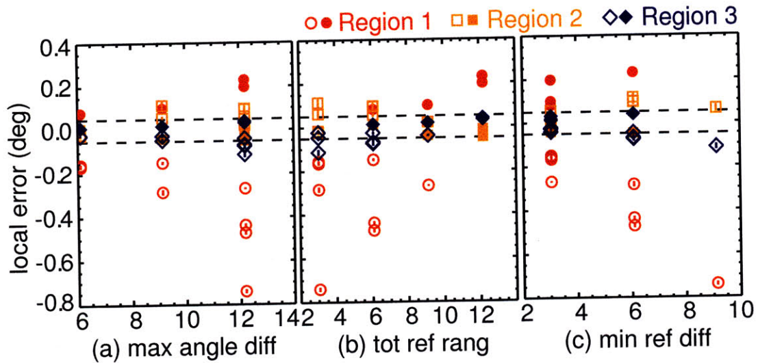
Figure E-4: Correlations between the local calibration error from each region and the three case parameters, (a) maximum angle difference, (b) total reference range, and (c) minimum reference distance all in degree using the linear-fit scheme. Different colors and symbols denote the errors from different regions shown in Fig E-1. Filled symbols indicate the tested angle is between two references and empty symbols indicate otherwise. The acceptable range of the error ( \pm 0.05^\circ ) is marked as two horizontal dashed lines.
