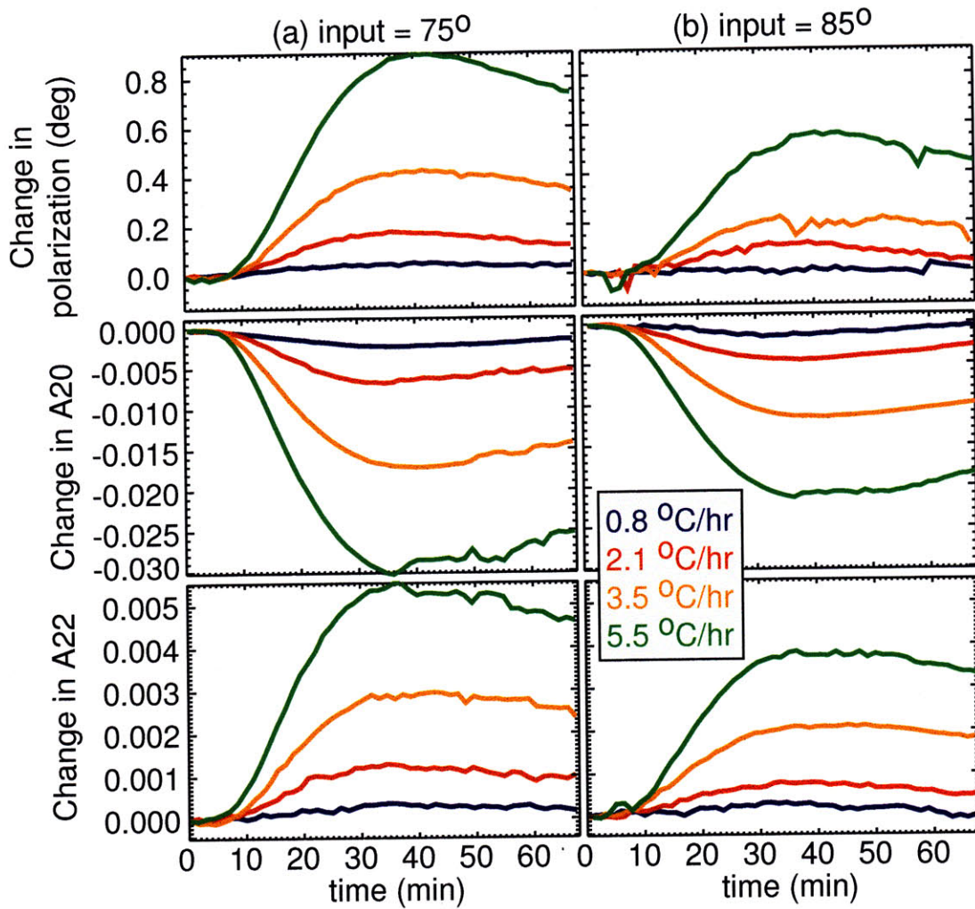
Figure 3-5: Change in the measured polarization angle (top) compared with the changes in the amplitudes of the 20 (middle) and 22 (bottom) kHz components from the L2-region heating tests on the bench with 4 different temperature slew rates which are given in the box on the plot. Two fixed input polarization angles are tried: (a) 75° and (b) 85°. These results are from the MSE channel 1, the edgemoat channel, that tends to have the largest change when the L2 region is heated.
