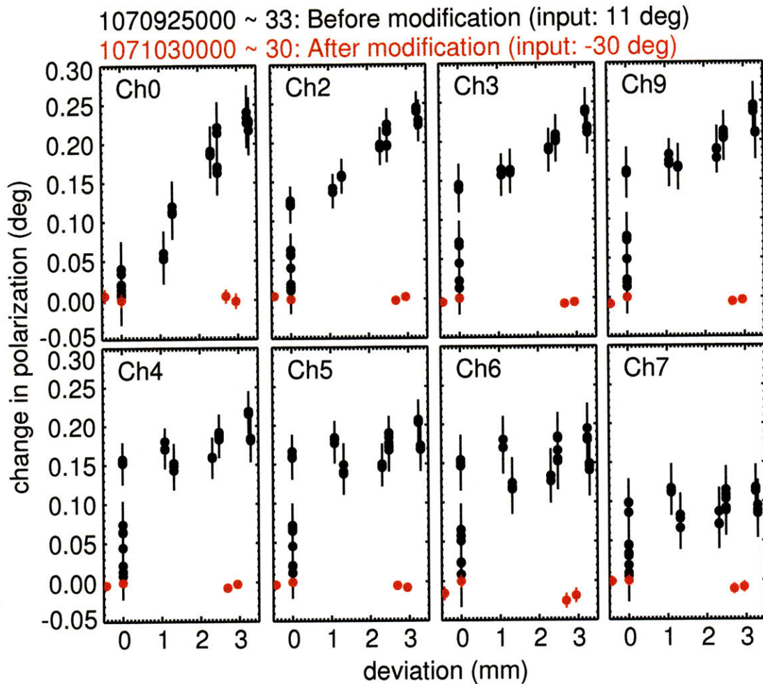
Figure C-4: Comparison of the stress effect on the L2D before and after the L2D holder modification. The change in the polarization angle has been plotted as a function of 'deviation' of the hose clamp diameter from the non-stress value, which is proportional to the amount of stress applied. The plots are arranged in the channel order.
