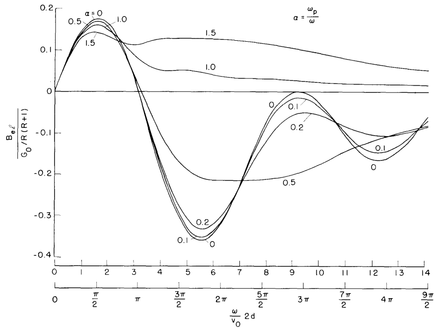
Fig. VI-14. Electronic-loading susceptance.
