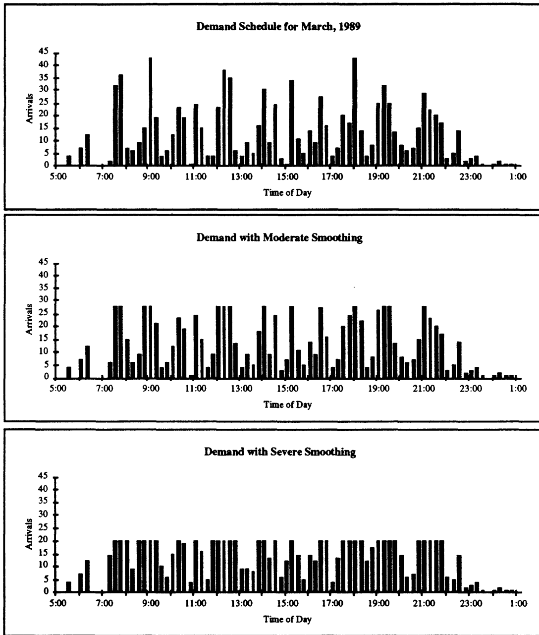
Figure 14: Alternative degrees of smoothing for DFW traffic
