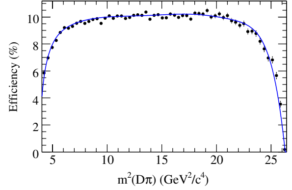
FIG. 7 (color online). The efficiency for signal decays as a function of m^2(D\pi) , as determined by MC simulation (points with statistical errors) and the results of the fit to the accepted and generated distributions (solid curve).
