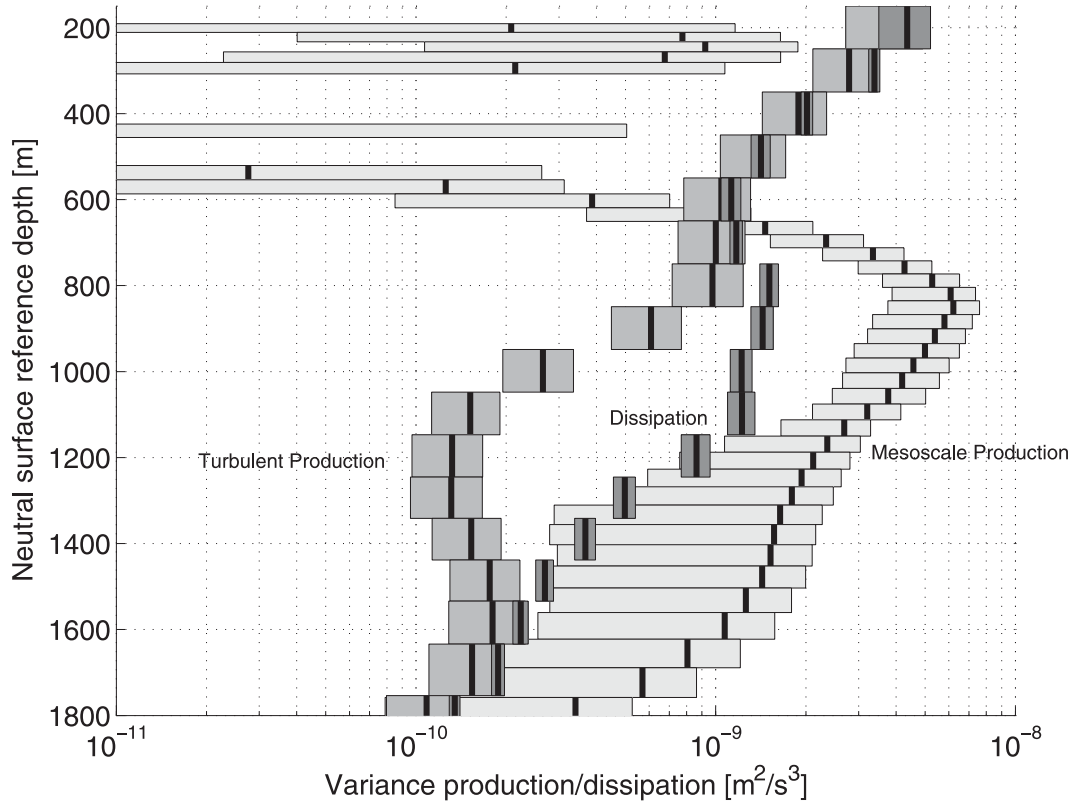
FIG. 9. The simulated production of temperature variance by lateral stirring in the central simulation ( -\sqrt{T} \cdot \overline{\mathbf{u}'T'} ; light gray). Also shown are microstructure estimates of temperature variance dissipation (darkest gray) and the production of variance by turbulent motions acting on the mean diapycnal gradient (medium gray). The shaded boxes for the microstructure data represent the error bars and for the mesoscale production indicate maximum and minimum simulated values in the equilibrated phase. The turbulent variance estimates were made using the Osborn (1980) model applied to the NATRE dataset (see Ferrari and Polzin 2005 for details).
