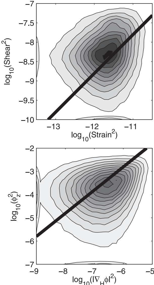
FIG. 14. (Top) The 2D PDF of |\mathbf{u}'_z|^2 and \sigma^2 at 1100-m depth. (bottom) The 2D PDF of \phi_z^2 and |\nabla\phi|^2 at 1100-m depth. In each panel, the thick black line represents the line with slope [N(1100\text{ m})/f]^2 .
