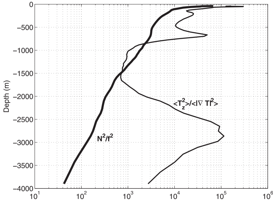
FIG. 16. Comparison of the squared Prandtl ratio (N/f)^2 to the inverse squared slope of the temperature field, \langle T_z^2 \rangle / \langle |\nabla T|^2 \rangle , for the central simulation.
