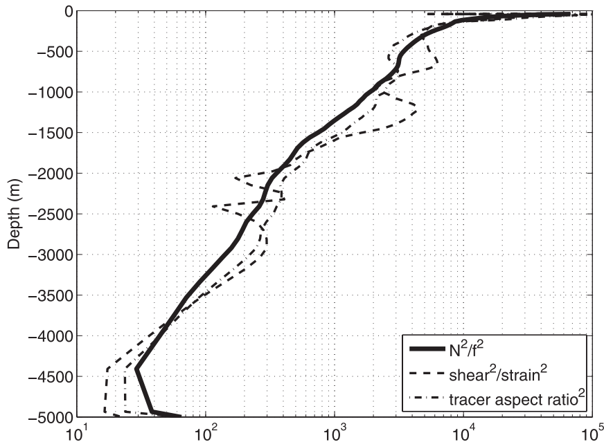
FIG. 13. Comparison of the squared Prandtl ratio (N/f)^2 (solid), squared shear over strain |u'_z|^2/\sigma^2 (dashed), and inverse squared tracer slope \overline{\phi_z^2}/|\nabla\phi|^2 (dashed-dotted) for the central simulation. The strain is computed as \sigma^2 = \overline{(u'_y + v'_x)^2 + (u'_x - v'_y)^2} , where the overbar denotes both a time and horizontal spatial average.
