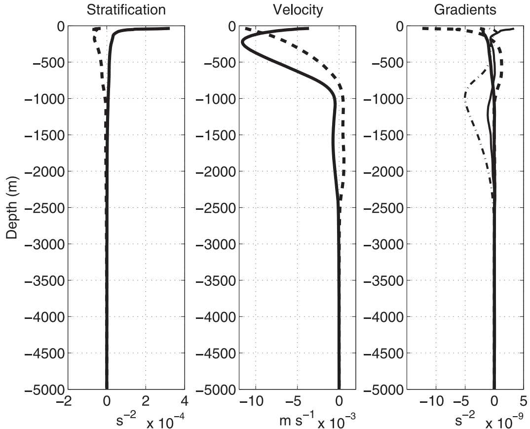
FIG. 3. Mean vertical structure of NATRE region: (left) mean stratification N^2 (solid) and equivalent for spice N_\gamma^2 (dashed line); (middle) mean velocity \bar{u} (solid line) and \bar{v} (dashed); (right) mean horizontal gradients of buoyancy [thick solid line: -(g/\rho_0)d\bar{p}/dx = f_0 d\bar{v}/dz and dashed line: -(g/\rho_0)d\bar{p}/dy = -f_0 d\bar{u}/dz ] and spice [thin solid line: -(g/\rho_0)d\bar{\gamma}/dx and dashed-dotted line: -(g/\rho_0)d\bar{\gamma}/dy ].
