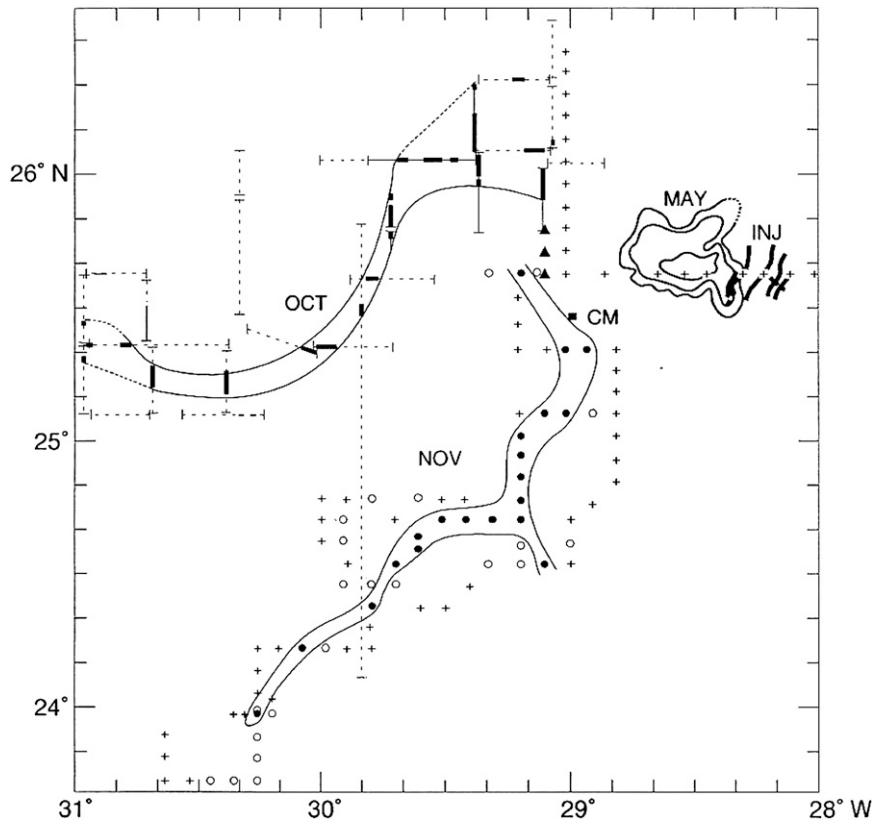
FIG. 2. Column-integrated tracer concentrations from NATRE. Injection streaks are shown as short heavy lines near 26^{\circ}\text{N} , 28^{\circ}\text{W} . Closed contours define a smoothed map of the patch at the initial (two week) survey. The sinuous features to the west and southwest define tracer filaments encountered during the 6-month survey. CM marks the location of the Subduction Experiment central mooring.
