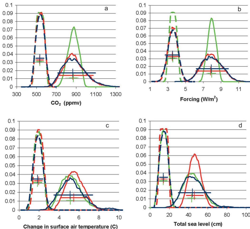
FIG. 11. Frequency distributions for (a) atmospheric \text{CO}_2 concentrations, (b) radiative forcing due to GHGs and sulfate aerosol, (c) surface air temperature, and (d) total sea level rise in simulations with full uncertainty (blue), climate uncertainty (green), and emissions uncertainty (red) averaged over 2041–50 (dashed lines) and 2091–2100 (solid lines).
