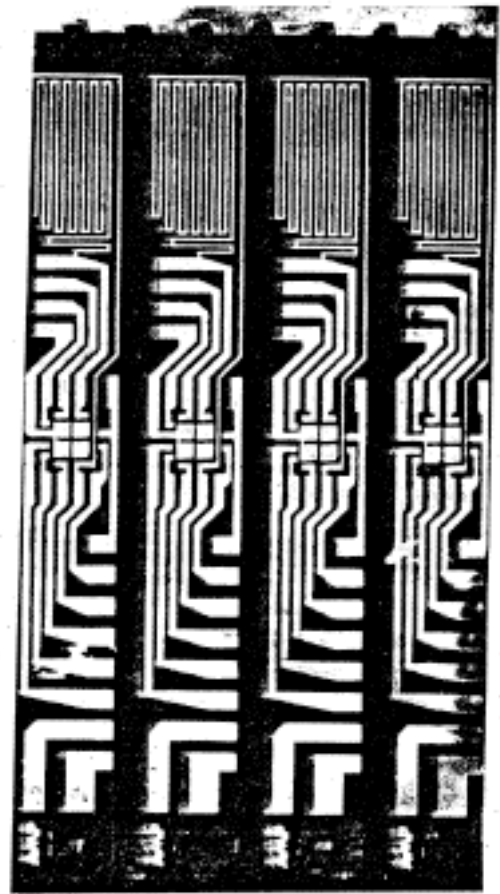
Figure 8: Film-carrier strip.
