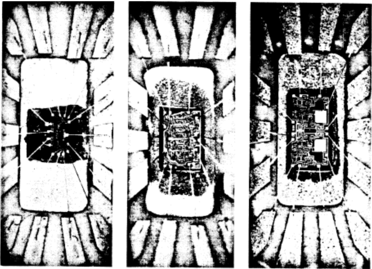
Figure 3: Typical integrated circuit chips lead-bonded into fourteen-pin dual-inline-packages using one-mil aluminium wire.
