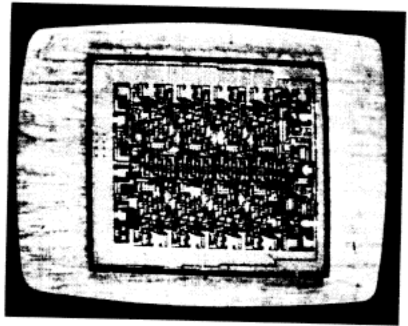
Figure 9: Micrograph and photo of TV monitor image of integrated circuit chip with bright aluminium border. Note dark gap in the border.
