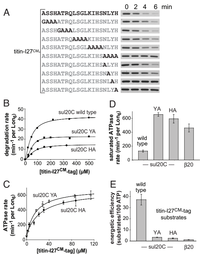
Fig. 3. Mutant sul20C tags alter Lon activity. (A) SDS/PAGE assays of Lon 6 (0.15 μM) degradation of titin-I27 CM (5 μM) bearing mutant sul20C tags. (B) Steady-state rates of Lon 6 (0.3 μM) degradation of different concentrations of 35 S-titin-I27 CM bearing wild-type, YàA (penultimate residue), or HàA (C-terminal residue) sul20C tags were fit to the Hill equation. (C) ATP hydrolysis by Lon 6 (0.15 μM) as a function of [titin-I27 CM - sul20C ] bearing the penultimate YàA mutation or C-terminal HàA sul20C mutations. Lines are fits to the equation rate = basal + (V max -basal)·[S]/(K 0.5 + [S]). (D) Rates of Lon ATP hydrolysis at saturating concentrations of titin-I27 CM with different degradation tags. Values are averages (n = 3) ± 1 SD. (E) The energetic efficiency of Lon degradation varies dramatically for titin-I27 CM variants with different degrons. Error bars are 1 SD.
