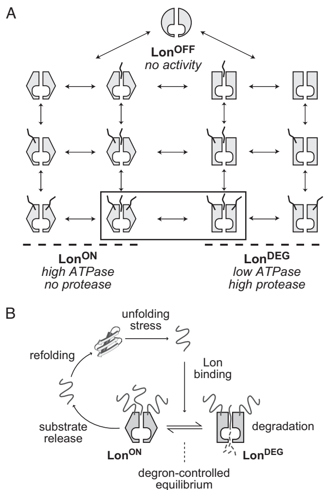
Fig. 4. Models for allosteric control of Lon. (A) Model showing equilibrium states of a system with three Lon conformations: Lon OFF (no activity), Lon ON , and Lon DEG (depicted by different shapes). Degrans are shown as squiggly lines. One degron-binding site in the axial pore of Lon and two flanking allosteric binding sites are depicted. At substrate saturation, the relative affinity of the degron for Lon ON versus Lon DEG determines the equilibrium distribution of the two fully liganded species shown in the rectangle. (B) Model in which an unfolded protein binds Lon and then partitions between a degradation pathway mediated by Lon DEG or a refolding pathway mediated by Lon ON and possibly other cellular chaperones. The substrate degron determines the equilibrium distribution of the two forms of Lon and thus determines which pathway is favored.
