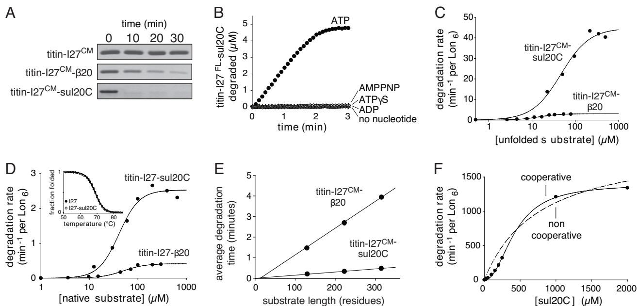
Fig. 1. Lon degradation of denatured and native proteins. (A) SDS/PAGE assays of Lon 6 (0.15 \mu M) degradation of untagged and tagged variants of unfolded titin-I27 CM (5 \mu M). (B) Lon 6 (0.3 \mu M) cleavage of sul20C-tagged titin-I27 (5 \mu M), unfolded by fluorescein modification of its cysteines, was assayed in the presence of no nucleotide or 2 mM ATP, ATP \gamma S, AMPPNP, or ADP. (C) Steady-state rates of Lon 6 (0.1 \mu M) degradation of different concentrations of sul20C-tagged or \beta 20-tagged 35 S-titin-I27 CM . Lines are fits to the Hill equation (rate = V_{max} \cdot [S]^n / (K_M^n + [S]^n) ). (D) Steady-state rates of Lon 6 (0.3 \mu M) degradation of native 35 S-titin-I27-sul20C or 35 S-titin-I27- \beta 20 were fit to the Hill equation. Inset , Titin-I27 (closed symbols) and titin-I27-sul20C (open symbols) had the same stability to thermal unfolding monitored by changes in circular dichroism. (E) Average degradation times normalized to Lon 6 (0.3 \mu M) are plotted as a function of substrate length for \beta 20-tagged (20 \mu M) or sul20C-tagged (50 \mu M) substrates containing 1–3 copies of titin-I27 CM . Values are averages ( n = 3 ), with standard deviations smaller than the plot symbol. (F) Degradation of sul20C peptide by Lon 6 (0.3 \mu M) shows strong positive cooperativity. The solid and dashed lines are fits to the Hill equation ( n = 2.2 ) and a noncooperative equation, respectively.
