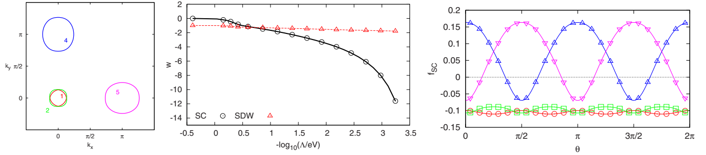
FIG. 2. (Color online) Left panel: the k_z=0 Fermi surfaces of LaFePO. Middle panel: the FRG flow of the interaction strength associated with the (\pi,0) SDW and the superconducting pairing. \Lambda is the energy cutoff. Right panel: the pairing form factor. The horizontal axis \theta is the polar angle of Fermi-surface points with respect to the center of each Fermi surface. \theta=0 means +k_x direction from the center of the Fermi surface. This notation will be used throughout this paper.
