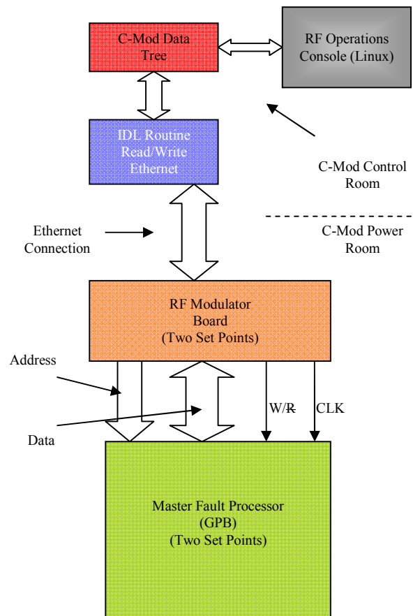
Figure 2. Data Flow Remote Ethernet Connection
