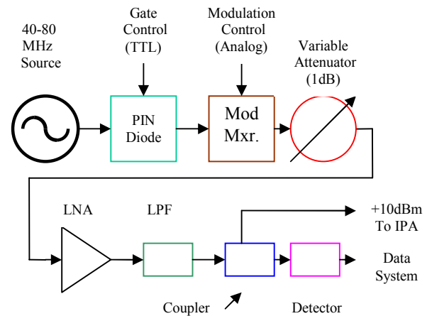
Figure 3. New Low Power Chain For Tunable Transmitters
