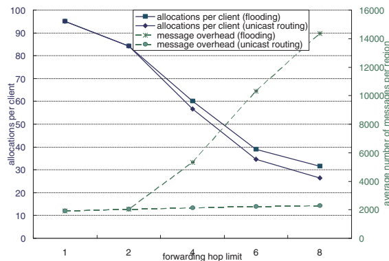
Fig. 4. Allocation performance with different renewal methods, fast moving case
