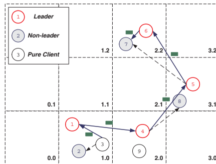
Fig. 1. Illustration of a virtual node system. A message from a pure client node 3 in region 1.0 is forwarded to a non-leader node 7 in region 2.2 through leader node 1,4,5 and 6. Non-leader node 2,7 and 8 work as backup routers.
