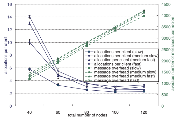
Fig. 8. Allocation performance with different node densities
