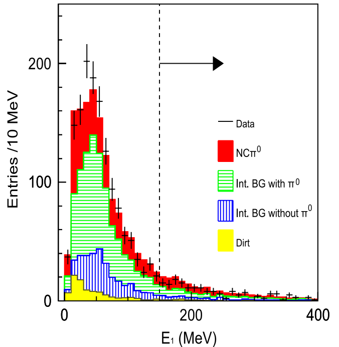
FIG. 7 (color online). Option 2 of the EC cut: the energy deposited in the upstream layer of the EC ( E_1 ) after the track disconnection cut. Events with E_1 > 150 \text{ MeV} pass the EC cut. Events with E_1 < 150 \text{ MeV} can pass the EC cut if they satisfy the requirement shown in Fig. 8.
