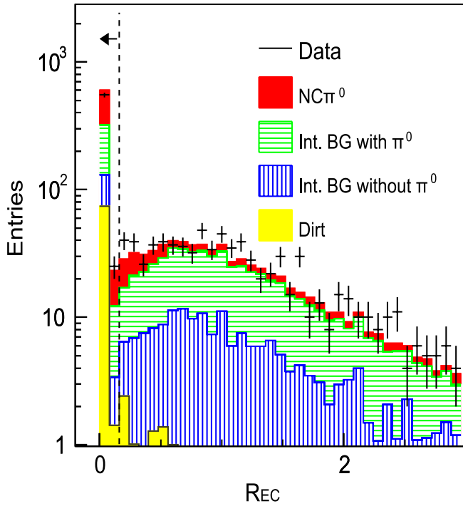
FIG. 8 (color online). Option 3 of the EC cut: the ratio of deposited energy in the downstream over the upstream layer ( R ) after the track disconnection cut. Only events with E_1 < 150 MeV are shown.
