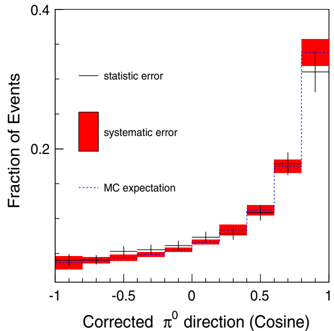
FIG. 22 (color online). The \pi^0 angular distribution after all corrections described in the text, with statistical (error bars) and systematic (red boxes) uncertainties. The dashed line shows the Monte Carlo expectation based on the Rein and Sehgal model.
