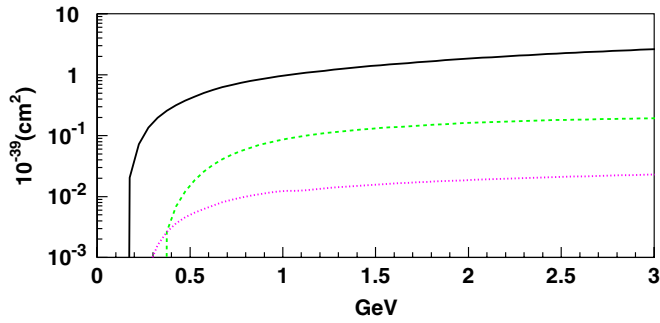
FIG. 3 (color online). Cross sections versus neutrino energy of the total CC interaction (solid line), the NC single \pi^0 production via baryon resonances (dashed line), and the NC coherent \pi^0 production (dotted line) calculated in NEUT per nucleon on polystyrene target.
