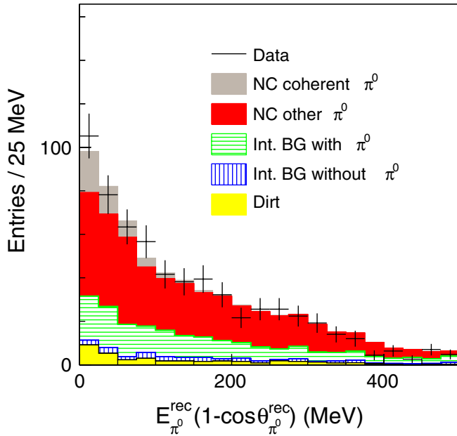
FIG. 23 (color online). E_{\pi^0}^{\text{rec}}(1 - \cos\theta^{\text{rec}}) after fitting. The coherent contribution and other NC \pi^0 are separately shown for the MC simulation.
