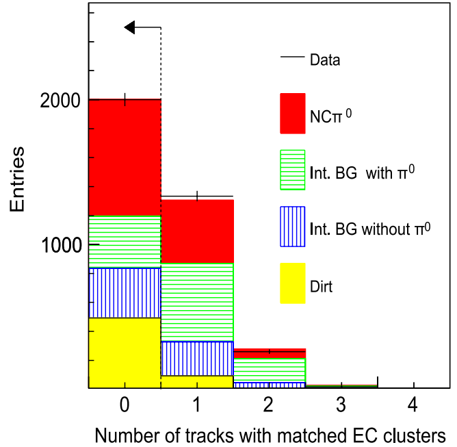
FIG. 6 (color online). Option 1 of the EC cut: the number of track with matched EC clusters after the track disconnection cut. Events without SciBar-EC matched tracks pass the EC cut. Events with SciBar tracks matching EC clusters can pass the EC cut if they satisfy the requirement shown in Fig. 7 or Fig. 8.
