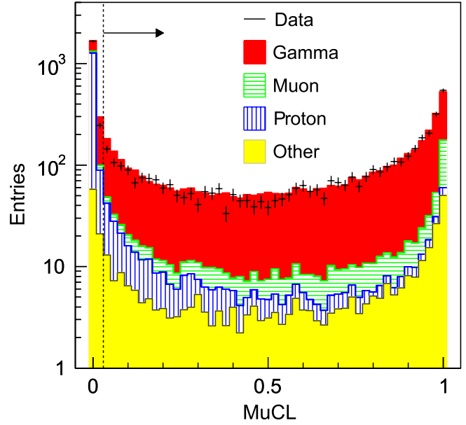
FIG. 9 (color online). The MuCL of tracks after the EC cut. The contributions from true gamma ray, muon, and proton tracks are shown separately for the MC simulation.
