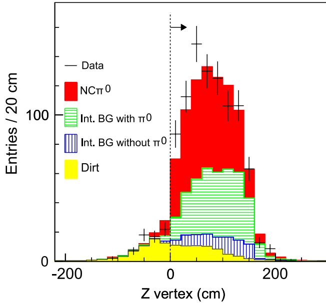
FIG. 11 (color online). The reconstructed z vertices of \pi^0 s after the requirement of at least two extended tracks.
