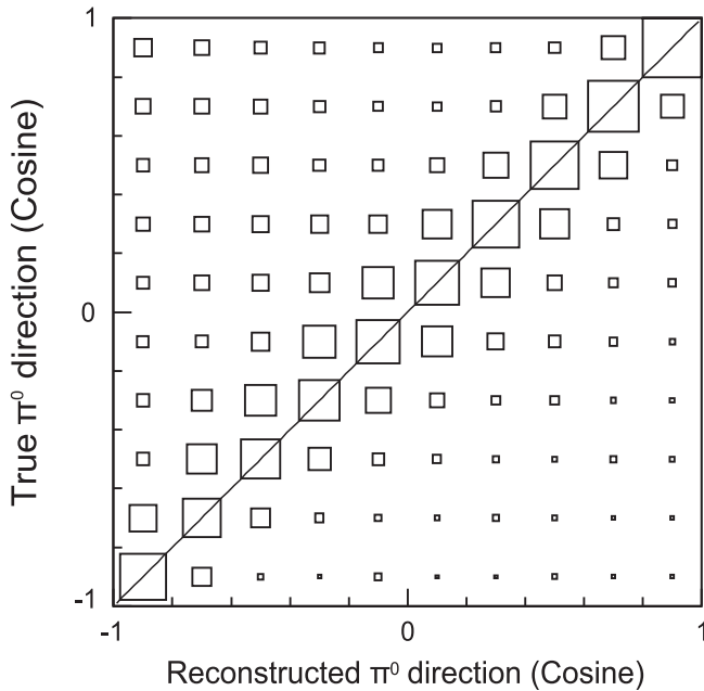
FIG. 20. The true \pi^0 direction ( \cos\theta^{\text{true}} ) versus reconstructed \pi^0 direction ( \cos\theta^{\text{rec}} ) from the MC simulation. The solid line shows the identity.
