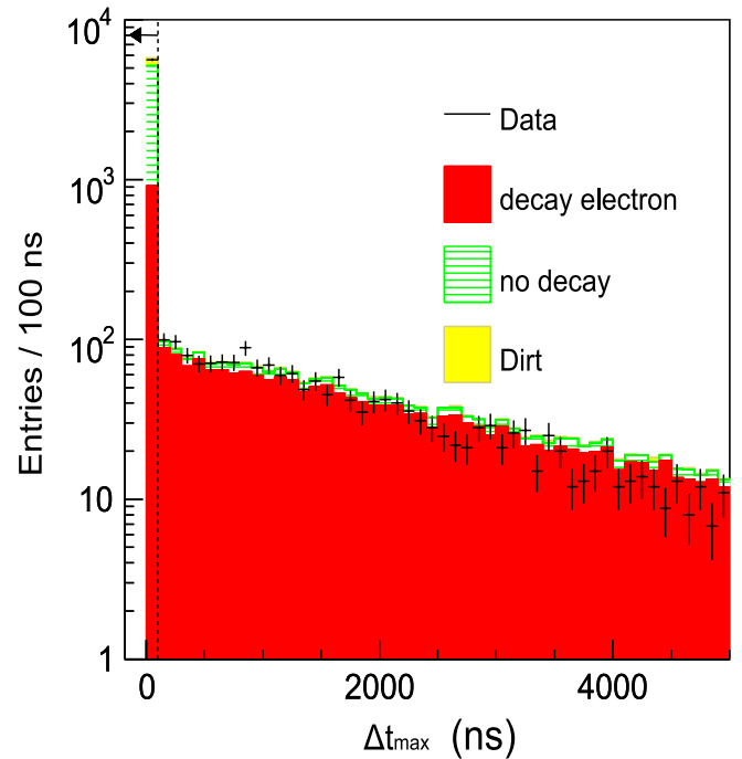
FIG. 4 (color online). \Delta t_{\text{max}} distribution (IV D 2) after rejection of side escaping tracks. The contributions from events with decay electrons, events without decay electrons and the dirt events are shown separately for the MC simulation.
