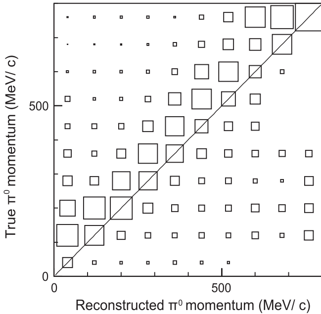
FIG. 19. The true \pi^0 momentum ( P^{\text{true}} ) versus reconstructed \pi^0 momentum ( P^{\text{rec}} ) from the MC simulation. The solid line shows the identity.
