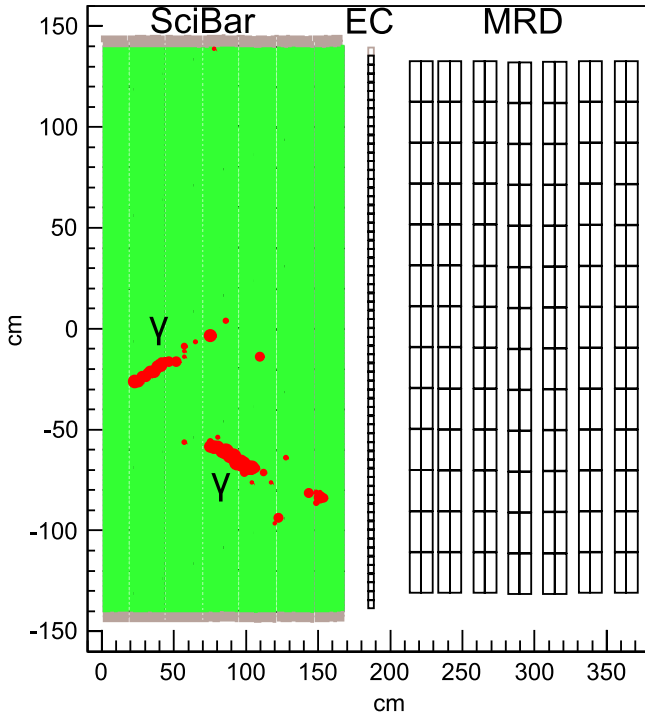
FIG. 1 (color online). Event display of a typical NC\pi^0 event candidate in SciBooNE data. The neutrino beam runs from left to right in this figure, encountering SciBar, the EC, and MRD, in that order. The circles on SciBar indicate analog-to-digital converter hits for which the area of the circle is proportional to the energy deposition in that channel. This event display shows the electromagnetic shower tracks from the pair conversions of the two \pi^0 decay photons.
