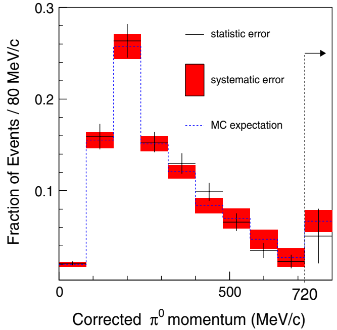
FIG. 21 (color online). The \pi^0 momentum distribution after all corrections described in the text, with statistical (error bars) and systematic (red boxes) uncertainties. The dashed line shows the Monte Carlo expectation based on the Rein and Sehgal model.
