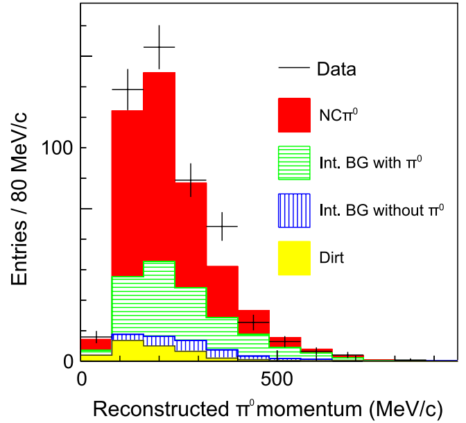
FIG. 15 (color online). The reconstructed \pi^0 momentum after all event selection cuts.
