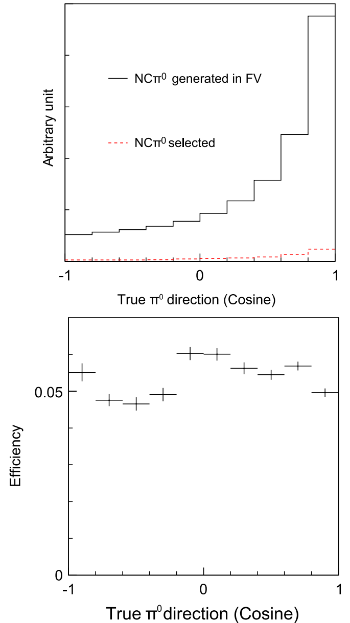
FIG. 18 (color online). The true \pi^0 angle with respect to the beam direction for generated MC events (solid) and selected MC events (dashed) for NC \pi^0 production (top), and the efficiency for NC \pi^0 production as a function of the true \pi^0 direction (bottom).
