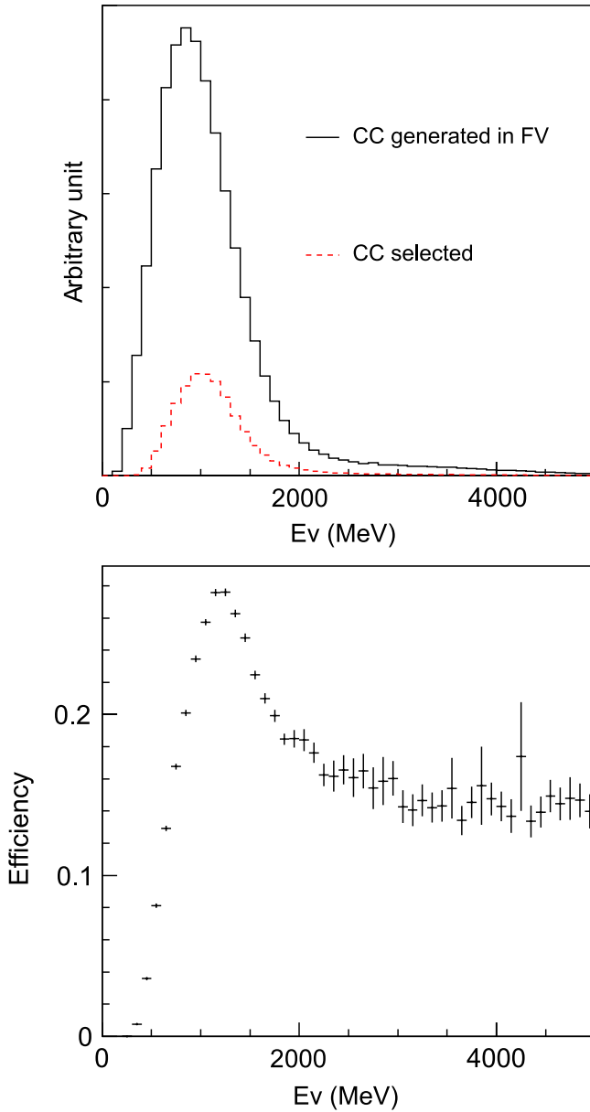
FIG. 14 (color online). Expected neutrino energy spectra and selection efficiency as a function of neutrino energy for all CC events.
