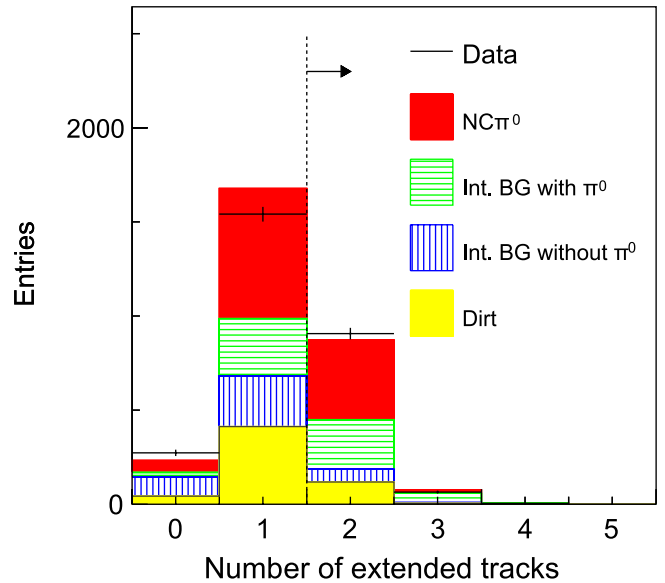
FIG. 10 (color online). The distribution of the number of extended tracks after the EC cut.
