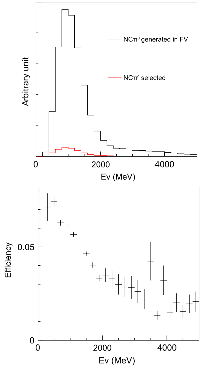
FIG. 13 (color online). Expected neutrino energy spectra and selection efficiency as a function of neutrino energy for \text{NC}\pi^0 events.
