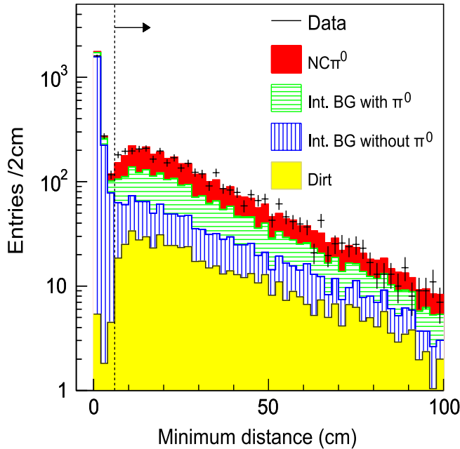
FIG. 5 (color online). The minimum distance between two tracks after muon rejection cuts. The contribution from \text{NC}\pi^0 production, internal backgrounds with a \pi^0 in the final state, internal background without a \pi^0 in the final state and “dirt” background events are shown separately for the MC simulation.
