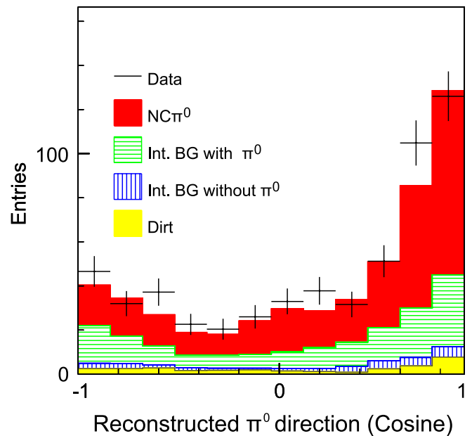
FIG. 16 (color online). Cosine of the reconstructed \pi^0 angle with respect to the beam direction after all event selection cuts.
