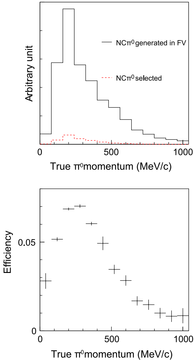
FIG. 17 (color online). The true \pi^0 momentum of generated MC events (solid) and selected MC events (dashed) for all NC \pi^0 production processes (top), and the true \pi^0 momentum dependence of the efficiency of NC \pi^0 production (bottom).
