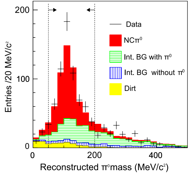
FIG. 12 (color online). The reconstructed mass of \pi^0 s after the reconstructed vertex position cut.
