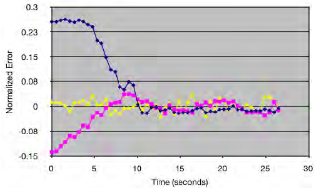
Fig. 6. Sample trajectory describing the Cartesian error of the robot's end-effector from its initial position to a successful grasp.
