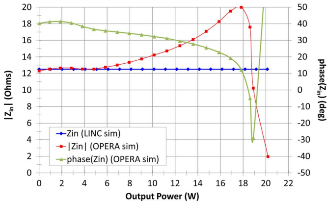
Fig. 14. Simulated isolation port impedance versus output power in the OPERA prototype. The desired isolation port impedance is also shown for reference.
