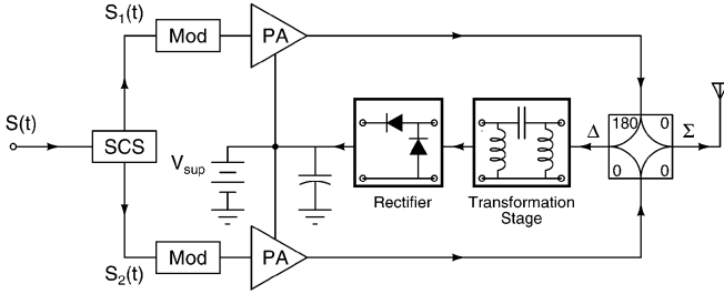
Fig. 2. Outphasing power amplifier with power recycling network.
