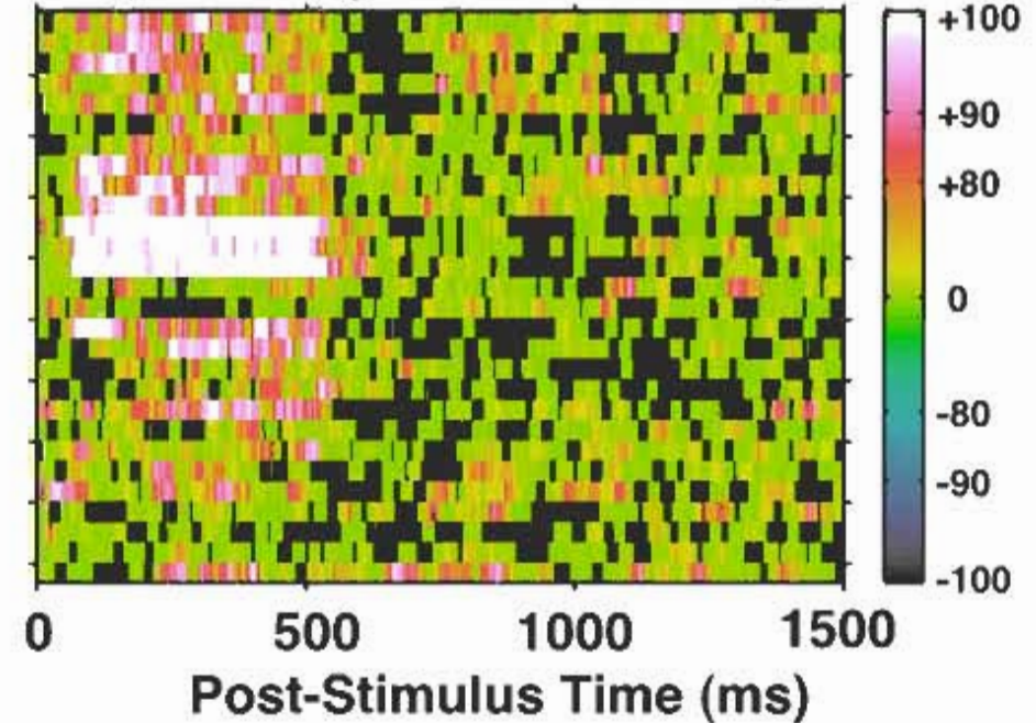
D Response significance re: bkgr
