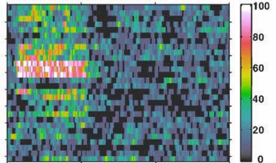
D Response significance re: bkgr
