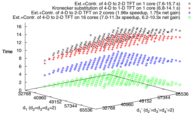
Figure 6. 4-variate multiplication timing (s) via balanced multiplication on 1, 2, 16 cores vs Kronecker substitution to 1-D TFFT.
