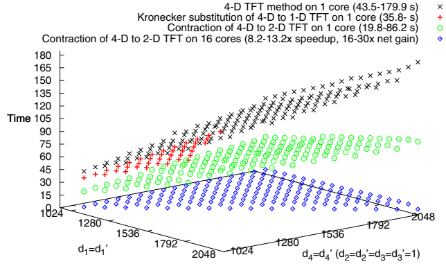
Figure 4. Timing (s) for 4-variate multiplication by direct 4-D TFT on 1 core vs Kronecker’s substitution on 1 core vs contraction from 4-D to 2-D TFT on 1 core and 16 cores.
