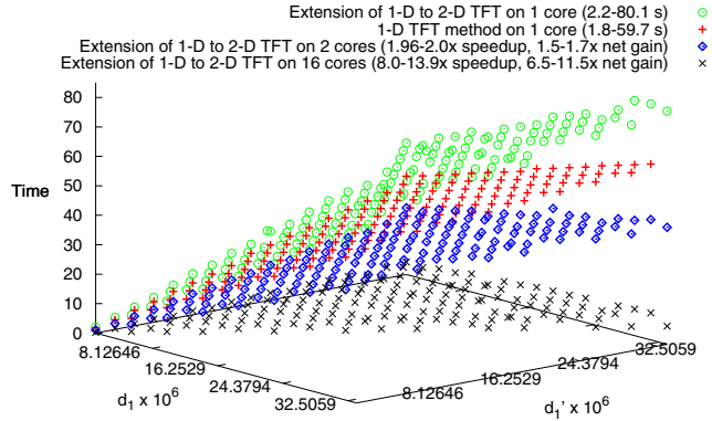
Figure 5. Univariate multiplication timing (s) via extension to 2-D TFT on 1, 8, 16 cores vs direct 1-D TFT.
