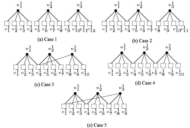
Fig. 1. All possible subgraphs subtended by three erroneous variable nodes.
