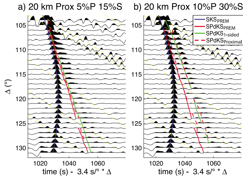
Figure 12. Synthetic seismograms for finite length, proximal ULVZ models (Figure 5f). The thickness of the ULVZ is 20 km, and the velocity perturbations are (a) 5\%V_p , 15\%V_s , and (b) 10\%V_p , 30\%V_s . Blue line shows SKS picks from PREM pseudospectral synthetic seismograms. Solid red line shows PREM SPdKS picks. Dashed red line shows SPdKS picks for this model. Note that although a partial split of the SPdKS is observed in Figure 12a, we do not delineate the second pulse because it is too close to the first pulse and thus is not preceded by a zero crossing (i.e., the reference point for phase picking). Green solid lines show SPdKS picks for equivalent one-sided ULVZ model. Yellow dashed lines indicate predicted arrival times for sPPP , PPPP , pPPP , and other multiple P arrivals (see Figure 3).
