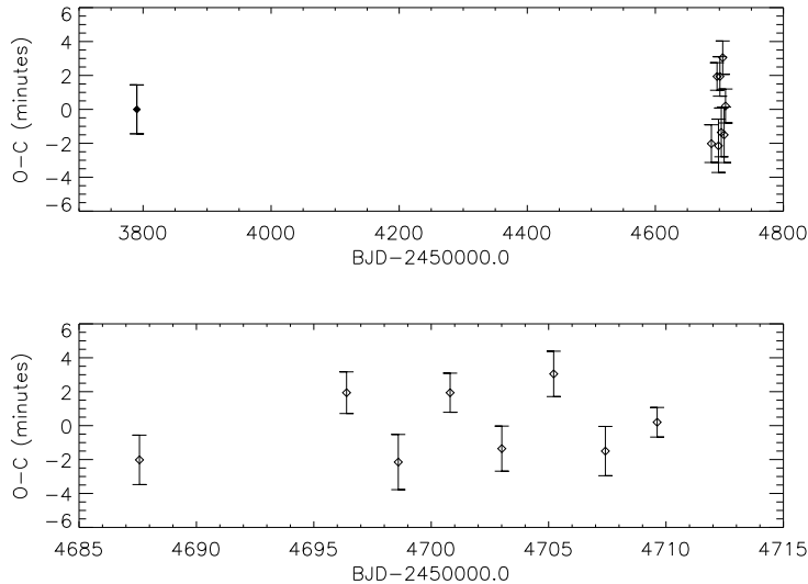
Fig. 3.— Observed transit times of HAT-P-7b minus the best fit linear ephemeris. Upper panel: The solid data point is from Pál et al. (2008), the hollow points are the EPOXI transit times. Lower panel: An expanded view of the EPOXI transit times.
