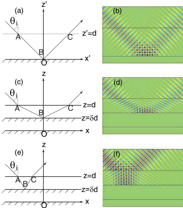
FIG. 2 (color online). Left column: Ray tracing diagrams of a ray with incident angle of \theta_i . Right column: A Gaussian beam with incident angle of \theta_i . (a),(b) A PEC ground plane in free space with no cloak. (c),(d) A perfect anisotropic cloak squeezing space between z = 0 and z = d into space between z = \delta d and z = d . (e),(f) Replace the anisotropic cloak with isotropic medium. In the illustration, \delta = 0.5 and \theta_i = 45^\circ .
