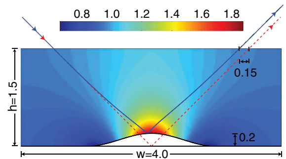
FIG. 4 (color online). A ray (blue solid line) incident at 45^\circ to the normal onto an isotropic ground-plane cloak. The bump has a maximum height of 0.2 units [5]. The red dotted line represents the trajectory of an undistorted ray in the absence of the cloak and the bump. The background represents n^2 . Notice the distorted ray has been shifted on top of the cloak toward the incident point by 0.15 units.
