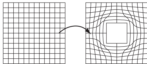
FIG. 1. An example of creating an invisibility cloak by coordinate transformation. In general the transformation is not a conformal mapping and the transformed cloak is anisotropic.
