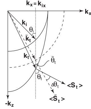
FIG. 3. k vectors used in phase matching between the incident and cloak media. The solid circle represents the incident medium and the solid ellipse represents the cloak medium. The dotted circle represents the isotropic medium that replaces the cloak medium.
