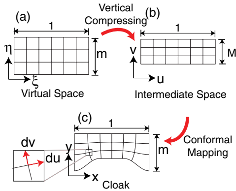
FIG. 5 (color online). Procedure of quasiconformal mapping. (a) A rectangle of 1 \times m in virtual free space. (b) Compressed rectangle of 1 \times M in the intermediate space. (c) An anisotropic cloak created from quasiconformal mapping.
