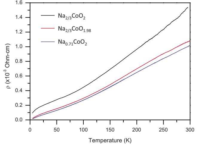
FIG. 4. (Color online) In-plane resistivities for \text{Na}_{0.71}\text{CoO}_2 , \text{Na}_{2/3}\text{CoO}_2 , and \text{Na}_{2/3}\text{CoO}_{1.98} .
