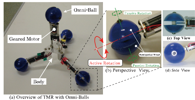
Fig. 2: First Prototype of Tetrahedral Mobile Robot [16] could be used for this robot, but the mobility on a rough terrain is important elements of the field, therefore we adopted this mechanism for a tetrahedral robot. This configuration can protect its own body and prevent taking damages from outsides.
