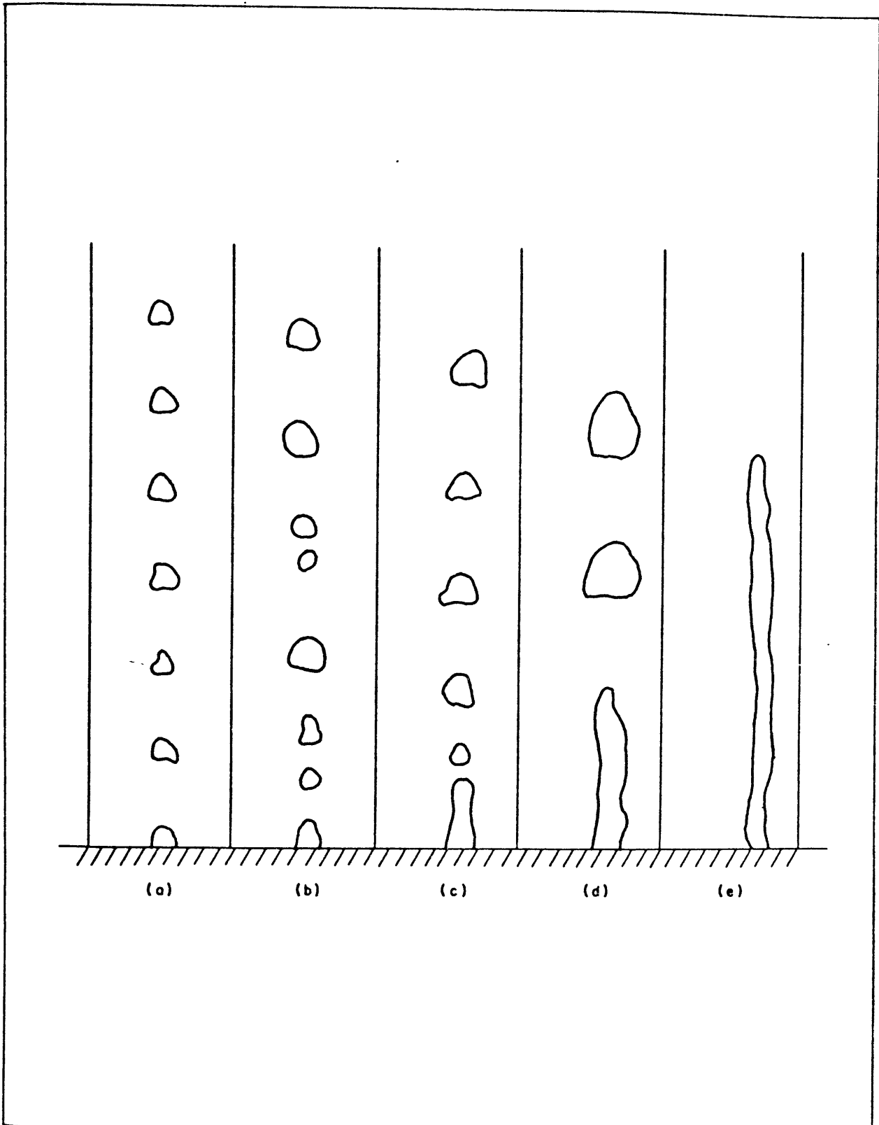
Fig. 19 - Stages in the Transition from the Region of Isolated Bubbles to the Region of Continuous Vapor Columns (vapors flow increasing from a to e) [ 22 ]
