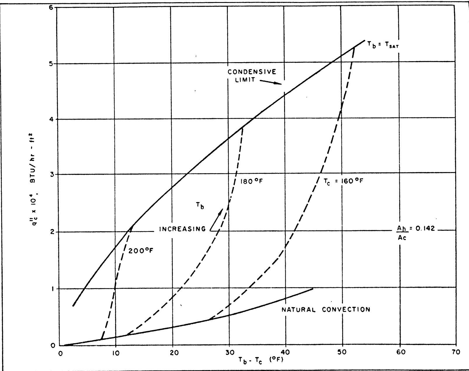
Fig. 33 - Bulk Temperature Variation with Condenser Heat Flux - Water
