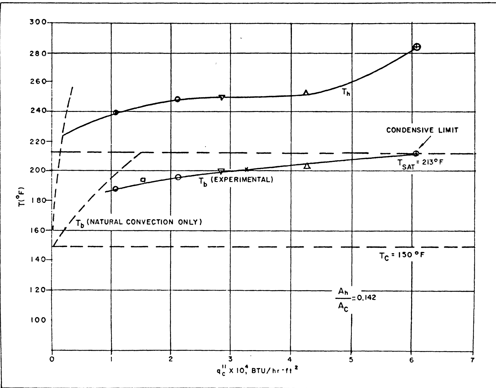
Fig. 13 - Bulk and Heated Surface Temperature Variation with Condenser Heat Flux - Water, One Heater
