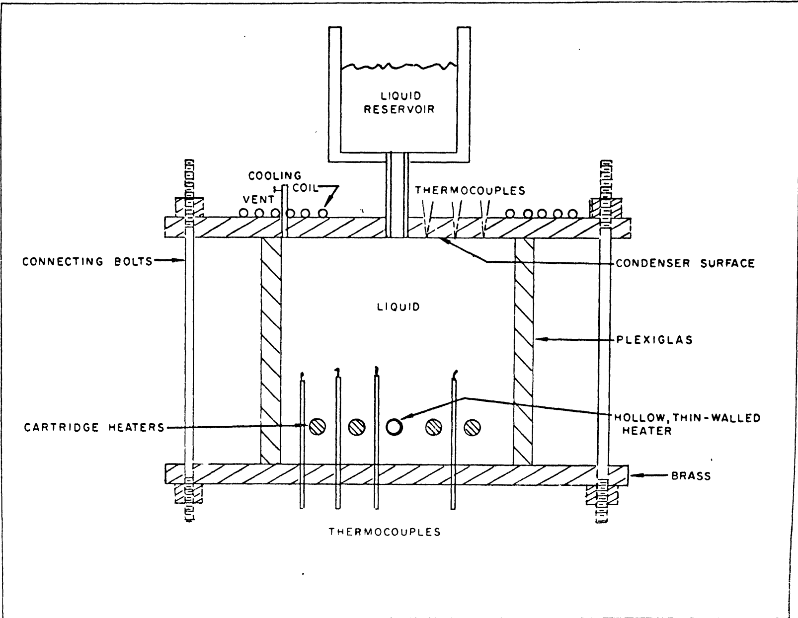
Fig. 5 - Schematic of Experimental Submerged Condenser Apparatus
