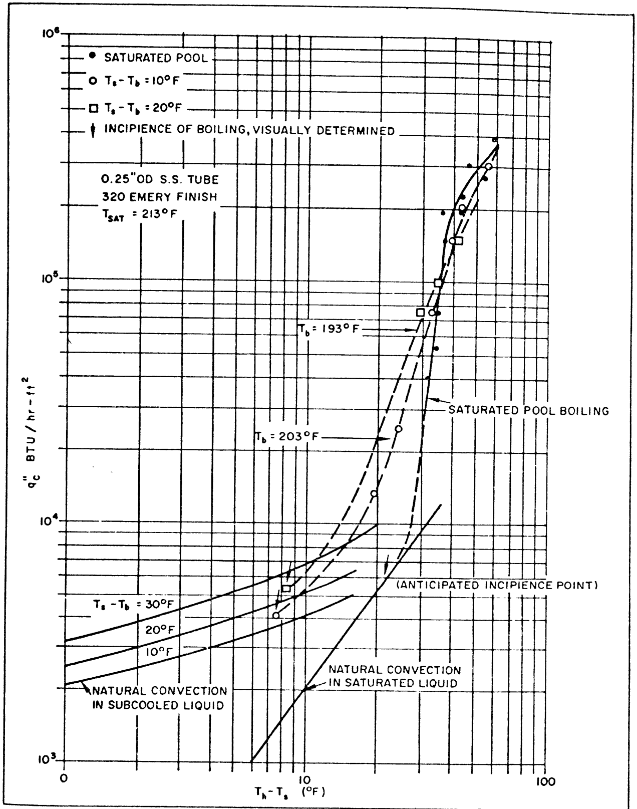
Fig. 18 - Pool Boiling of Water
