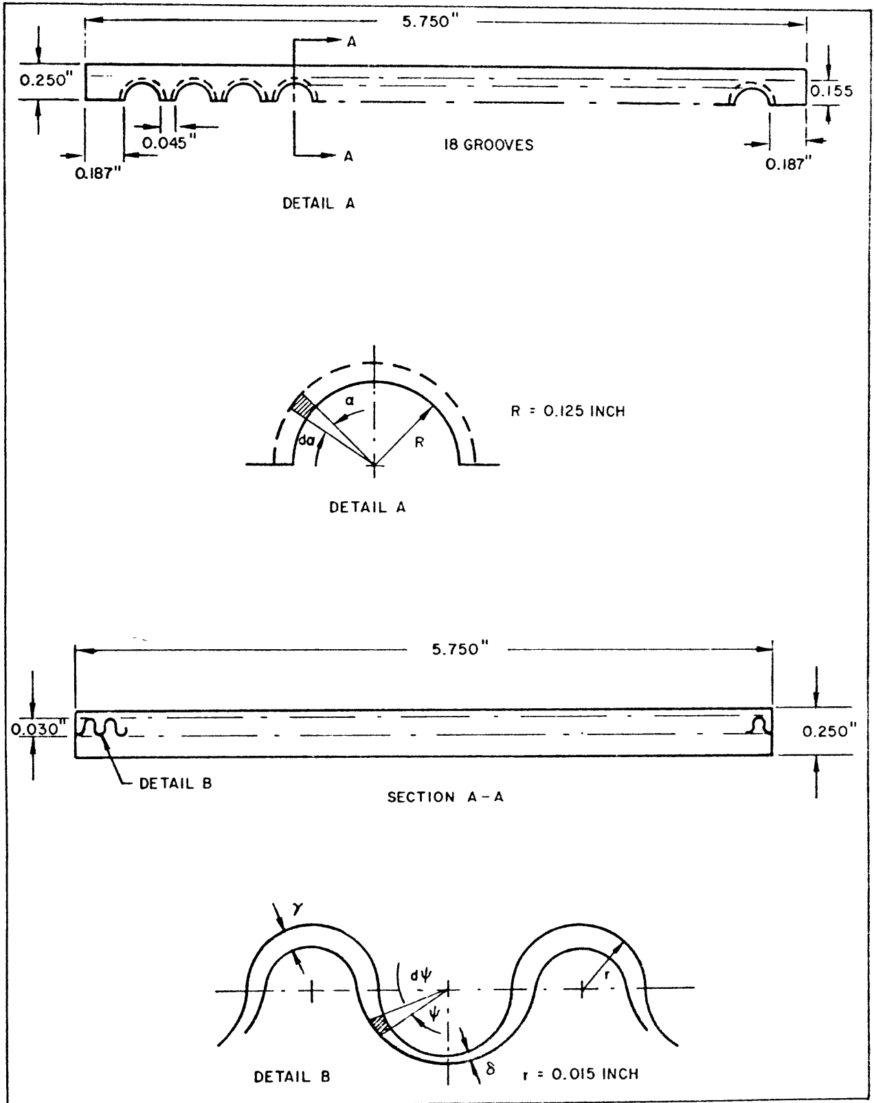
Fig. 29 - Schematic and Coordinate System for Doubly-Rippled Surface
