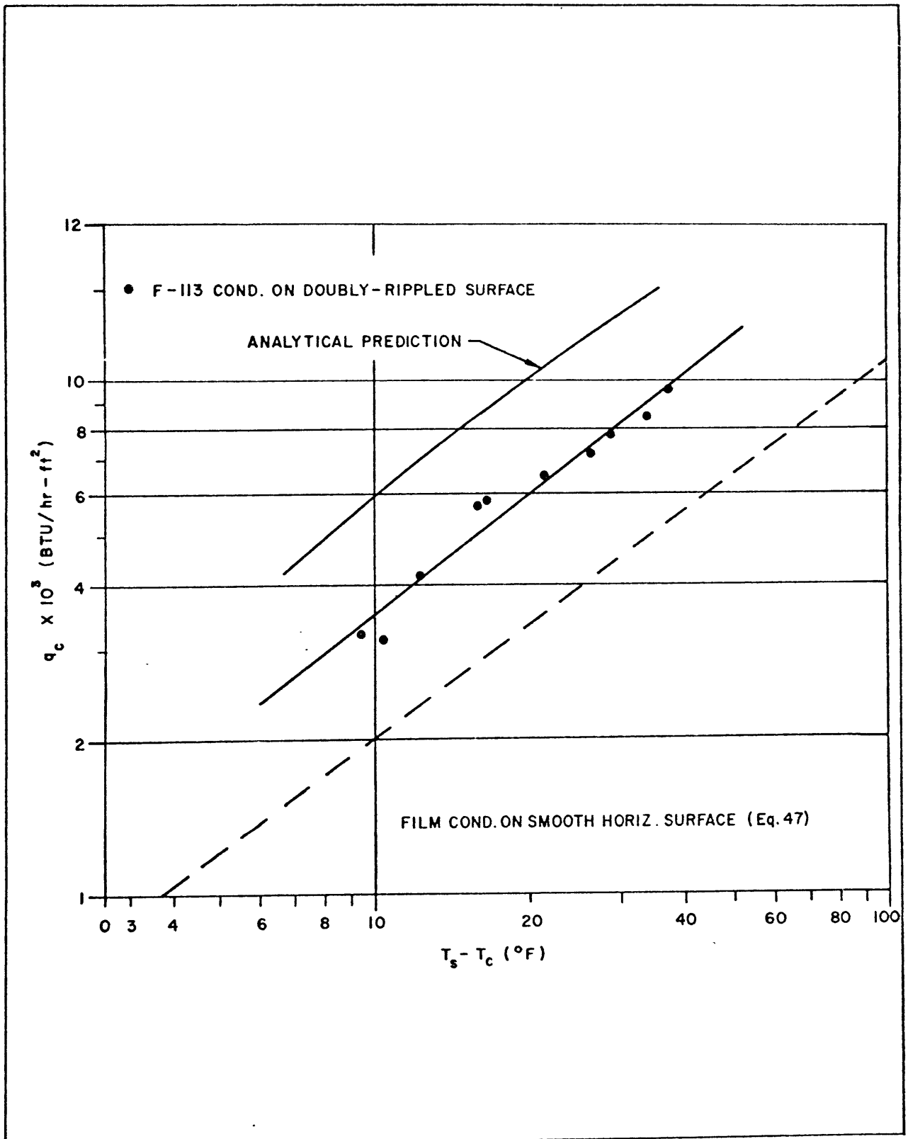
Fig. 32 - Condensive Limit for Doubly-Rippled Horizontal Condenser Surface
