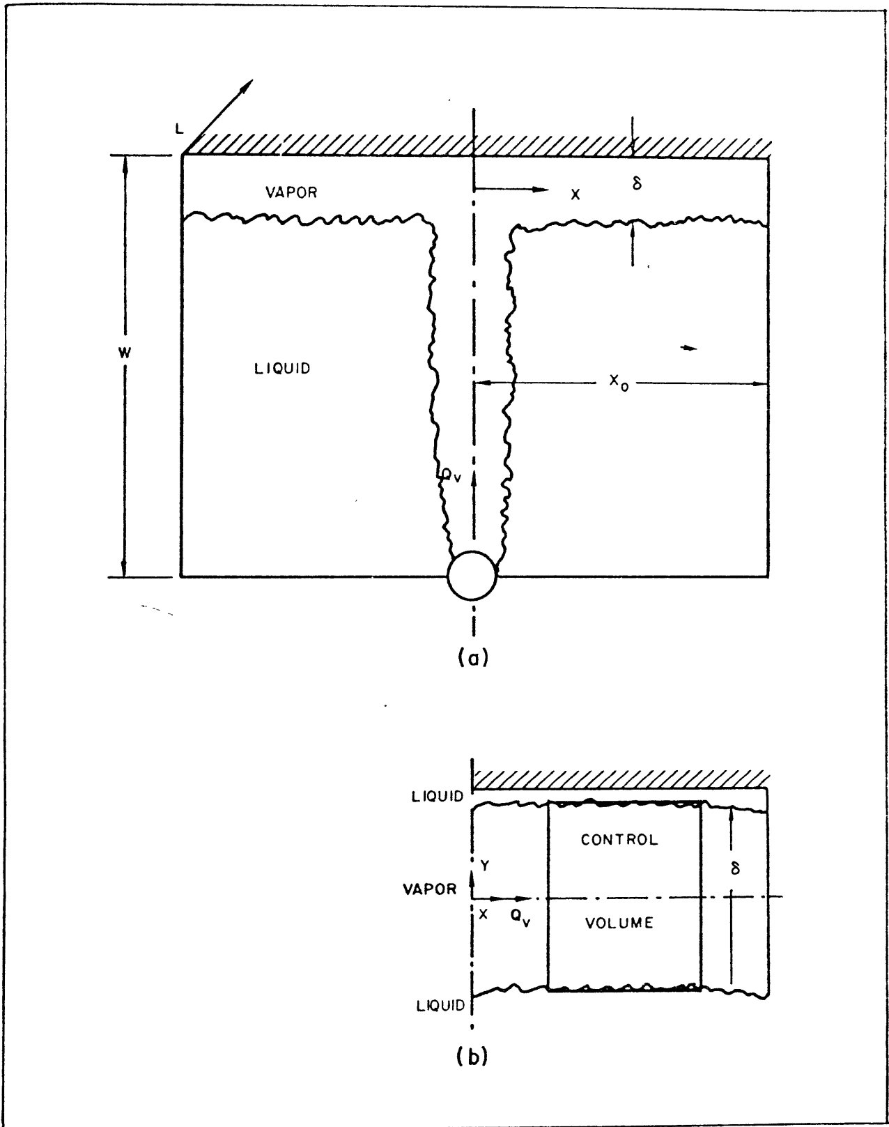
Fig. 25 - Model and Coordinate System for Vapor Gap Analysis
