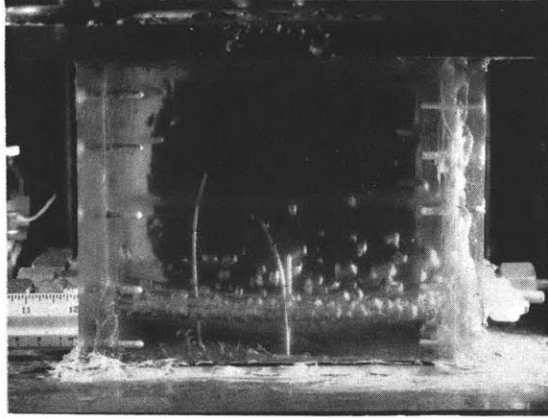
11a: SUBMERGED CONDENSER OPERATING MODE II \alpha - WATER, ONE HEATER ( q_c'' = 1.4 \times 10^4 , T_b = 206 )
