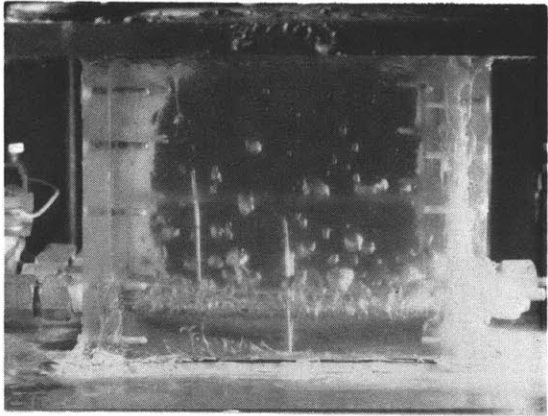
11b: SUBMERGED CONDENSER OPERATING MODE II \alpha - WATER, ONE HEATER ( q_c'' = 1.4 \times 10^4 , T_b = 208 )
