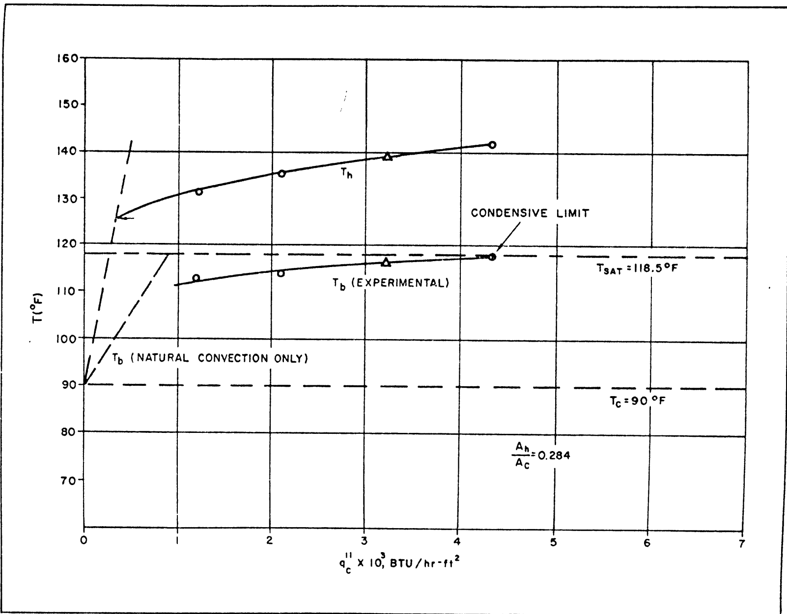
Fig. 16 - Bulk and Heated Surface Temperature Variation with Condenser Heat Flux - Freon-113, Two Heaters
