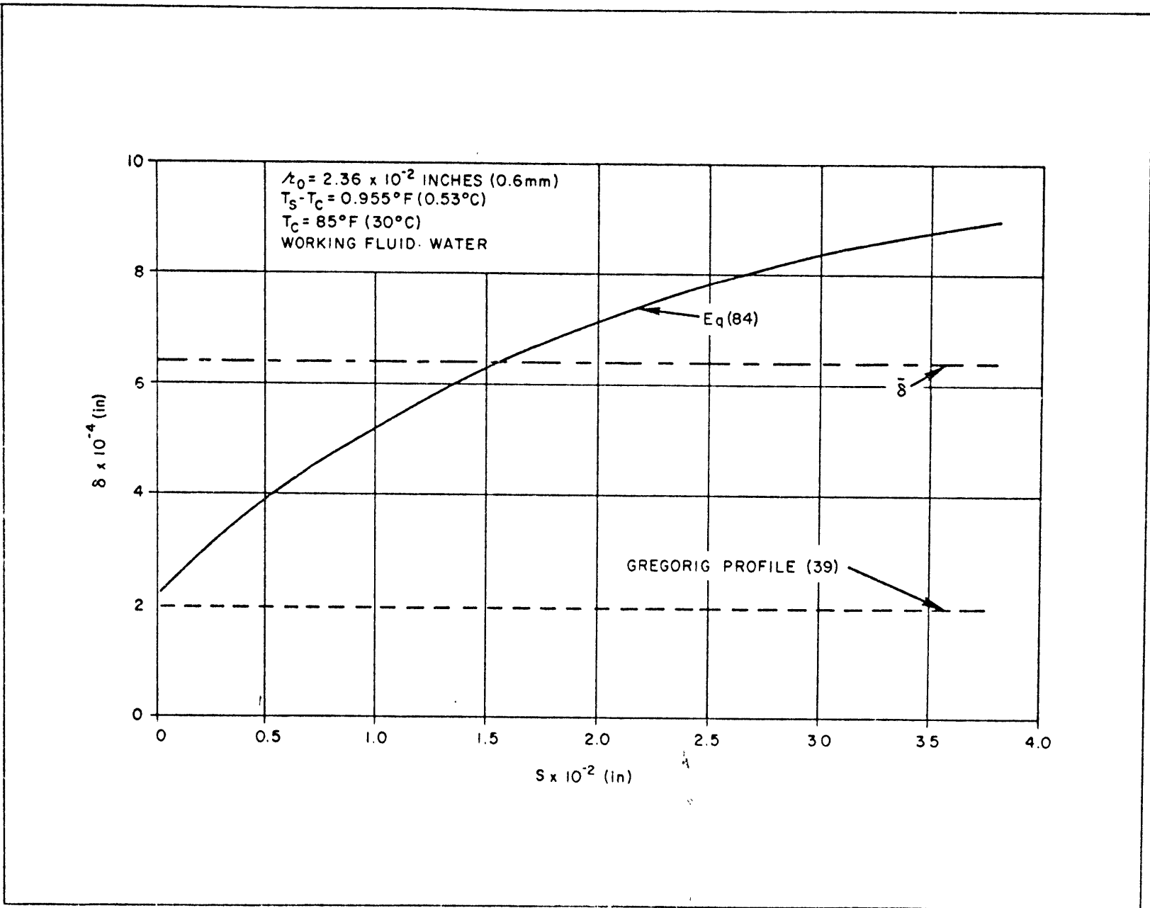
Fig. 31 - Condensate Film Thickness on Crest of Sinusoidal and Gregorig Type Profiles
