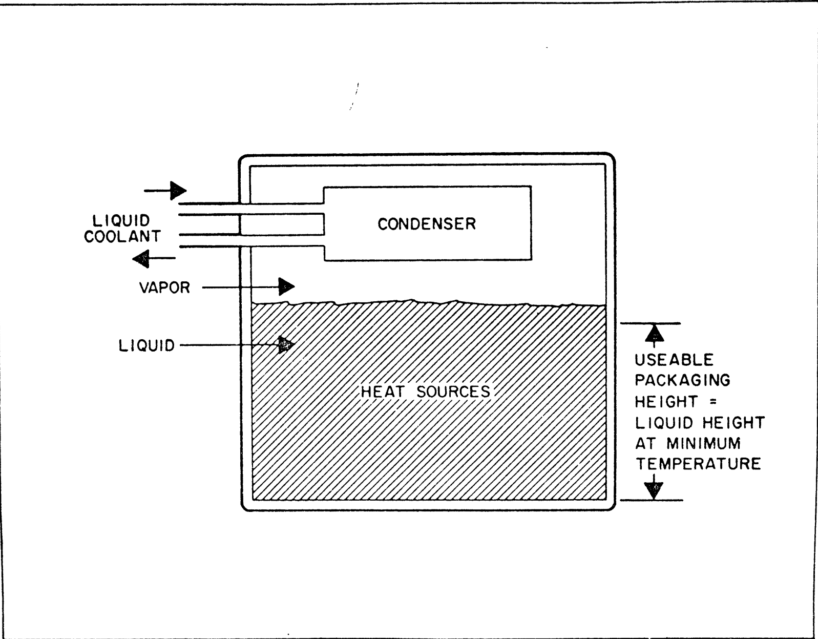
Fig. 1 - Pool Boiler for Electronic Components with Vapor Space Condenser (1)
