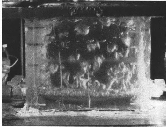
12a: SUBMERGED CONDENSER OPERATING MODE II b - WATER, ONE HEATER ( q_c = 1.4 \times 10^4 , T_b = 210.5 )
