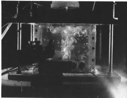
12b: SUBMERGED CONDENSER CONDENSATION LIMIT - WATER, ONE HEATER ( q_c = 1.4 \times 10^4 , T_b = 213 )
