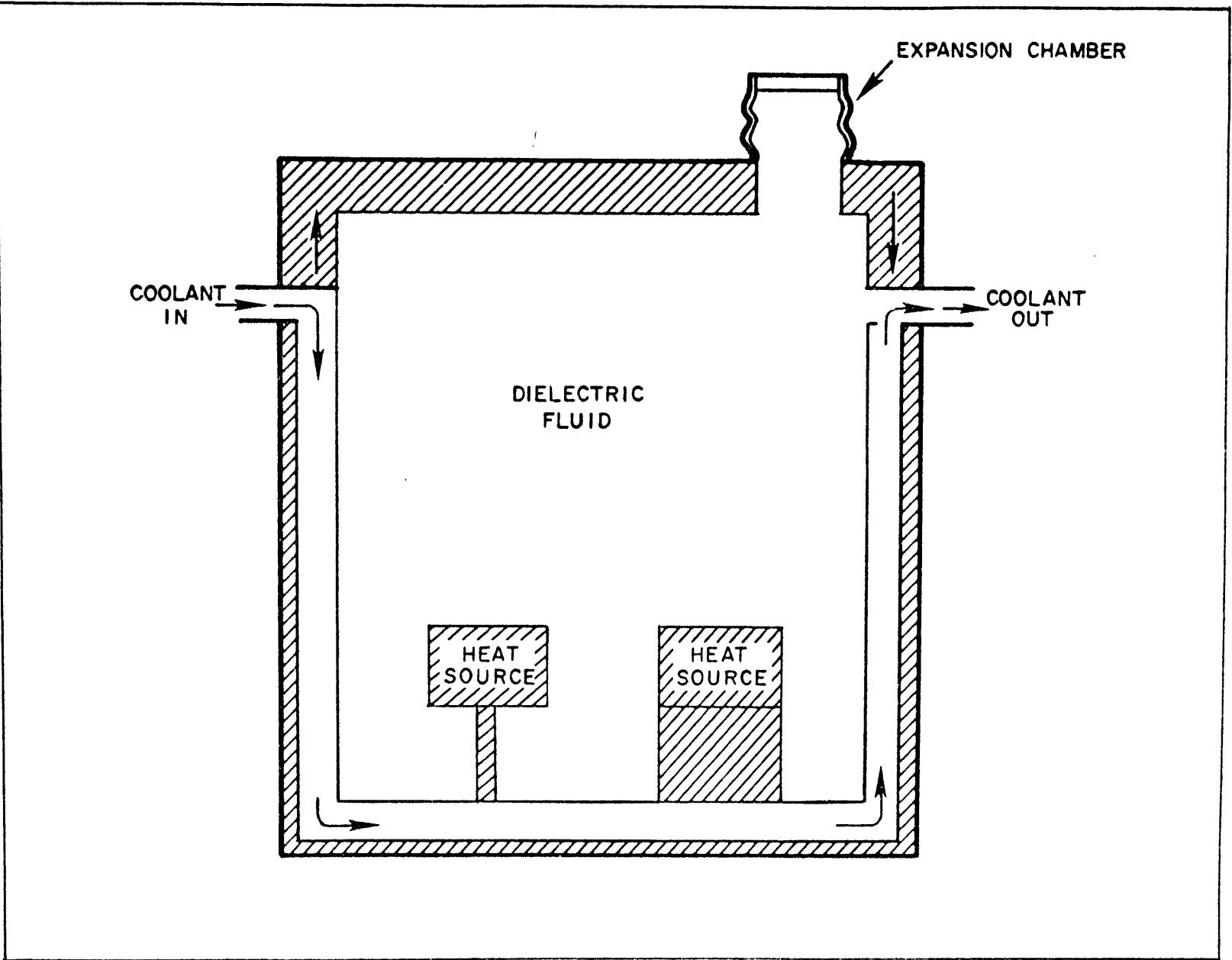
Fig. 3 - Pool Boiler for Electronic Components with Side Wall Cooling
