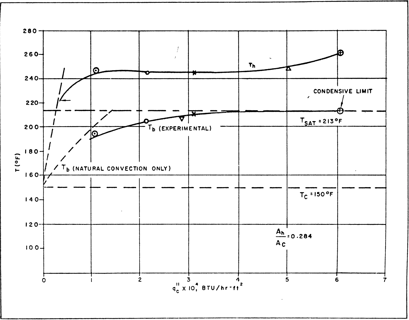
Fig. 14 - Bulk and Heated Surface Temperature Variation with Condenser Heat Flux - Water, Two Heaters 23
