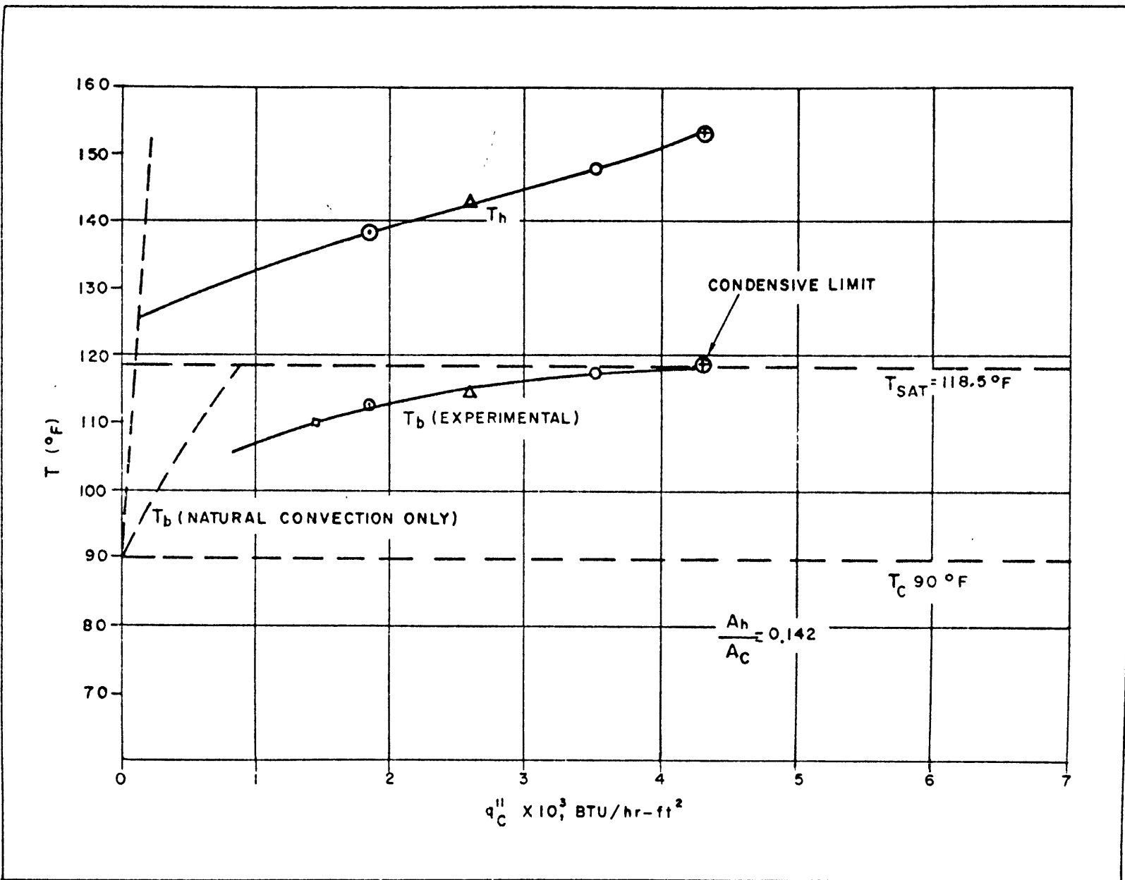
Fig. 15 - Bulk and Heated Surface Temperature Variation with Condenser Heat Flux - Freon-113, One Heater
