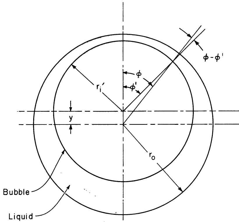
MODEL FOR BUBBLE RISE FIGURE A-1
