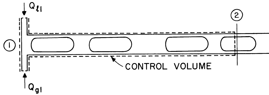
MODEL FOR CONTINUITY EQUATION
