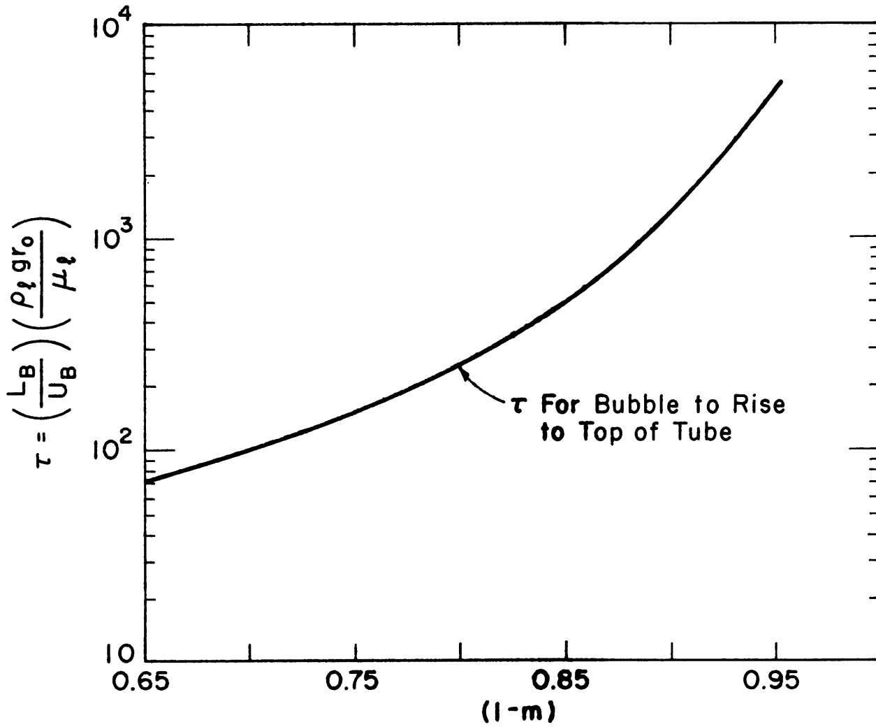
BUBBLE RISE TIME
