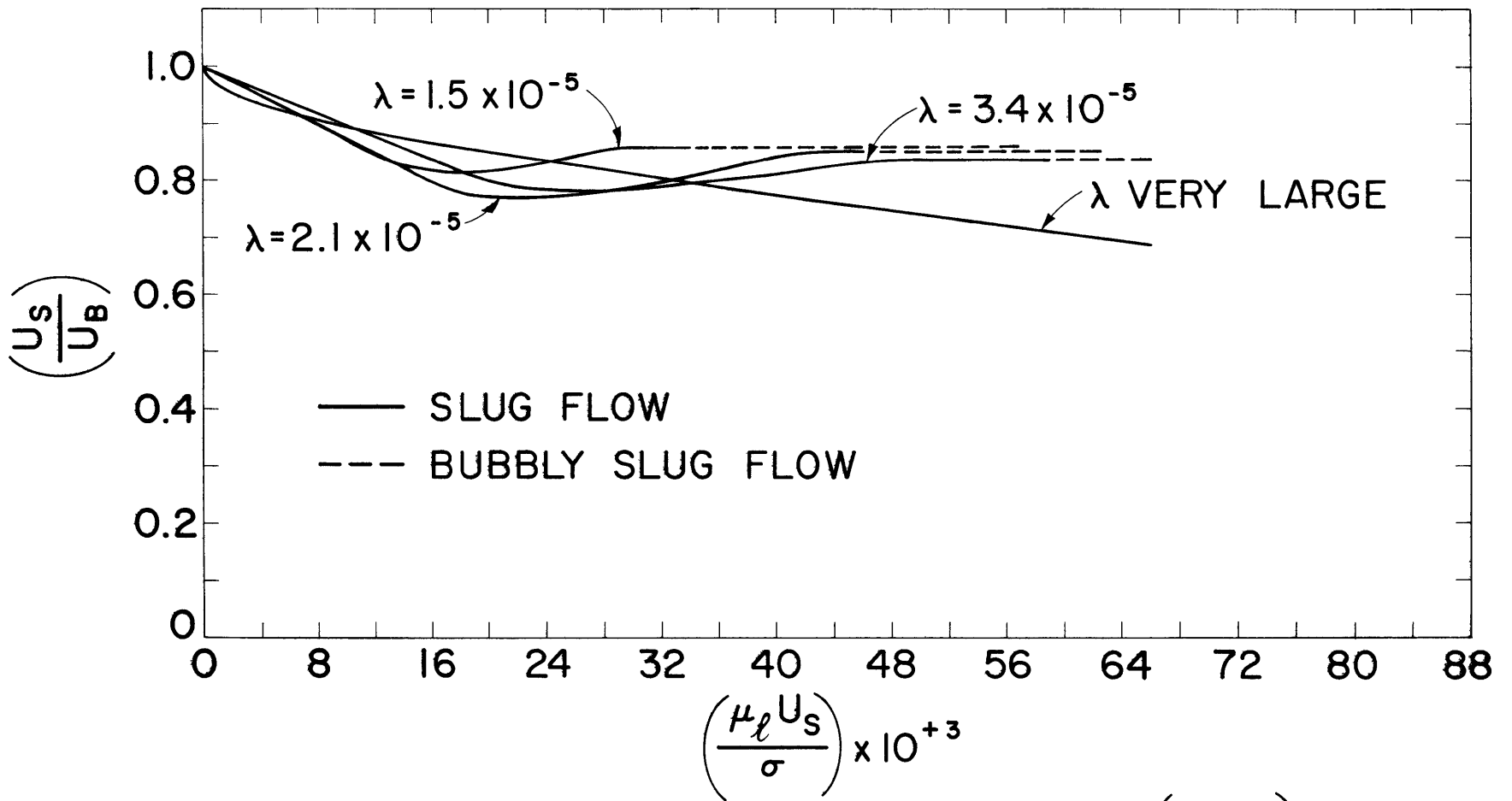
VELOCITY RATIO AS A FUNCTION OF \left(\frac{\mu_l U_s}{\sigma}\right) FIGURE 17
