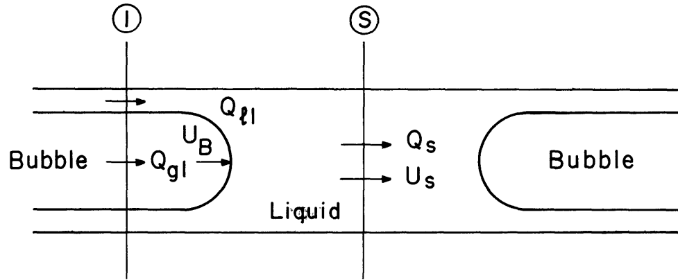
FLOW MODEL FOR FILM THICKNESS FIGURE C1
