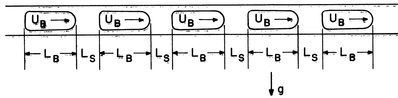
UNIFORM BUBBLE AND SLUG LENGTH MODEL OF CAPILLARY SLUG FLOW
