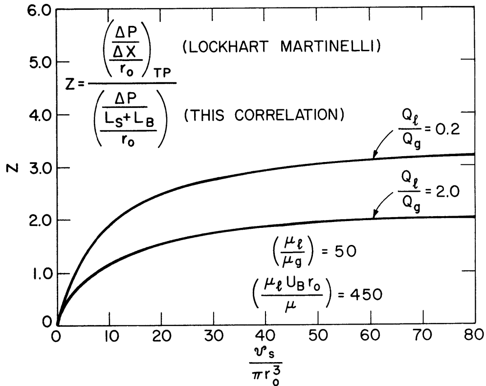
COMPARISON OF LOCKHART MARTINELLI PRESSURE-DROP TO THIS CORRELATION
