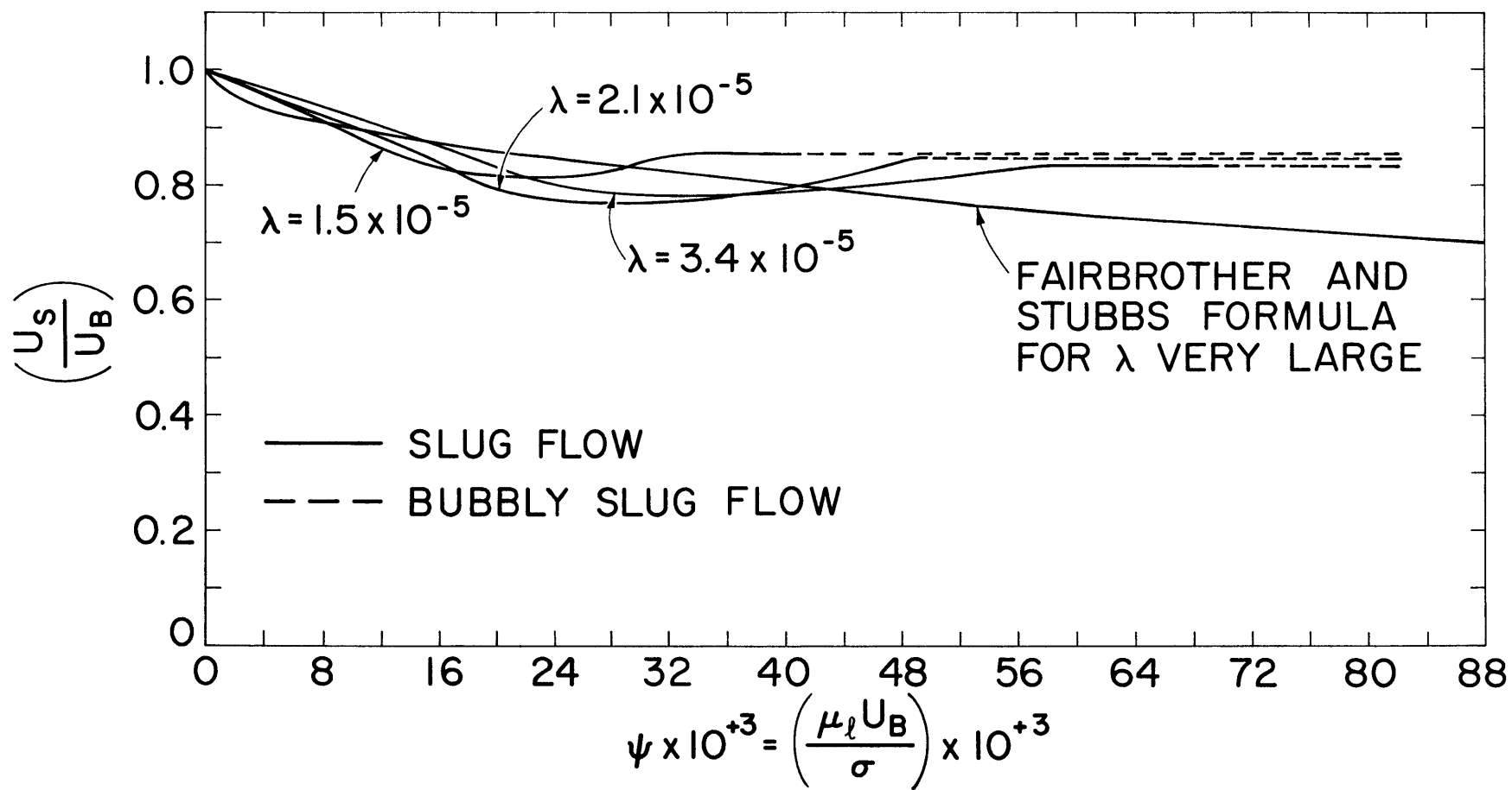
VELOCITY RATIO CORRELATION
