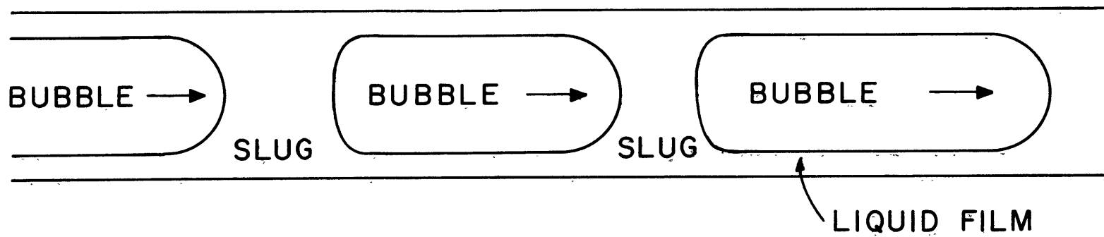
CAPILLARY SLUG FLOW
