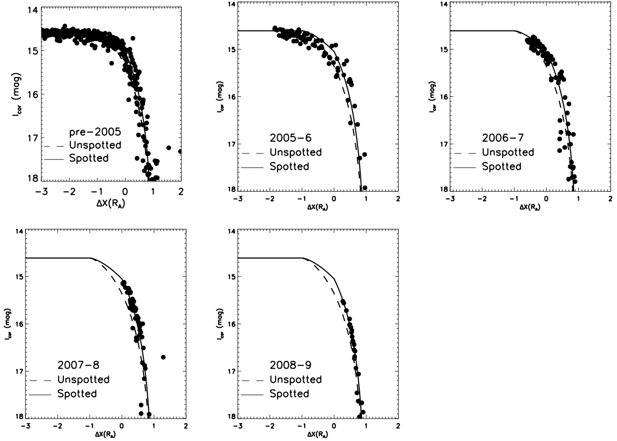
Fig. 11.— The pre-2005 data from Hamilton et al. (2005) and recent data, by observing season, from this paper are shown corrected for scattering as described in the text. It is clear that when allowance is made for the scattered light component, a slightly variable height in the occulting edge, and perhaps a spotted surface, the data fit the knife edge model very well.
