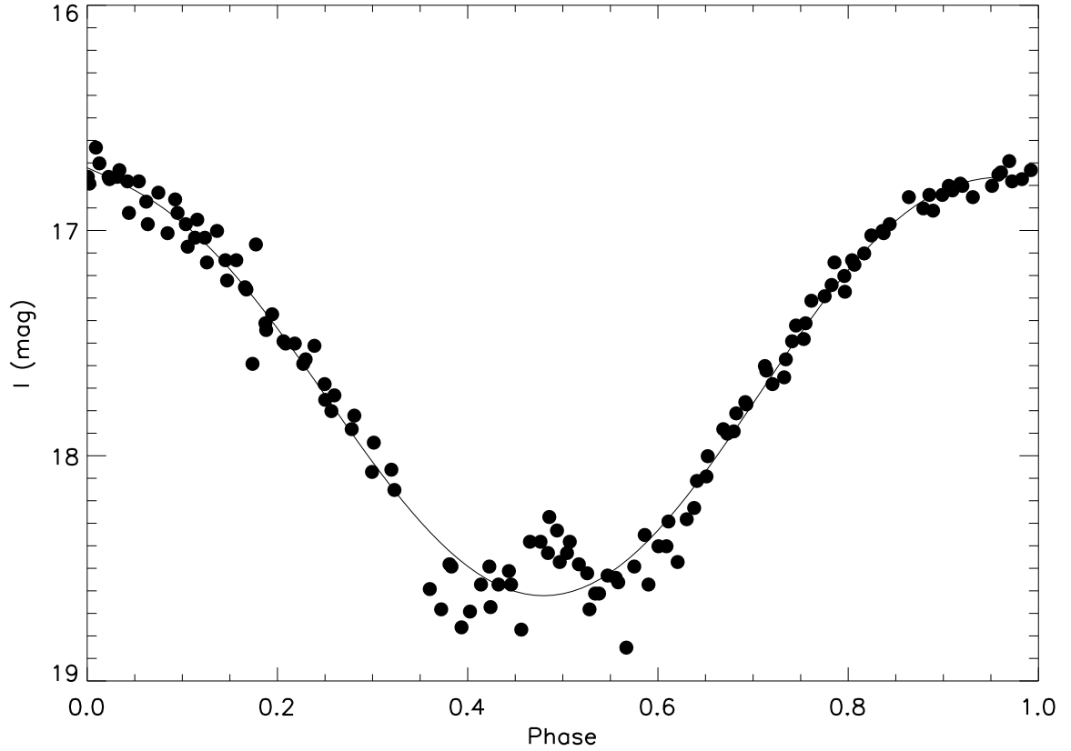
Fig. 7.— The 2009-10 data are plotted (solid circles), phased with the orbital period of 48.37 days. A sixth degree polynomial fit is shown (solid line) and was used to correct the total system light for the scattered light component. Note that the reversal of the decline near phase 0.5 is real and is caused by the rise of star B to a point where it is the dominant source of the reflected light received at Earth during those phases. This small reversal was not included in the fit to the data since it has no effect on the analysis done in this paper.
