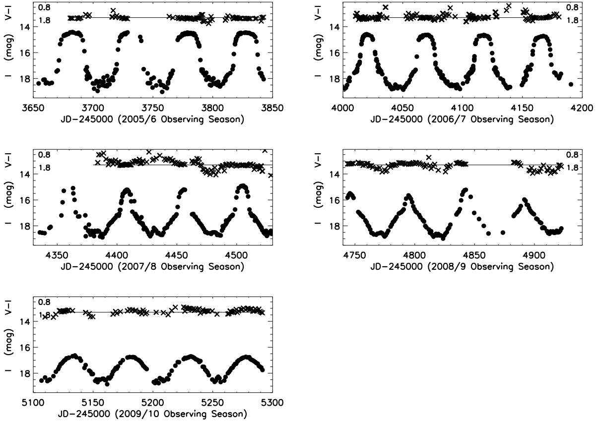
Fig. 3.— The measured I magnitude (solid circles) and V-I color (X's) of KH 15D over the five seasons 2005-6 to 2009-10. The solid line represents the out-of-eclipse mean color of V-I=1.575 . Bluer colors are towards the top of the figure. Only color data with errors less than 0.25 mag are plotted. Obviously the time spent near maximum brightness, when star A is not occulted at all, has continued to diminish such that by the 2009-10 observing season star A is fully occulted at all times. It is interesting that color changes are often seen near minimum light but they can be to the blue or to the red and are quite substantial.
