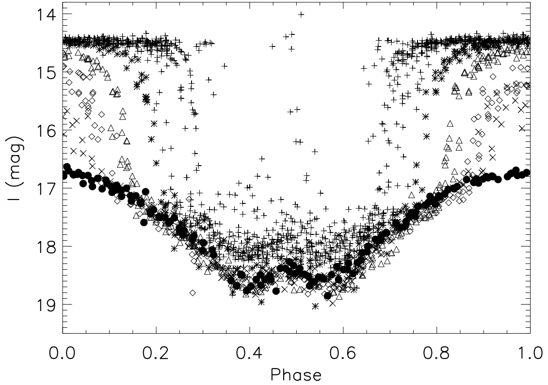
Fig. 4.— The KH 15D light curve phased with the period 48.37 days. Plus signs designate data obtained between 1995 and April of 2005. The new data reported here are plotted as asterisks (2005-6), triangles (2006-7), diamonds (2007-8) and X's (2008-9) and solid circles (2009-10). The light curves show a steady progress towards deeper and broader minima. The 2009-10 data generally define the faint boundary of the light curve and represent the scattered light component of the system alone.
