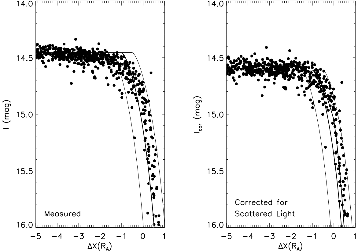
Fig. 8.— The left panel shows the pre-2005 data (Hamilton et al. 2005) plotted versus \Delta X , the distance of the center of star A from the occulting edge in units of the stellar radius based on the model of Winn et al. (2006). It is clear, as noted by Winn et al. (2006) and Silvia & Agol (2008), that there is an apparent decline in brightness of the system that occurs well before the point of “first contact” at \Delta X = -1 . When account is taken of the scattered light (by subtracting a fit to the 2009-10 light curve from all earlier data, as shown in Fig. 7), however, one obtains a light curve that has no such precursor (right panel). The solid lines on both panels show the expected light curve for a limb darkened star occulted by a knife edge of negligible thickness with no forward scattered light or halo. The limb darkening prescription of (Silvia & Agol 2008) has been adopted. Three lines are shown corresponding to \Delta X = (-0.5, 0, +0.5) allowing for some range in this quantity. A fourth line on the right hand panel (third line from left) represents the spot model described in the text.
