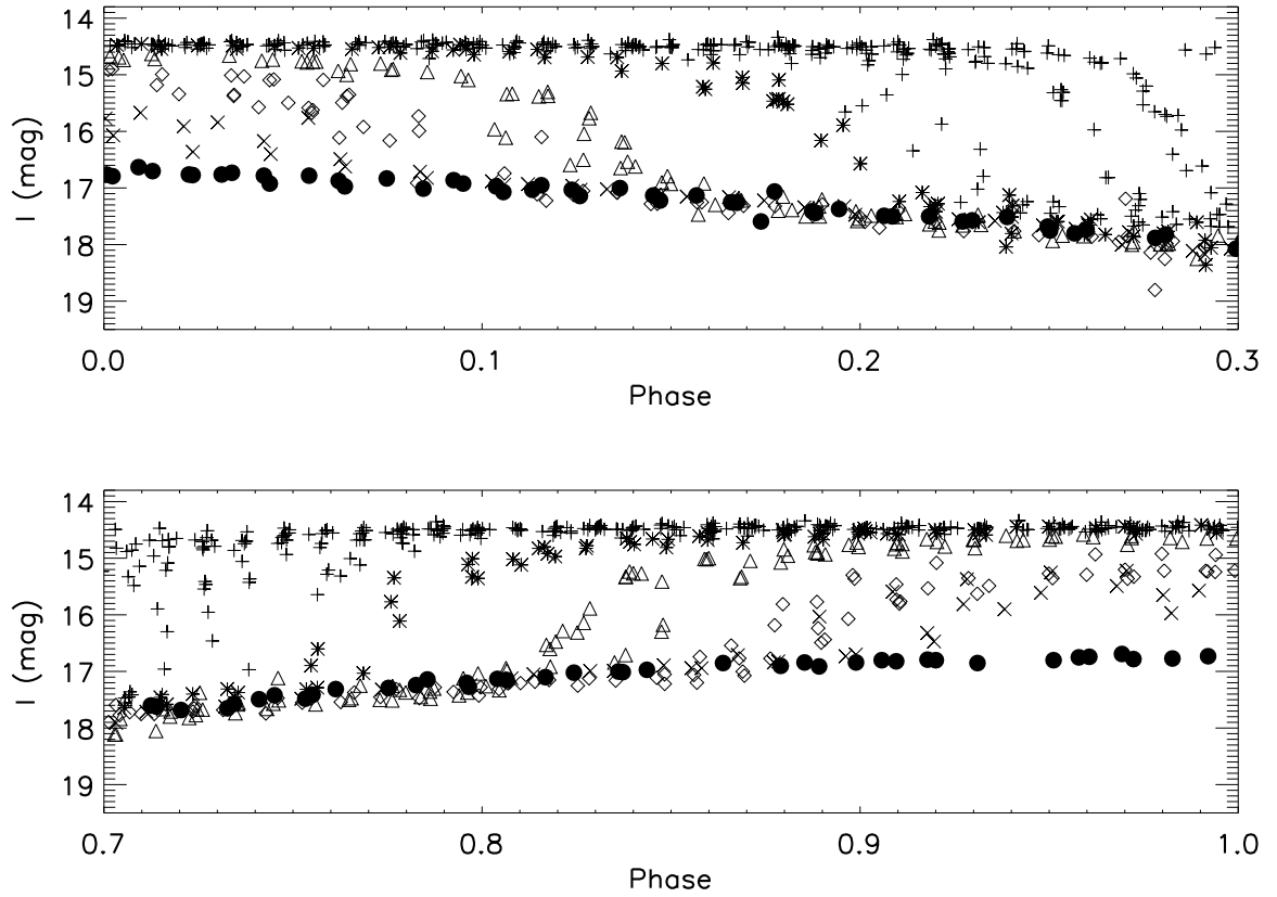
Fig. 5.— Same as Fig. 4 but with expanded horizontal axis. It is clearly seen that the light curve in 2009-10 (solid circles), when Star A was fully eclipsed at all binary phases, forms a low luminosity boundary to the light curve at all epochs.
