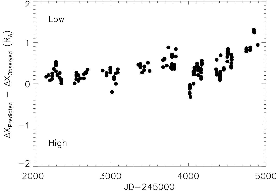
Fig. 10.— The difference between \Delta X predicted from Model 3 of Winn et al. (2006) and “observed” (based on the knife edge model corrected for scattered light) is plotted against Julian Date. A positive value of this quantity indicates that the system was brighter than Model 3 predicted at that time, meaning that the occulting edge was observed to be lower with respect to the star (i.e. the system was brighter) than the prediction. The unit on the y-axis is the radius of star A ( 1.3 R_{\odot} ). Only data for which the value of \Delta X inferred from the photometry lay within the range -0.3 < \Delta X < 0.6 are plotted, because these are the most reliable points, corresponding to the times when the system brightness is changing most rapidly.
