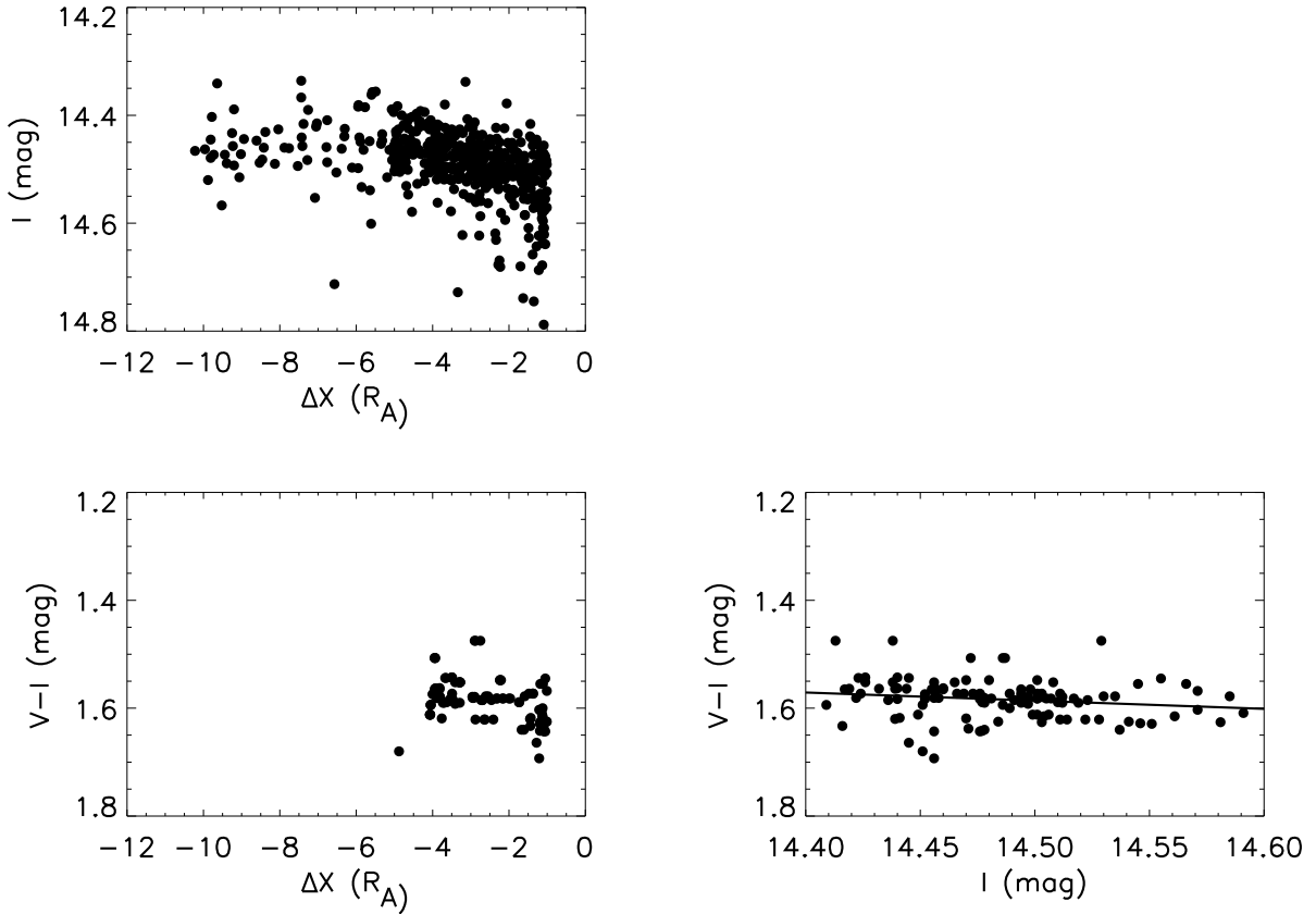
Fig. 6.— The top panel shows that when Star A is more than 5 stellar radii above the disk edge it shows no dependence of brightness on \Delta X . However, for -4.7 \leq \Delta X \leq -1 there is a clear dependence of brightness on height above the disk, characterized by a slope of 0.020 \pm 0.003 mag per stellar radius. The lower left panel shows that there is no detectable reddening of the system associated with the observed decline in brightness for -4.7 \leq \Delta X \leq -1 . The lower right panel shows that when the star is in its non-eclipsed state ( \Delta X < -1.5 , there is a small but significant correlation between its brightness and color, as reported previously by Hamilton et al. (2005). This is due to the fact that the brightness variations out of eclipse are caused by the rotation of a spotted star.
