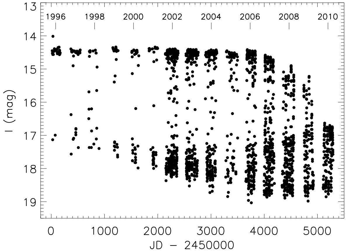
Fig. 2.— The light curve of KH 15D in the Cousins I band based on CCD photometry obtained at VVO, CTIO and MMO from 1995 to 2010. It is quite apparent that the system no longer reaches its previous brightness levels. Note that the one measurement in 1995 showing the system at about magnitude 14 is real. It represents our only fully unobscured CCD detection of Star B.
