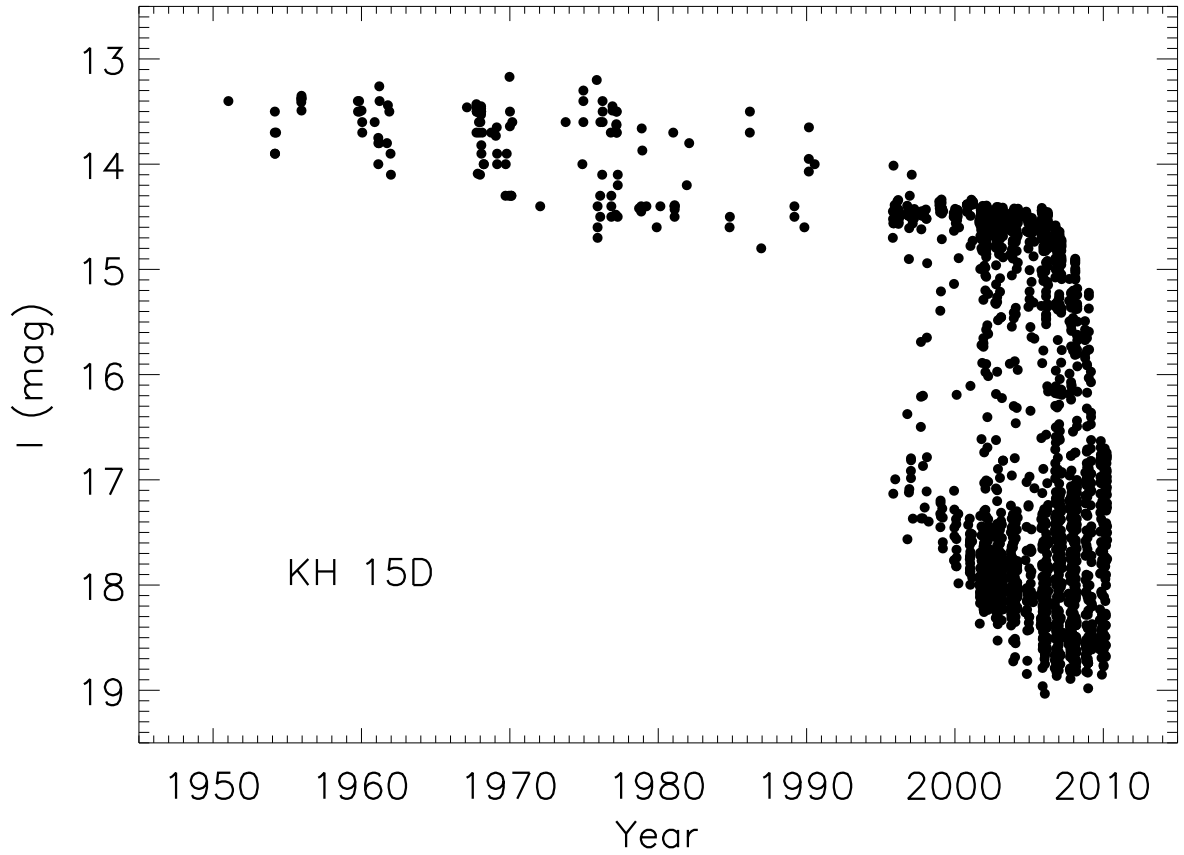
Fig. 1.— The light curve of KH 15D in the Cousins I band. Included here are all of the I or effective I measurements from the photographic photometry of Johnson & Winn (2004) and Johnson et al. (2005) that span the period 1950 to early 1996 as well as the CCD photometry from Hamilton et al. (2005) and this paper, which cover the period from late 1995 to early 2010 and are expanded in Fig. 2.
