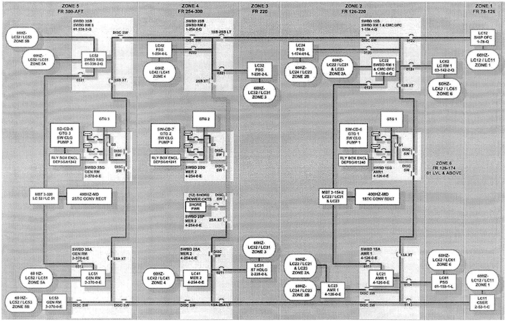
Figure 7: DDG 79-90 ACZEDS Layout [5]
