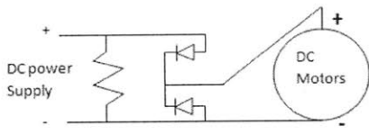
Figure 35: Basic Circuit Diagram
