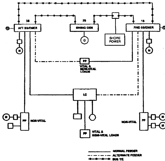
Figure 4: Radial Distribution System with Dual Purpose Generators [4]
