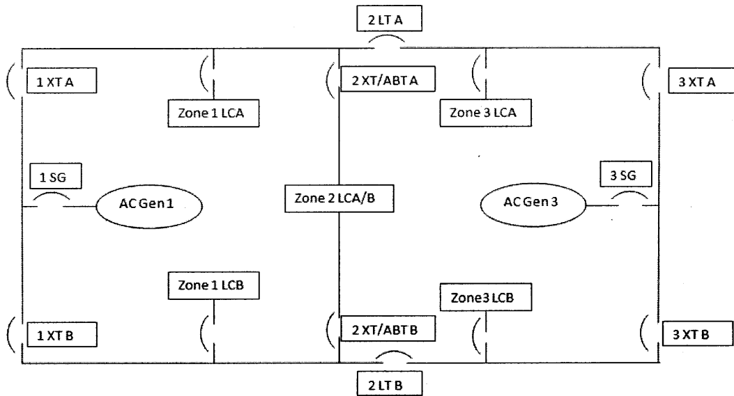
Figure 20: AC ZEDS Hardware Model Concept
