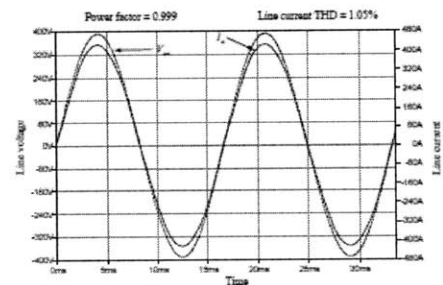
Figure 54: Wave Form of an Active Rectifier
