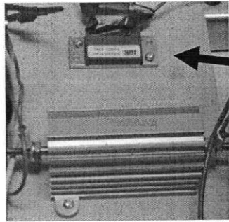
Figure 36: HEXFRED™ Diode
