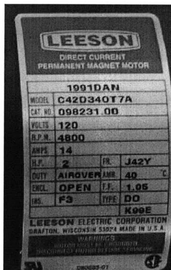
Figure 17: DC Motor Name Plate
