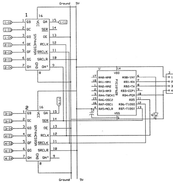
Figure 43: AC ZEDS Circuit Diagram (1 of 2)
