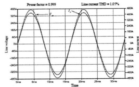
Figure 53: Wave Form of Passive Rectifier with Filtering
