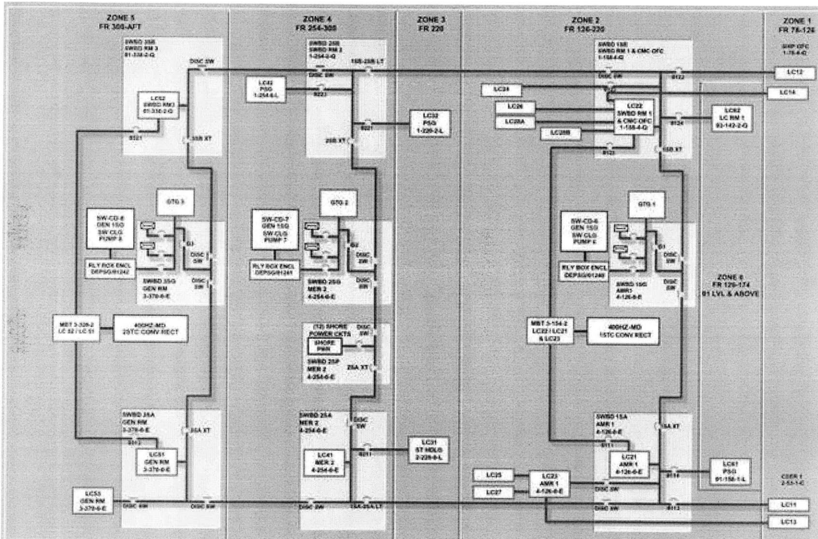
Figure 8: DDG 91+ AC ZEDS Layout [6]
