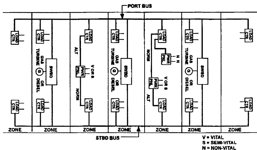
Figure 6: AC ZEDS for a Surface Combatant Ship [4]
