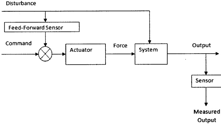
Figure 59: Feed-Forward Controller
