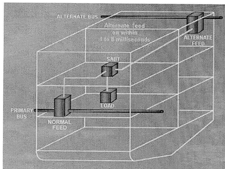
Figure 9: Example SABT Configuration [6]
