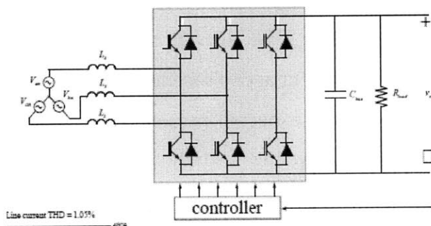
Figure 51: Active Rectification Circuit
