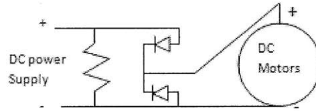
Figure 38: DC Motor Electrical Connection Diagram
