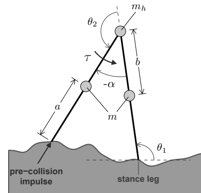
Fig. 27. Four states of the CG walker during continuous dynamics. The biped model is depicted here immediately after an impact. A pre-collision impulse occurs at each step, and only the torque source at the hip actuates the walker until the next step occurs.
