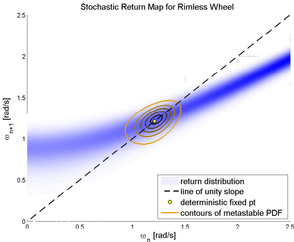
Fig. 4. Return distribution and metastable “neighborhood” for an 8-spoke rimless wheel on downhill terrain with a mean step-to-step slope of 8^\circ and \sigma = 1.5^\circ . There is now a probability density function describing the transition from \omega_n to \omega_{n+1} .
