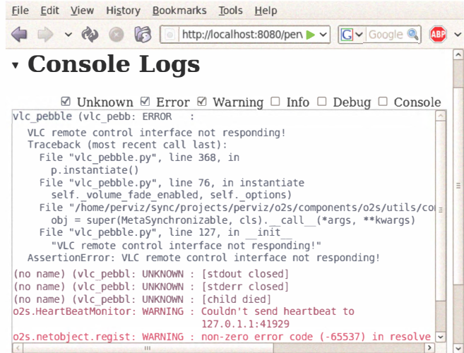
Figure 4. Filtering controls help remove low-level debugging so that errors become more apparent. Here, the aggregated debugging console distinctly shows an error traceback within a remote application component. Debugging messages are color-coded to their respective sources.
