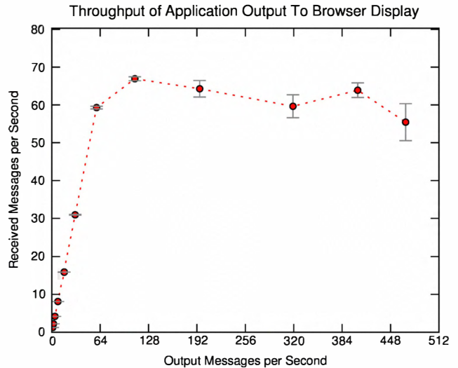
Figure 6. Sustained throughput tapers at 60 messages/second, or a message roughly every 16ms. Each point represents the average of 10 runs.
