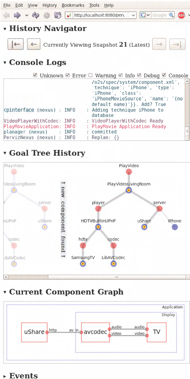
Figure 1. PerViz provides a web-based interface to inspect running systems in real-time. Here, the system just found a new potential component for use.
