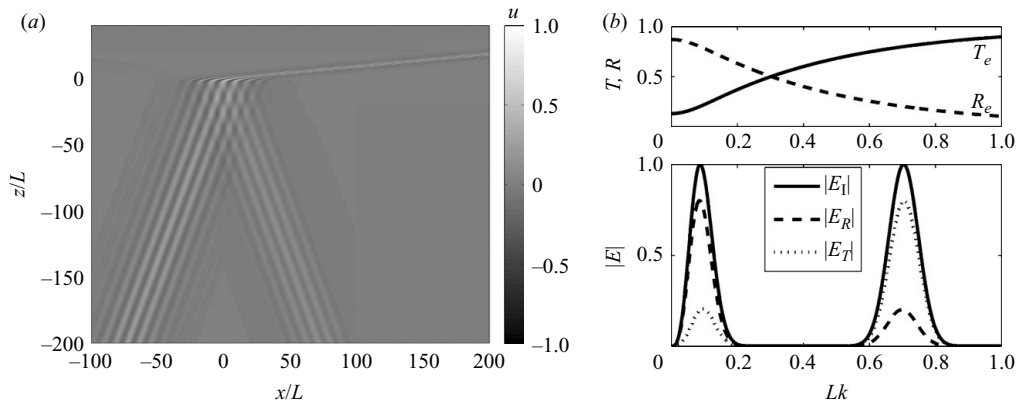
FIGURE 5. Filtering of an internal wave beam by a finite-width transition region. (a) The horizontal velocity field u at an arbitrarily chosen phase. The maximum value is scaled to unity, and the spatial dimensions are scaled by the interface length-scale L . (b) The plane wave reflection and transmission coefficients as a function of Lk . (c) The energy spectrum |E(k)|=k|\Psi|^2\cot\theta for the incident ( I ), transmitted ( T ) and reflected ( R ) wave beams. The values of \omega/N_1 and N_2/N_1 are 0.94 and 10, respectively.
