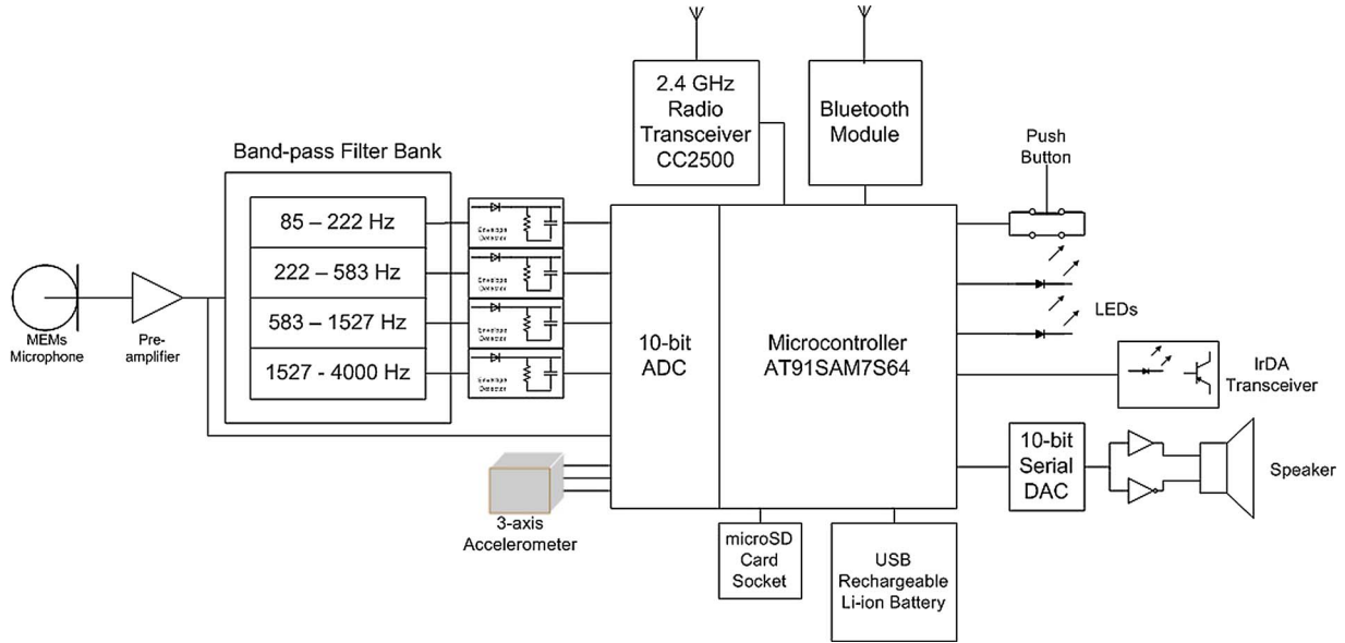
Fig. 2. Wearable sociometric badge's block diagram.
