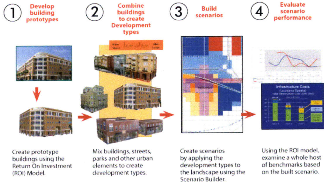
Figure 5-2: Approaches That Calculate Neighborhood/District Energy Consumption based on the Aggregation of Individual Building Prototypes 4
