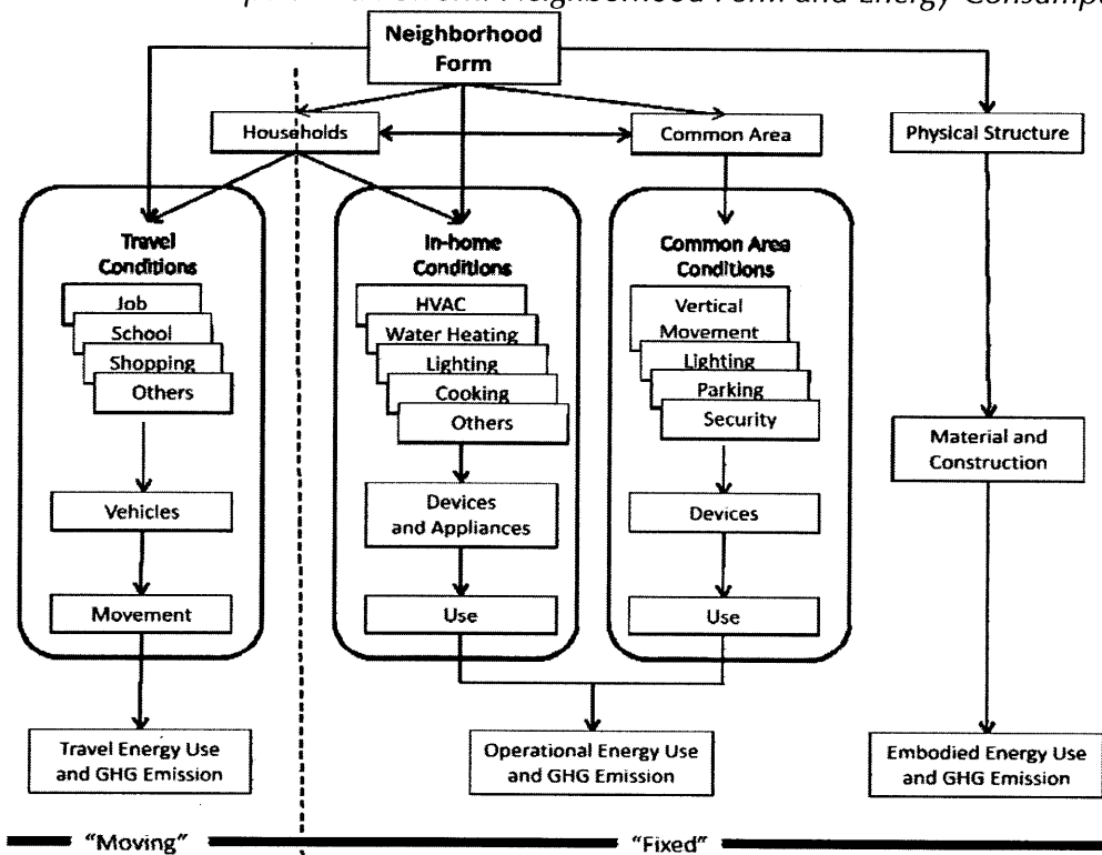
Figure 2-1: The Conceptual Framework: Neighborhood Form and Energy Consumption 2
