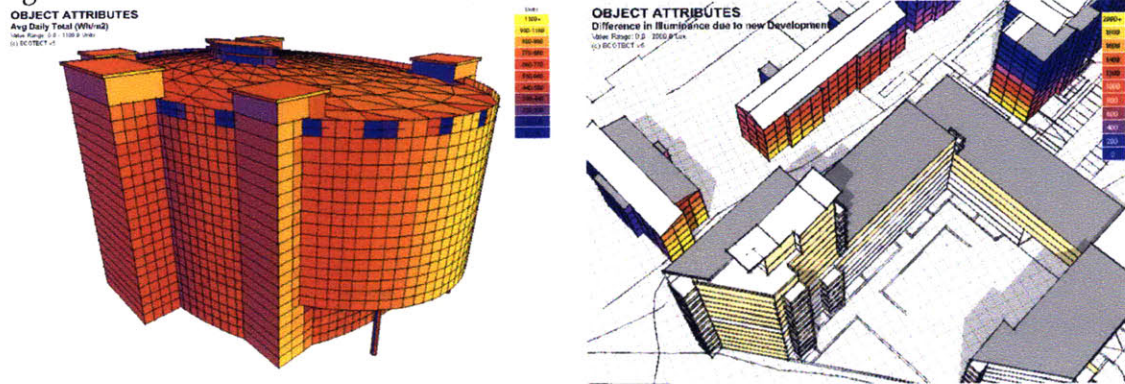
Figure 4-1: Cumulative Solar Radiation over the External Surfaces by Ecotect 1
