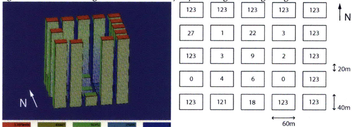
Figure 4-2: Maximizing Solar Radiation by Optimizing Building Height 3
