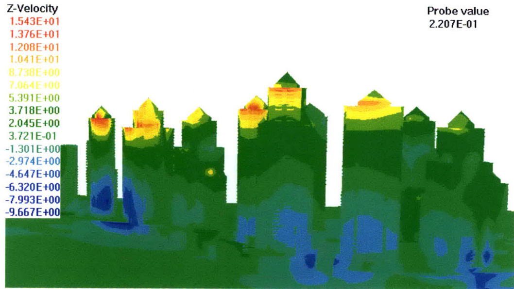
Figure 4-5: Wind Speed on Buildings, Simulated by FLAIR, Phoenix 8
