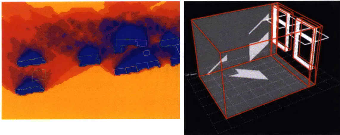
Figure 3-1: ECOTECT Solar Tool for Site Analysis and Internal Sun Penetration
