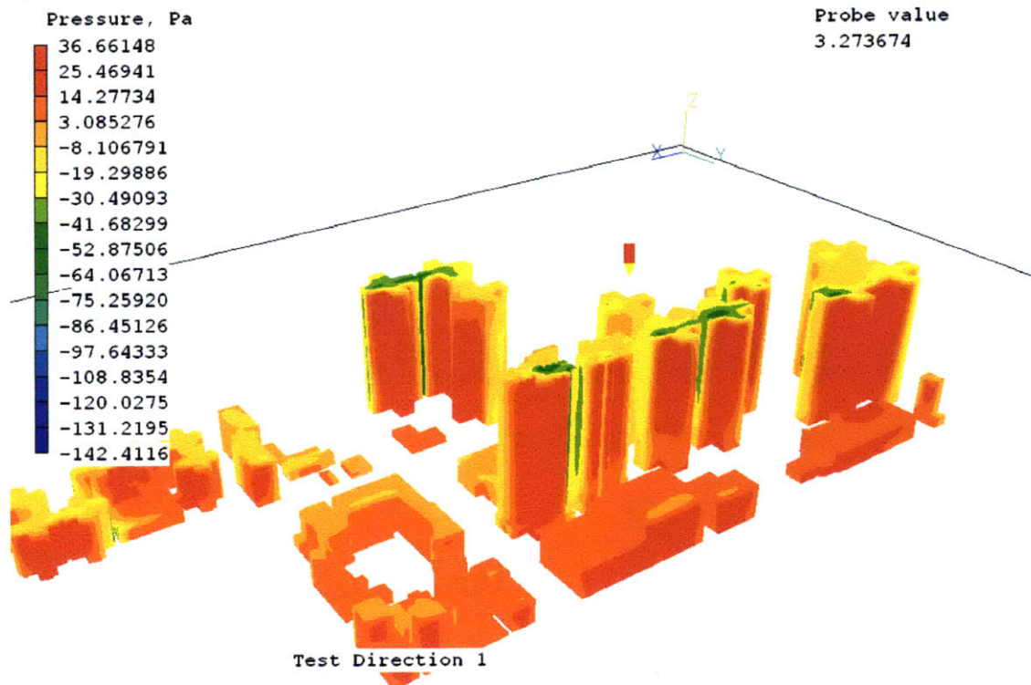
Figure 4-4: Wind Pressure on Buildings, Simulated by FLAIR, Phoenics 7
