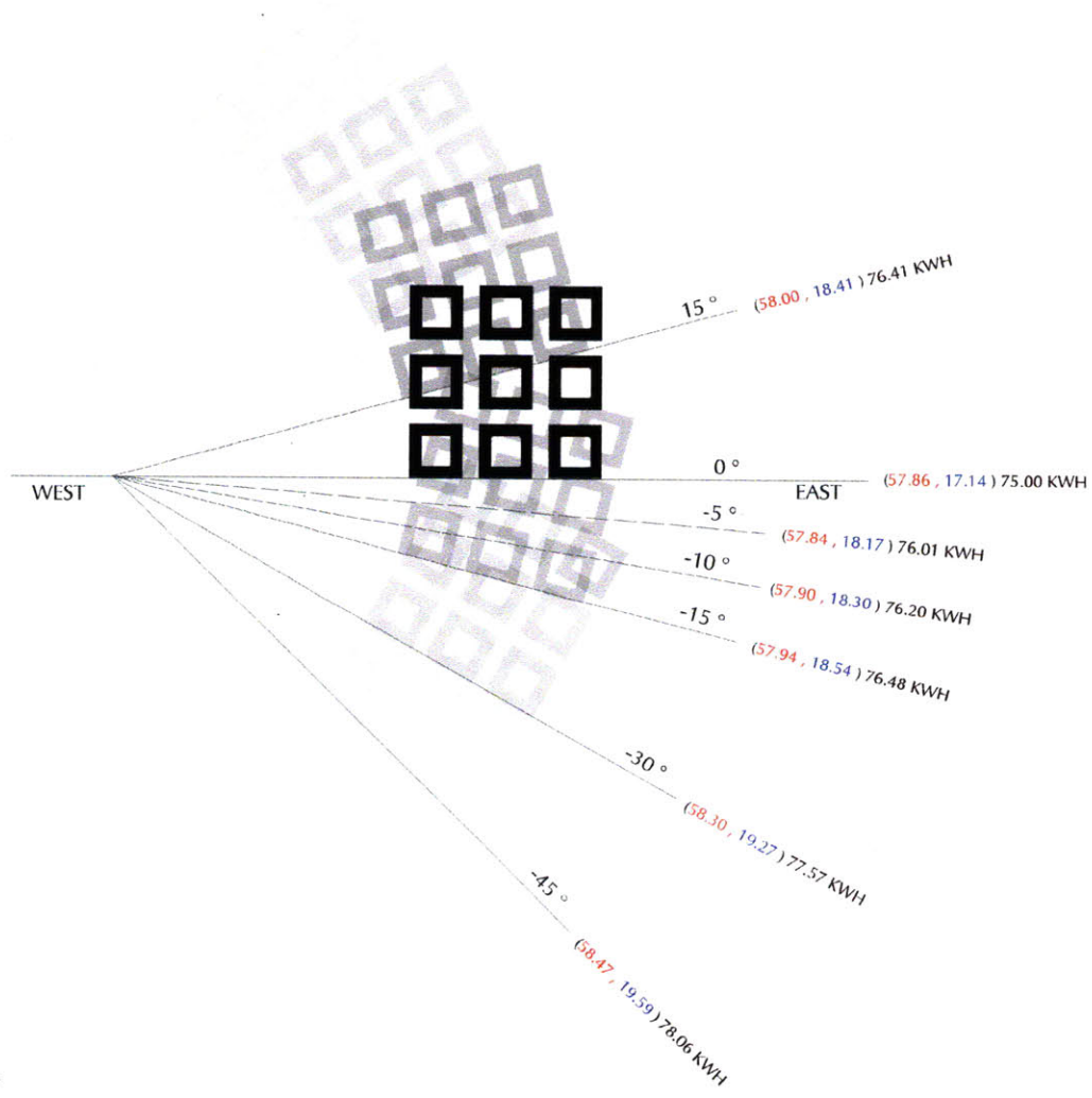
Figure 6-4: Yearly Energy Consumption with Variation in Cluster Orientation*
