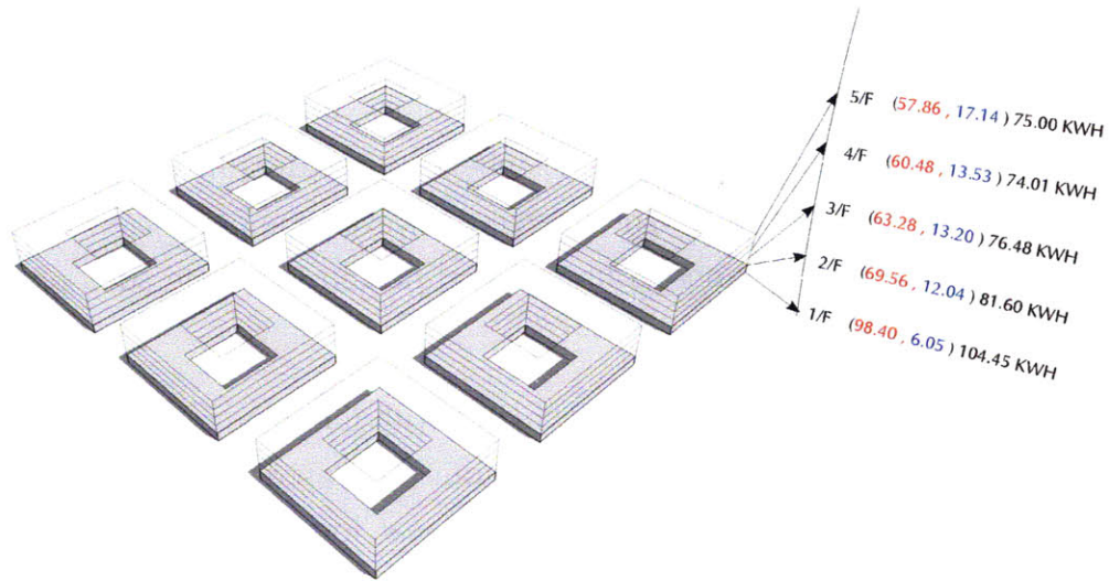
Figure 6-2: Yearly Energy Consumption with Variation in Height*
