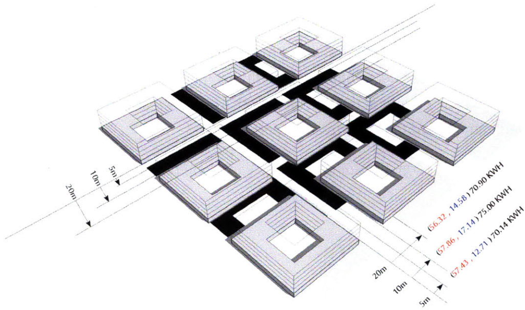
Figure 6-3: Yearly Energy Consumption with Variation in Distance *
