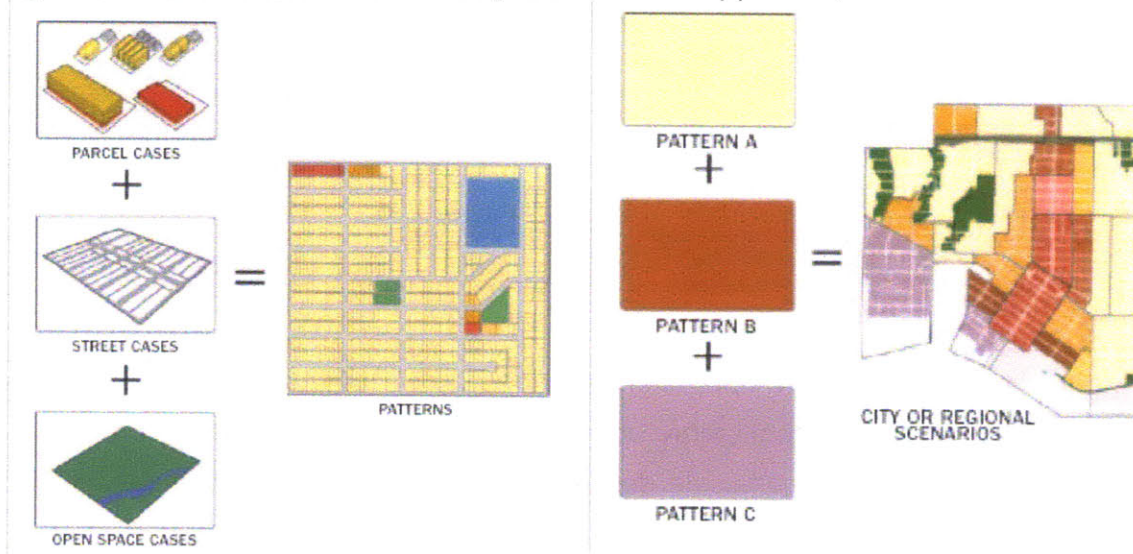
Figure 5-3: Patterns in DPA (Development Pattern Approach) 6
