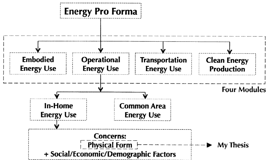
Figure 2-4: Relationship between the Thesis and the Energy Pro Forma
