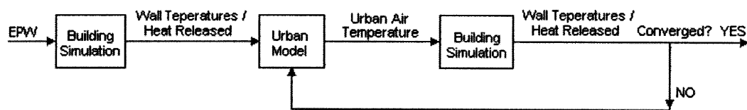
Figure 5-6: The Coupling Process of UWG
