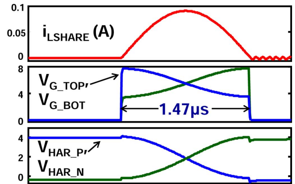
Fig. 14. Simulation plots of the voltage at the output nodes of the harvester and the gate-drive of the bias-flip switches.
