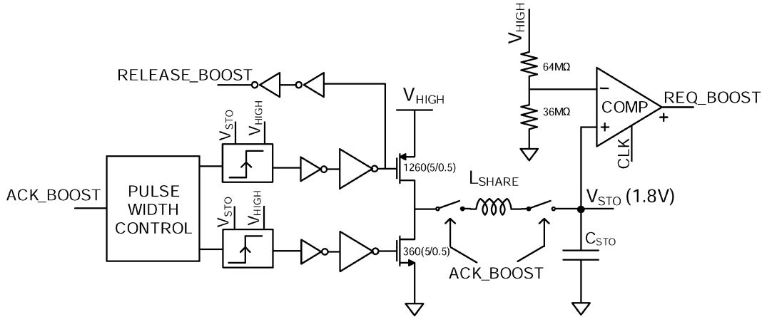
Fig. 16. Architecture of the boost DC-DC converter used to generate V_{HIGH} .
