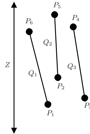
Fig. 8. Shown above are three line segments, Q_1 , Q_2 , and Q_3 , and a line Z which does not intersect the convex hull of P . We want to find m(\bigcap_{i=1}^{|Q|} [Q_i]) which is equivalent to m([Z] \cap [Q_1] \cap [Q_2] \cap [Q_3]) .
