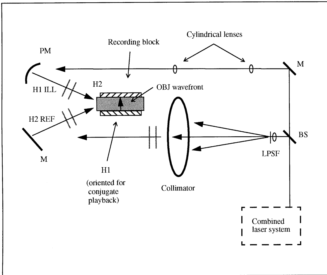
Figure 5.17: Optical setup used for recording a transmission-mode edgelit (H2) hologram using an edgelit reflection H1 coupled to the same recording block. (LPSF--lens-pinhole spatial filter; M--mirror; BS--beam splitter)
