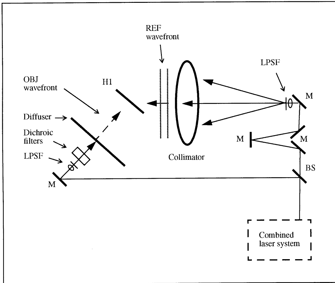
Figure 5.10: Optical setup used to record conventional reflection H1 with two-color gamut. (LPSF--lens-pinhole spatial filter; M--mirror; BS--beam splitter)
