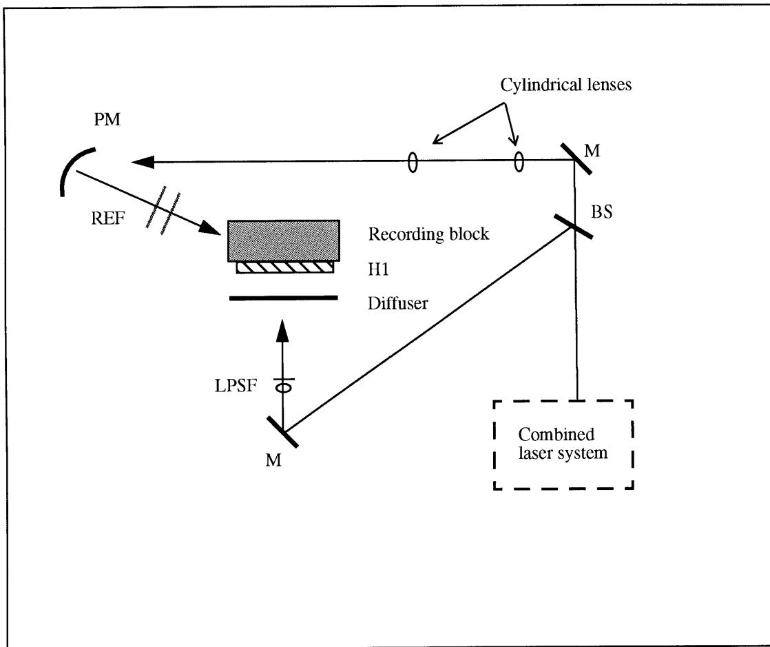
Figure 5.14: Optical recording setup for reflection-mode edgelit master (H1) hologram. (LPSF--lens-pinhole spatial filter; M--mirror; BS--beam splitter)
