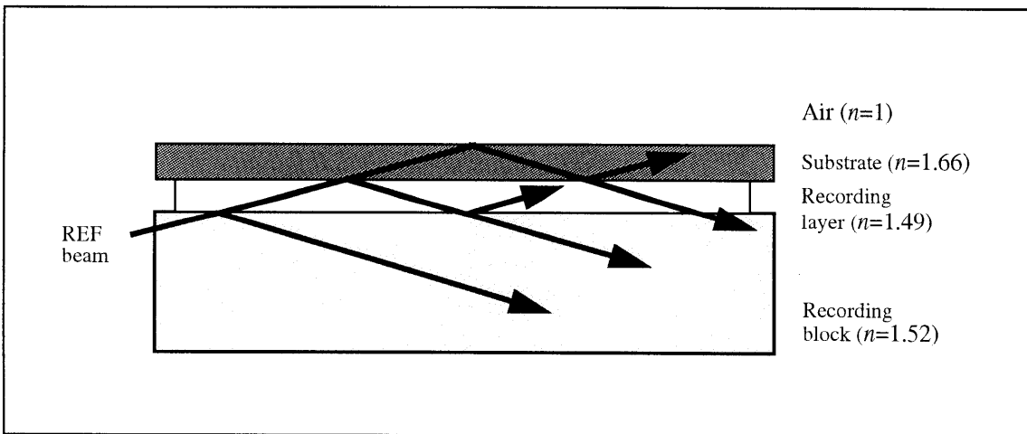
Figure 3.3: Schematic of the Fresnel reflections caused by reference beam propagating through photopolymer material coupled to a recording block. Note: refraction is omitted for clarity.
