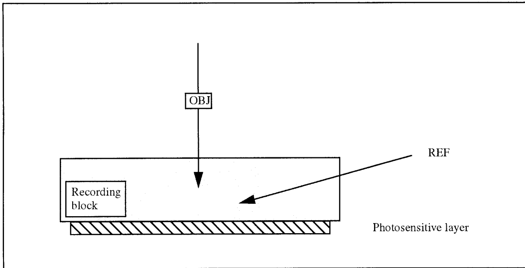
Figure 4.5: Schematic of a typical coupled transmission-mode edgelit recording stack. The photosensitive layer is coupled to the recording block on the side farthest from the object light. The reference and object beams illuminate the photosensitive layer from the same side. (OBJ--object light, REF--reference light)
