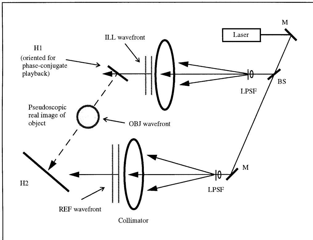
Figure 5.5: Optical setup used for recording the intermediate full-aperture transfer (H2). (LPSF--lens-pinhole spatial filter; M--mirror; BS--beam splitter)
