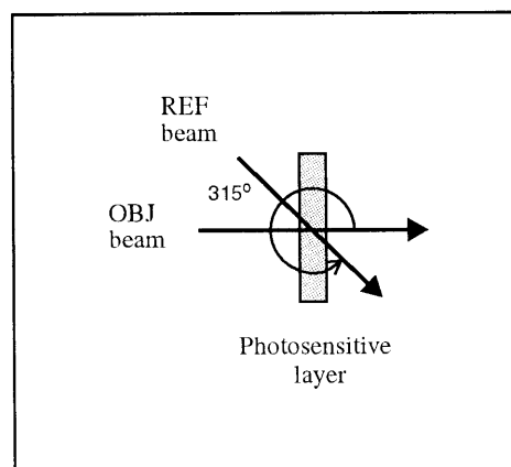
Figure 2.7: Typical transmission hologram recording geometry. Reference and object beams illuminate the photosensitive layer from the same side. (The hologram substrate is not shown, and angles are specified as measured in air.)
