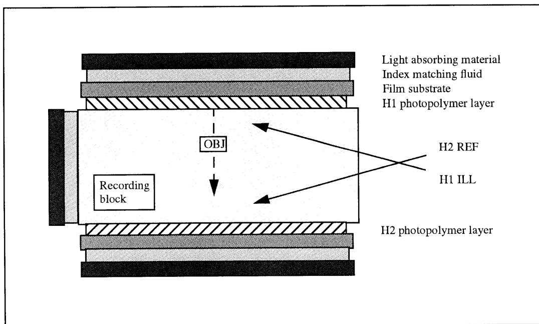
Figure 5.16: Detail of typical recording stack used to record a transmission-mode edgelit transfer hologram using a reflection-mode edgelit H1 coupled to the same recording block.
