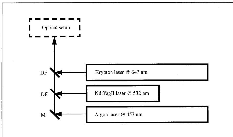
Figure 5.1: Laser beam combining setup for multi-wavelength color holography. (DF--dichroic filter, and M--high energy mirror.)
