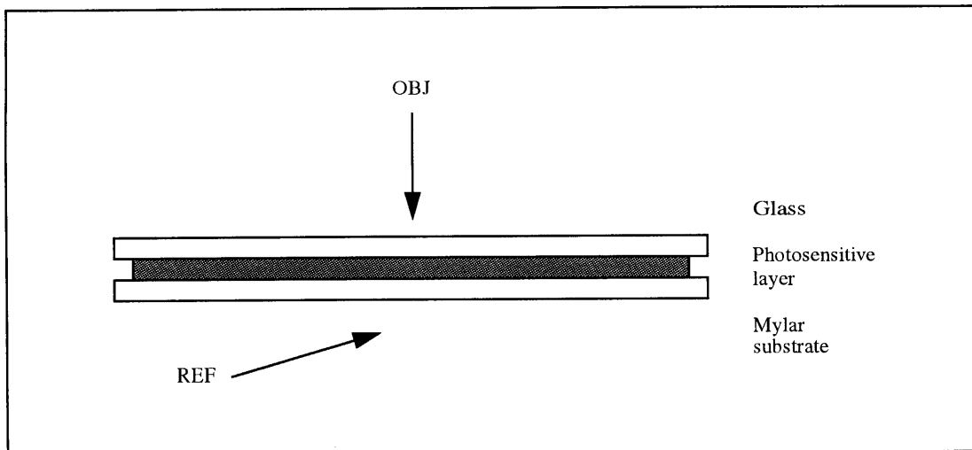
Figure 5.12: Schematic of the coupled recording stack used to record a conventional color reflection H1 in photopolymer.
