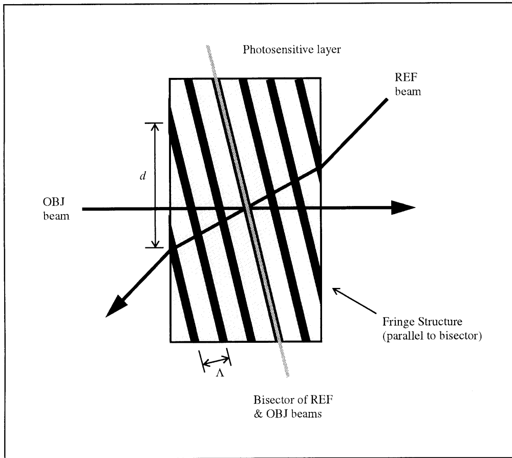
Figure 2.11: Interference fringe structure of a conventional reflection hologram. Fringes are oriented more or less parallel to the plane of the photosensitive layer.
