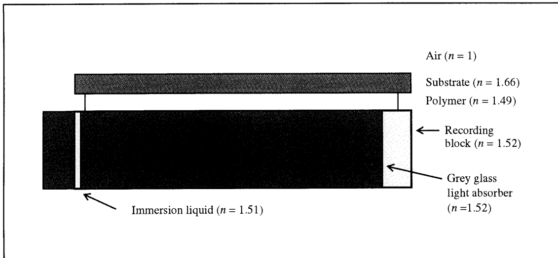
Figure 5.3: Coupled recording stack for a photopolymer edgelit hologram. Note that the grey glass absorbing material is coupled to three edges of the recording block.
