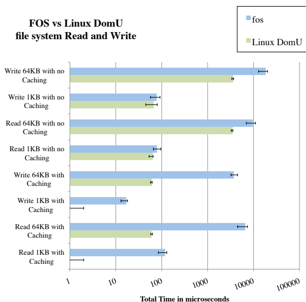
Figure 5: Overall latency experienced by the fos and Linux DomU ext2 file systems in reading and writing files of varying sizes from the file system.
