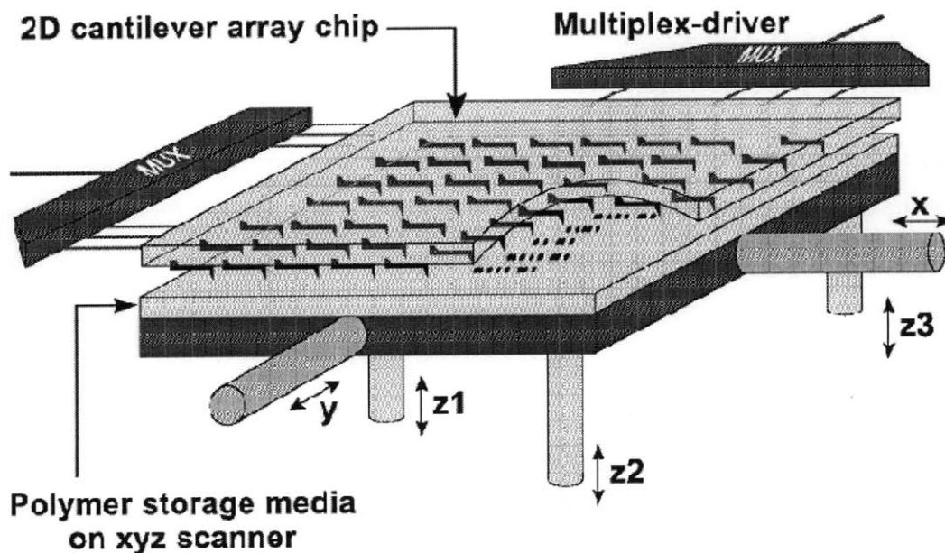
Figure 10. Schematic drawing showing Millipede concept [92]
