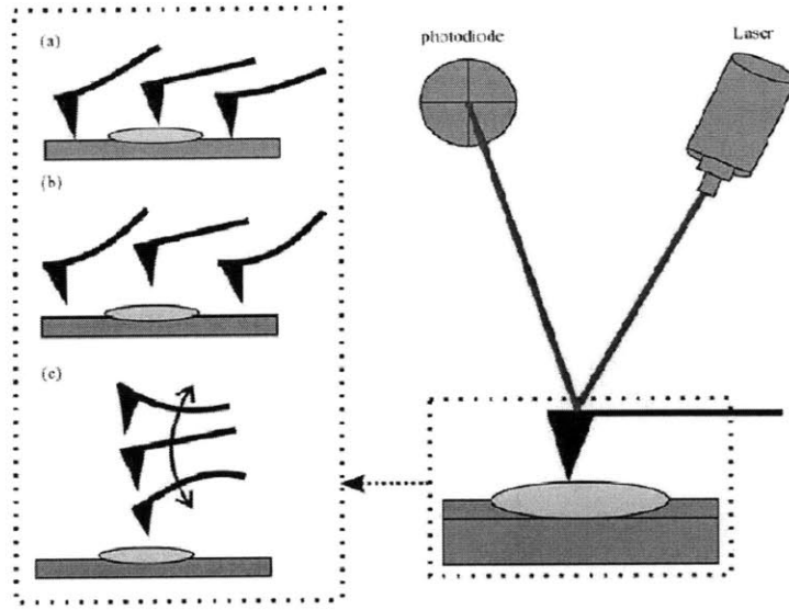
Figure 4. Principle of AFM operation [64]
