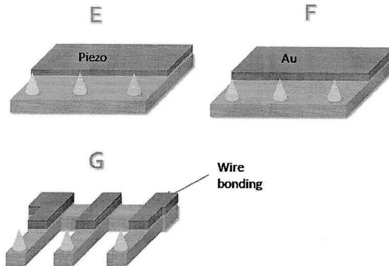
Figure 13. Cantilever array fabrication process
