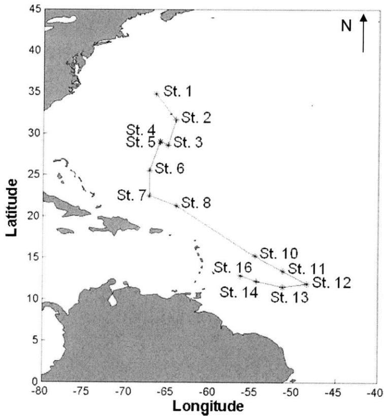
Figure 1: Leg one of cruise OC469, from Woods Hole, MA to Bridgetown, Barbados from October 2-22, 2010. Stations (*) are labeled 1-16.
