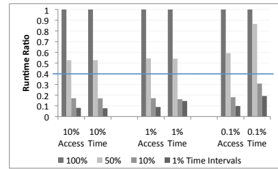
Fig. 12. Query performance with temporal predicates.
