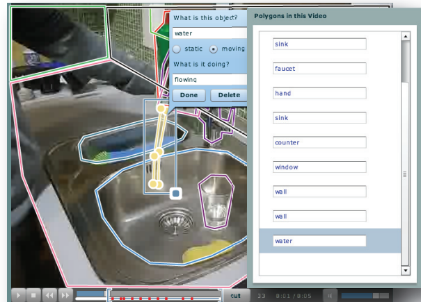
Figure 2. Object annotation. Users annotate moving or static objects in a video by outlining their shape with a polygon and describing their actions.
