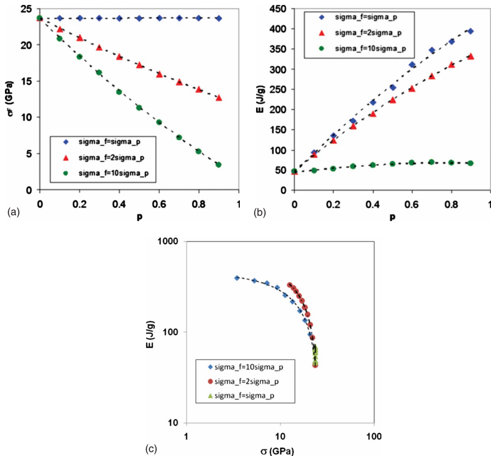
FIG. 6. (Color online) Numerically calculated dependence of (a) specimen strength \sigma_f and (b) energy-to-break (per unit mass) E on the parameter p ; (c) corresponding energy-to-break vs strength plot. Numerical points are fitted with second-order polynomials.
